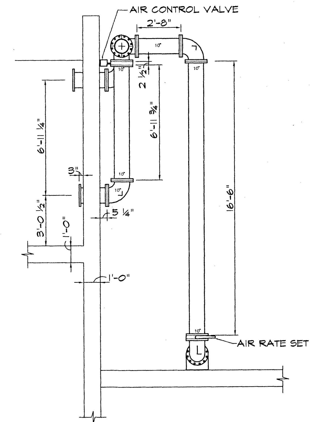
AIR PIPING SECTION NOT TO SCALE
