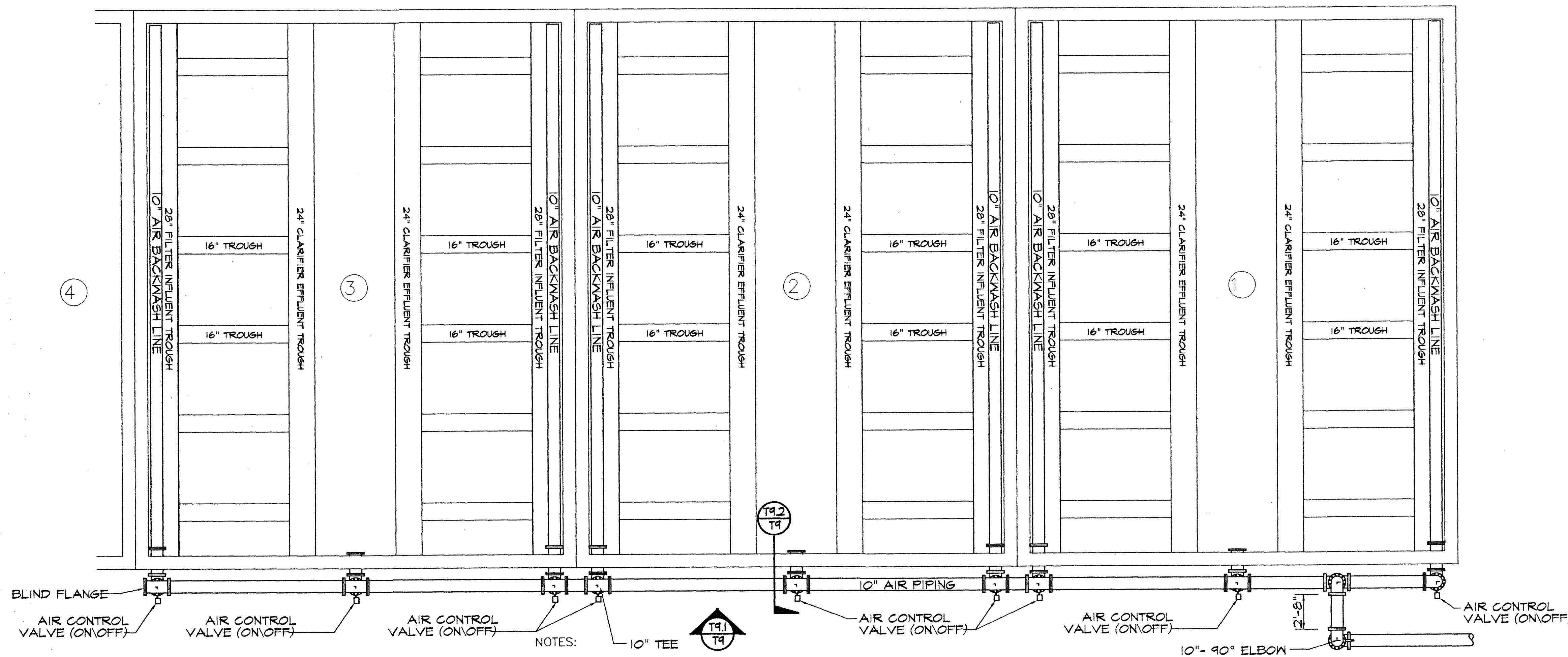
AIR PIPING PLAN SCALE 1" = 5'-0"
