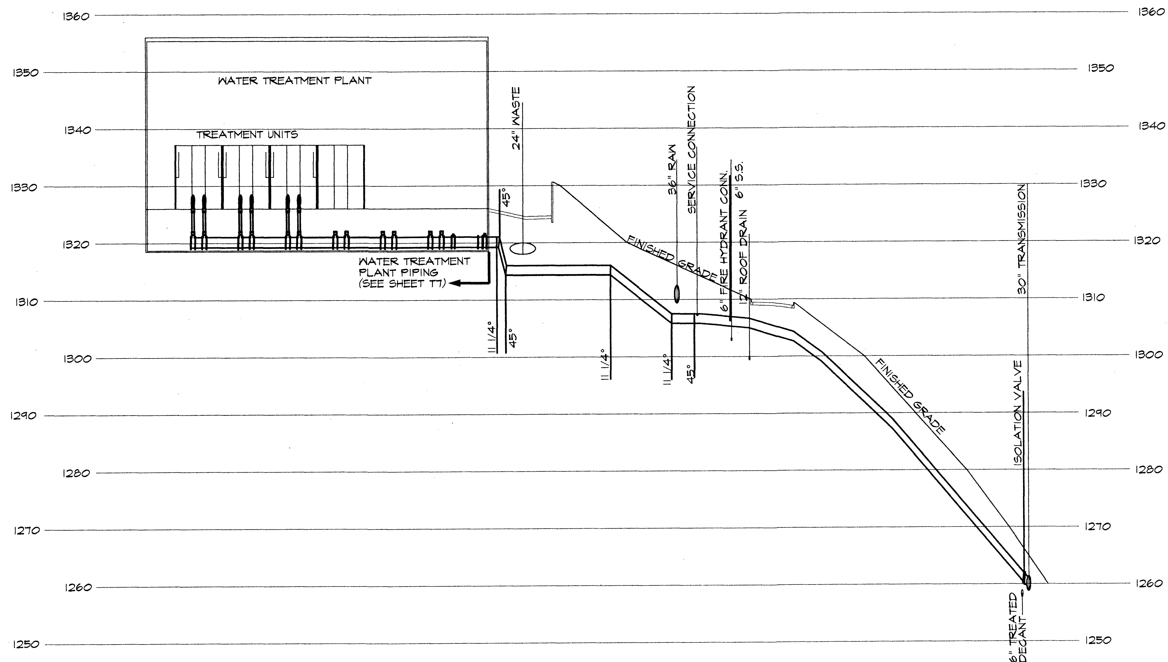
BACKWASH FEED LINE PROFILE SCALE VERT 1" = 10'-0" HORIZ 1" = 40'-0"
