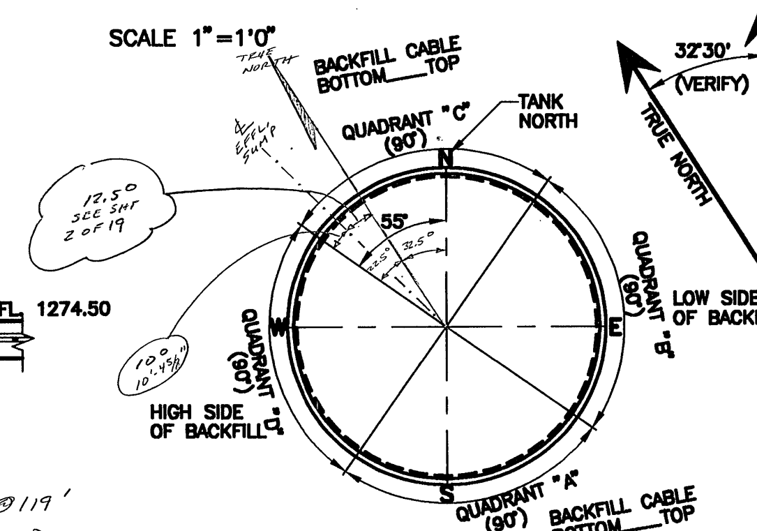
RESTRAINT CABLE LOCATION PLAN
