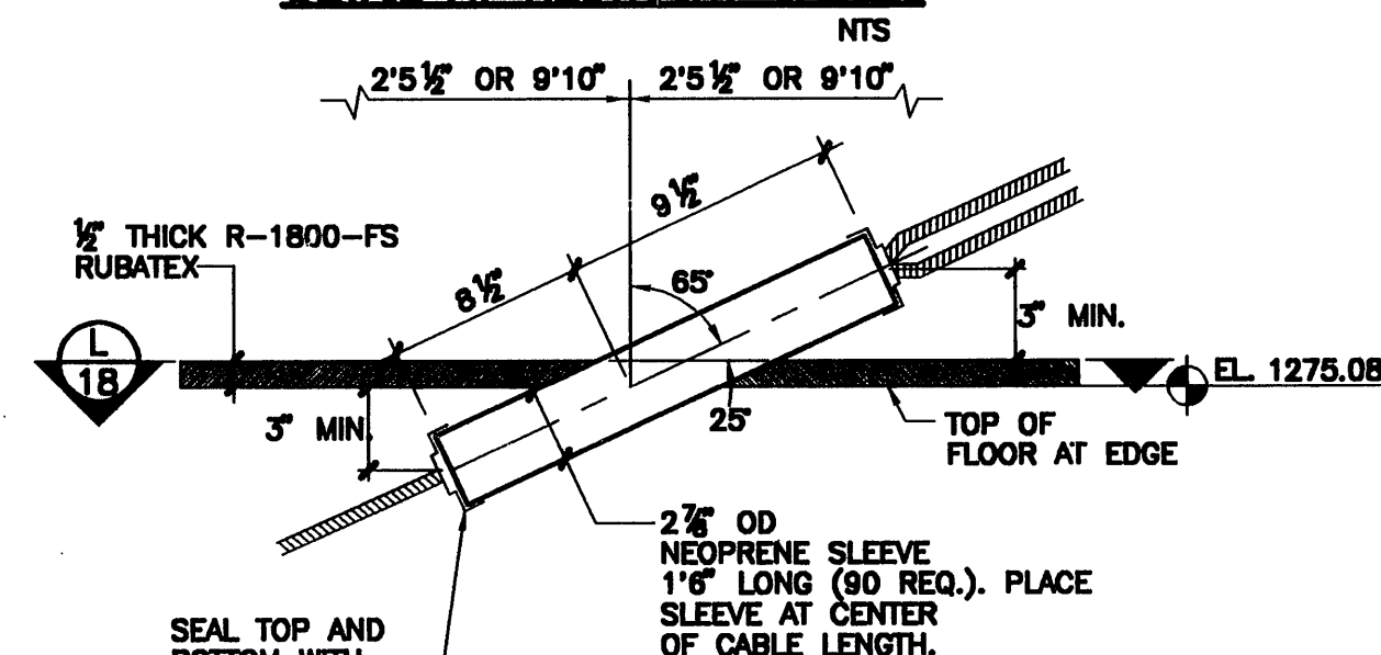
DETAIL AT RESTRAINT CABLES
