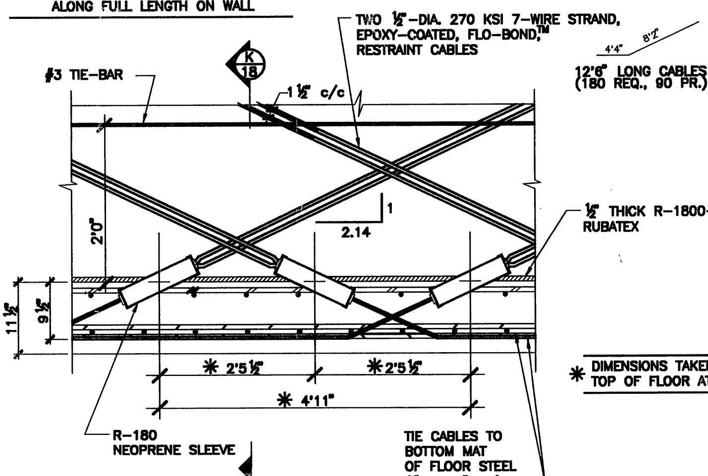
DETAIL AT RESTRAINT CABLES
