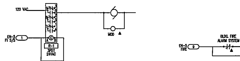
F-21 WIRING DIAGRAM
