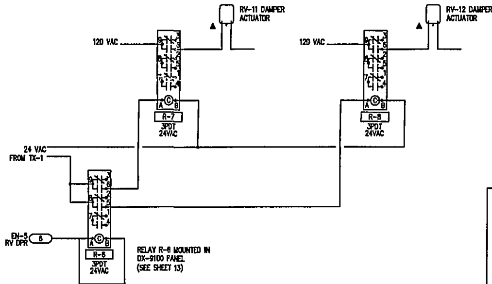
RV-11 & 12 DAMPER CONTROL
