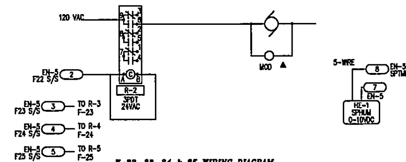
F-22, 23, 24 & 25 WIRING DIAGRAM
