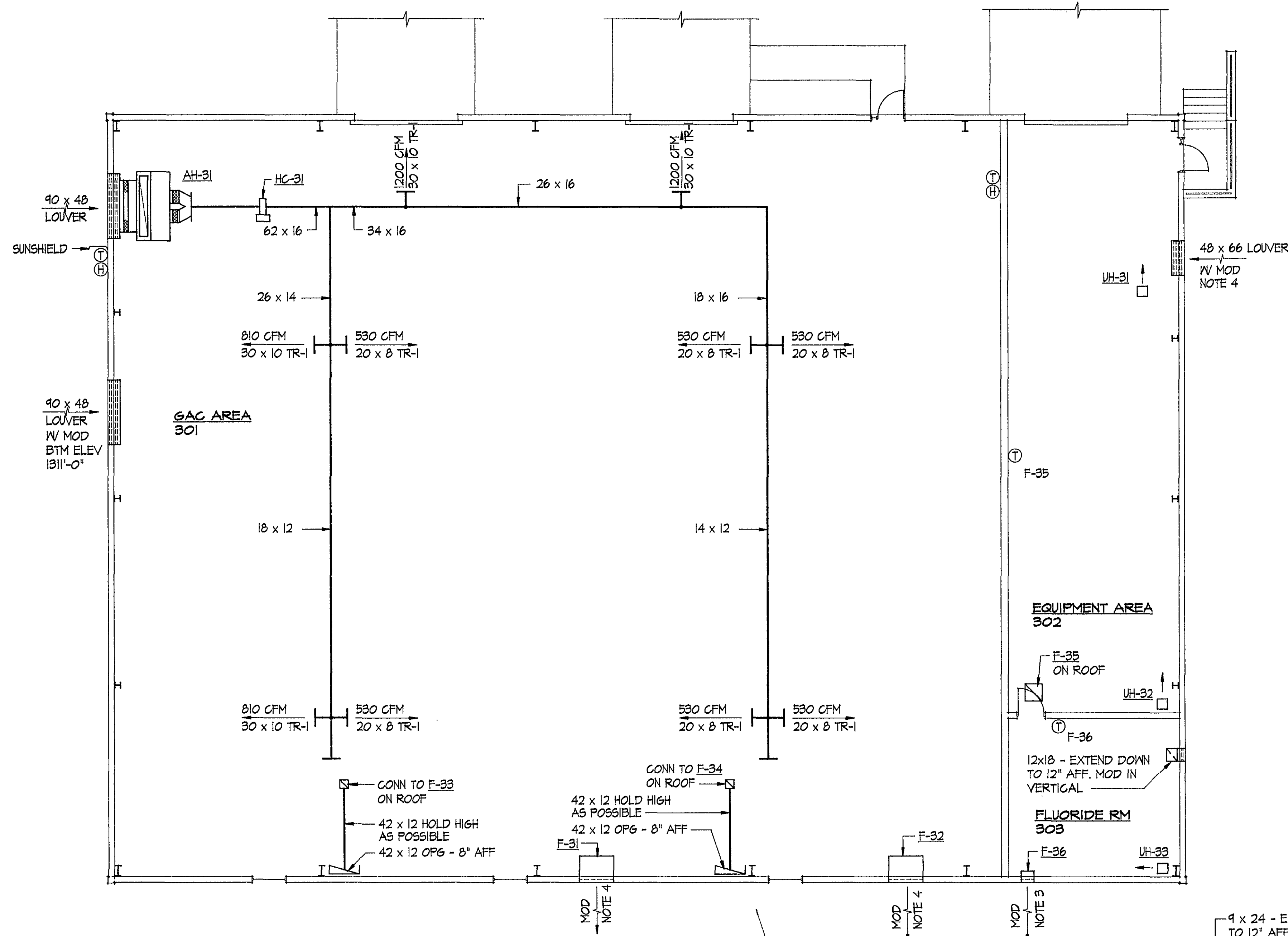
MECHANICAL DIAGRAM - GAC BUILDING SCALE 1/8" = 1'-0"
