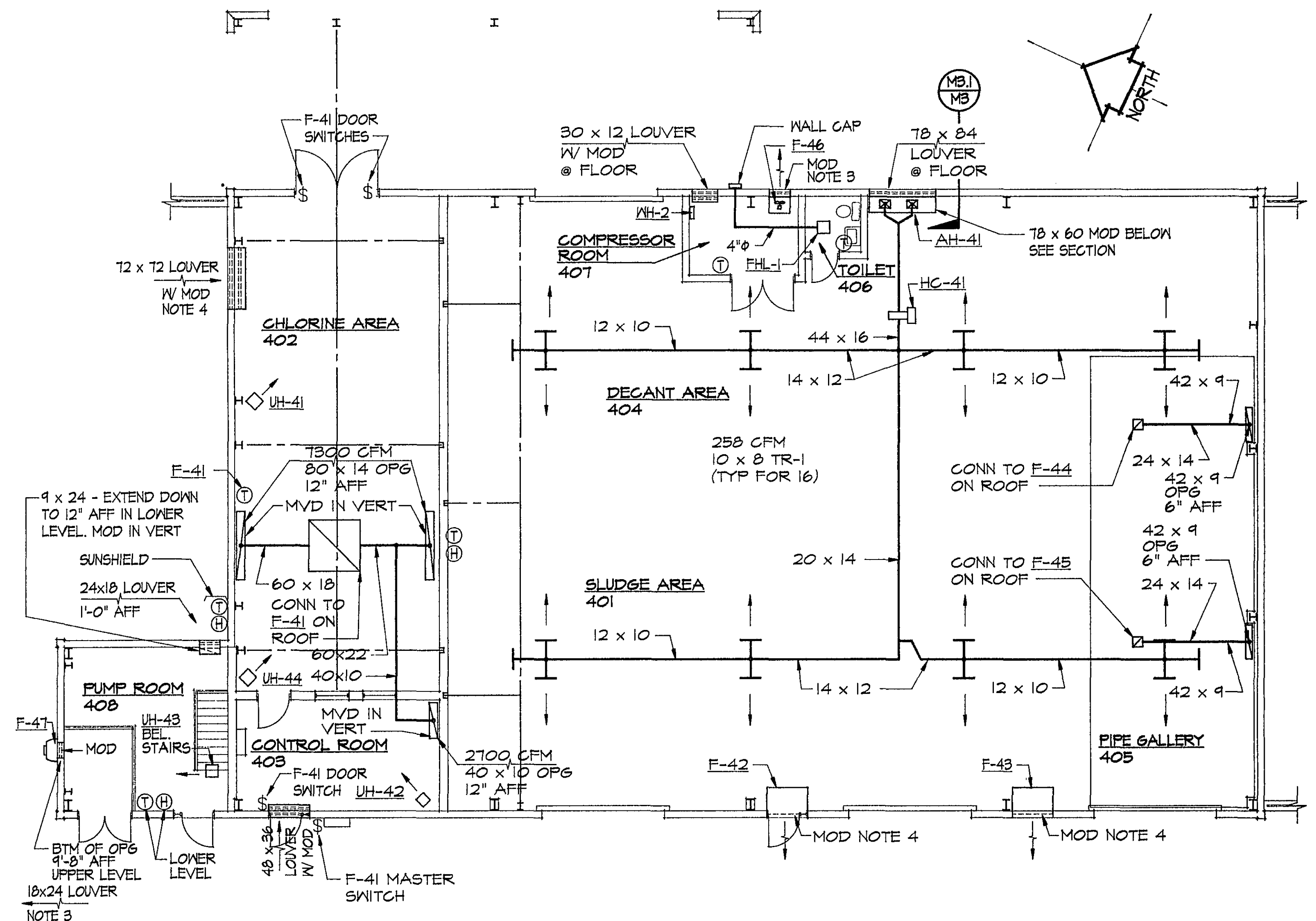
MECHANICAL DIAGRAM - POST TREATMENT BUILDING SCALE 1/8" = 1'-0"
