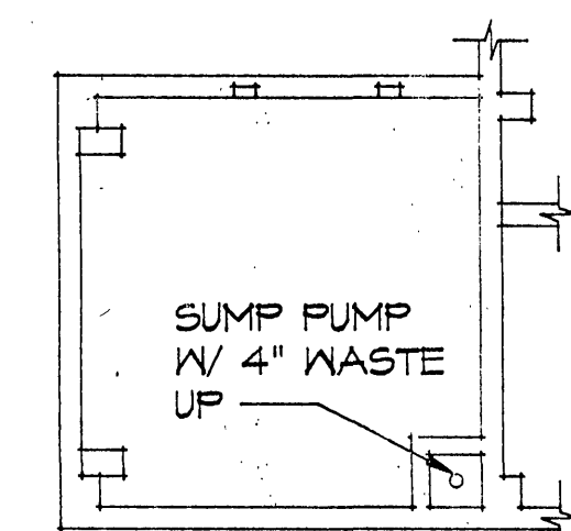
BASEMENT DIAGRAM - PUMP ROOM SCALE 1/8" = 1'-0"
