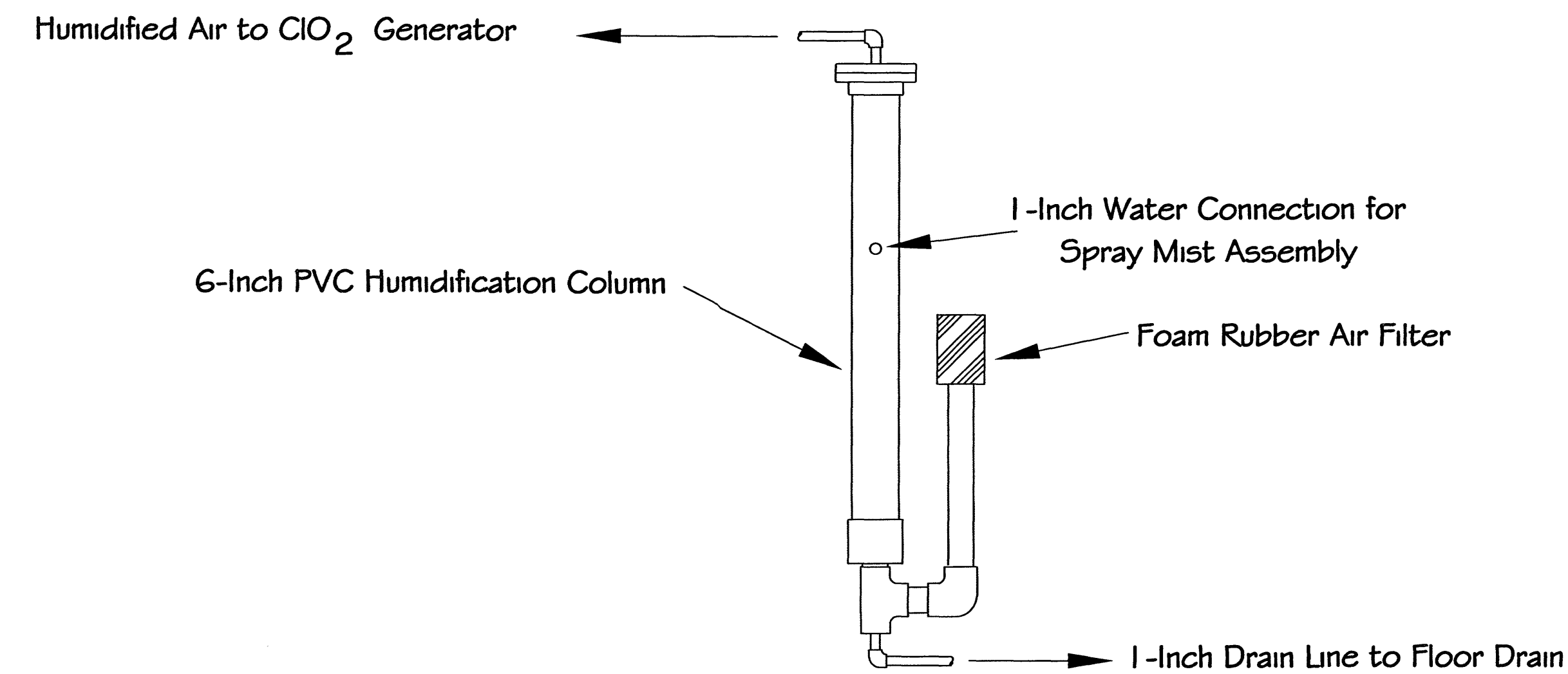
Air Humidification Column Detail SCALE: 3/4" = 1'
