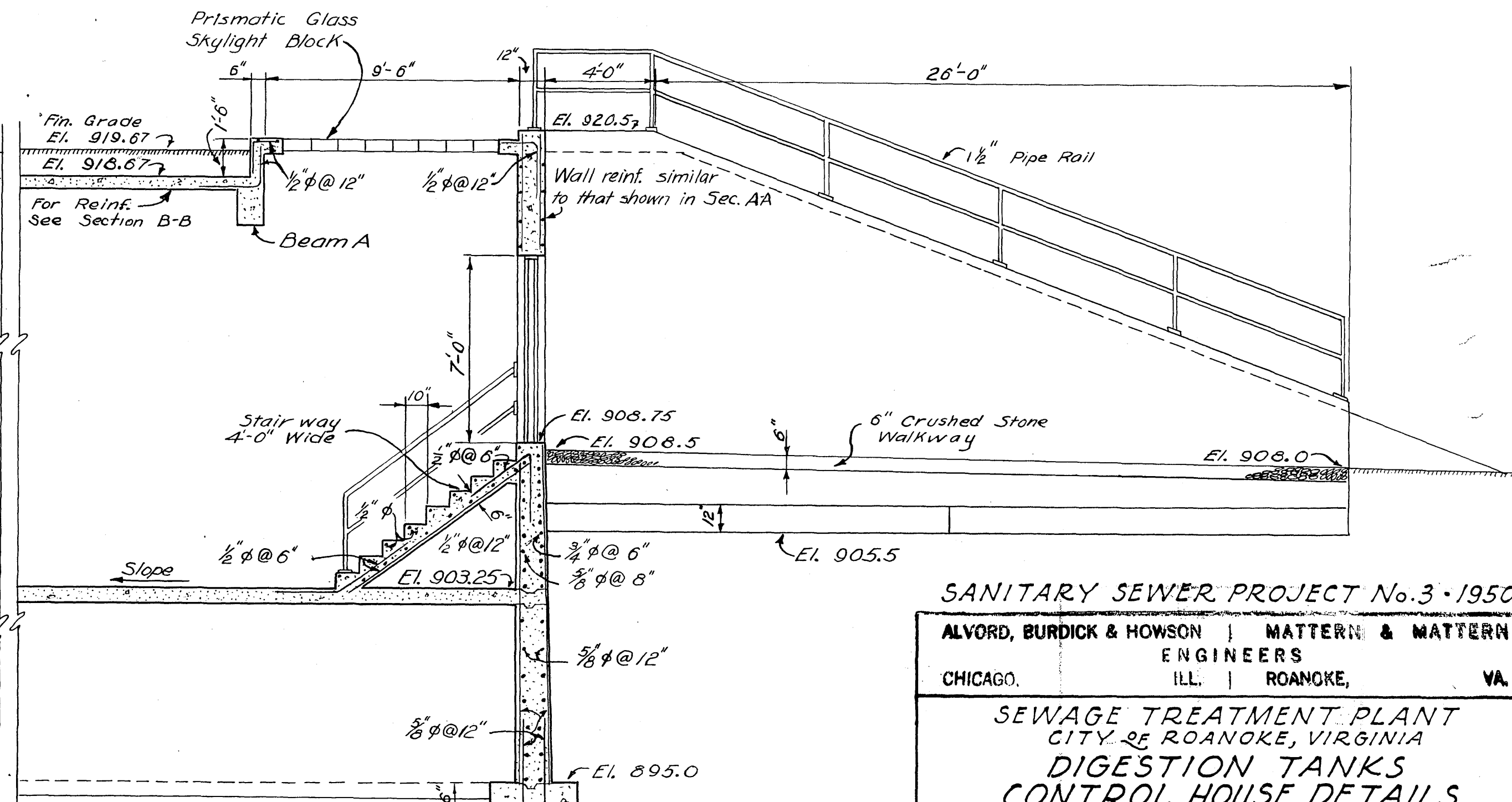
SECTION F-F
