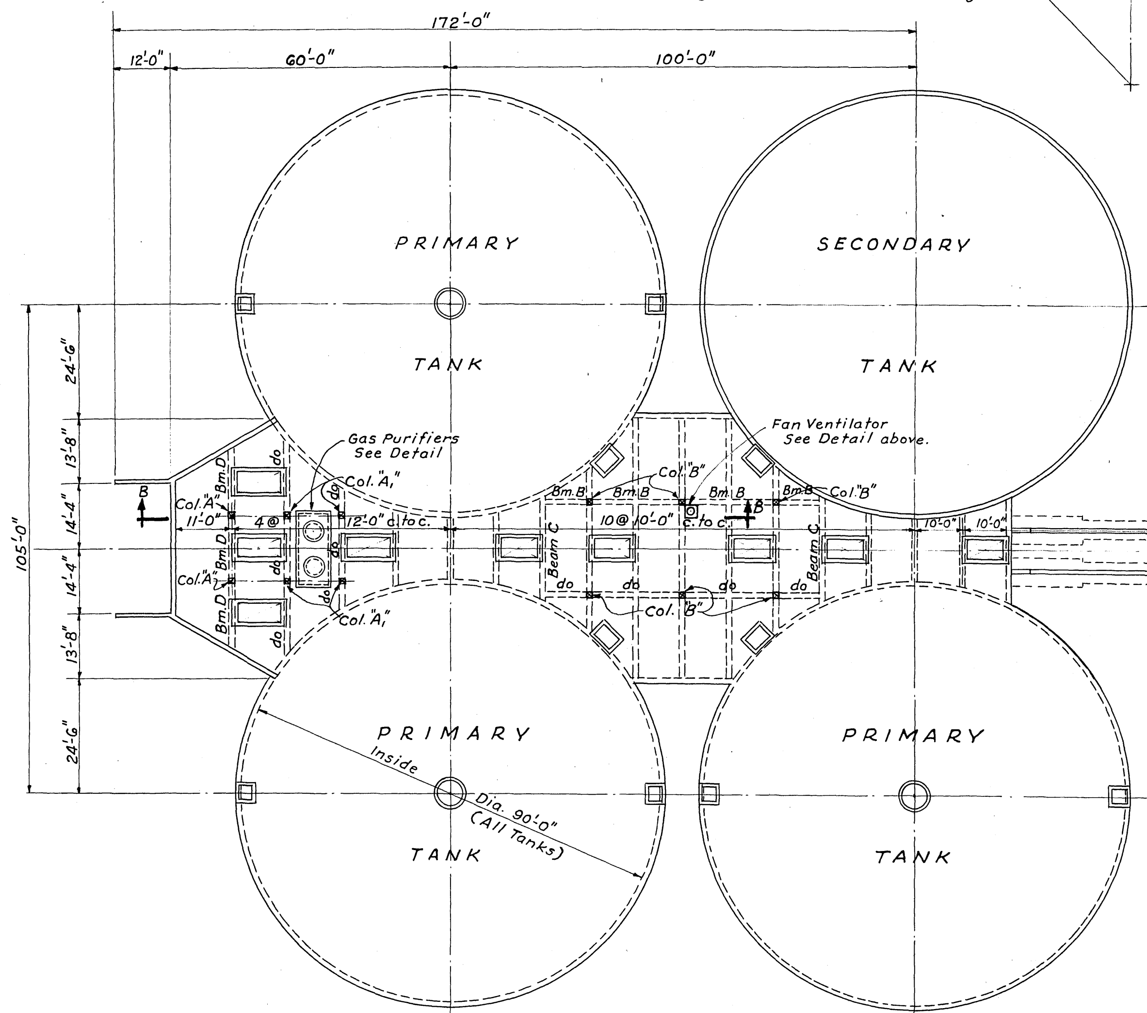
ROOF PLAN OF DIGESTION TANKS
