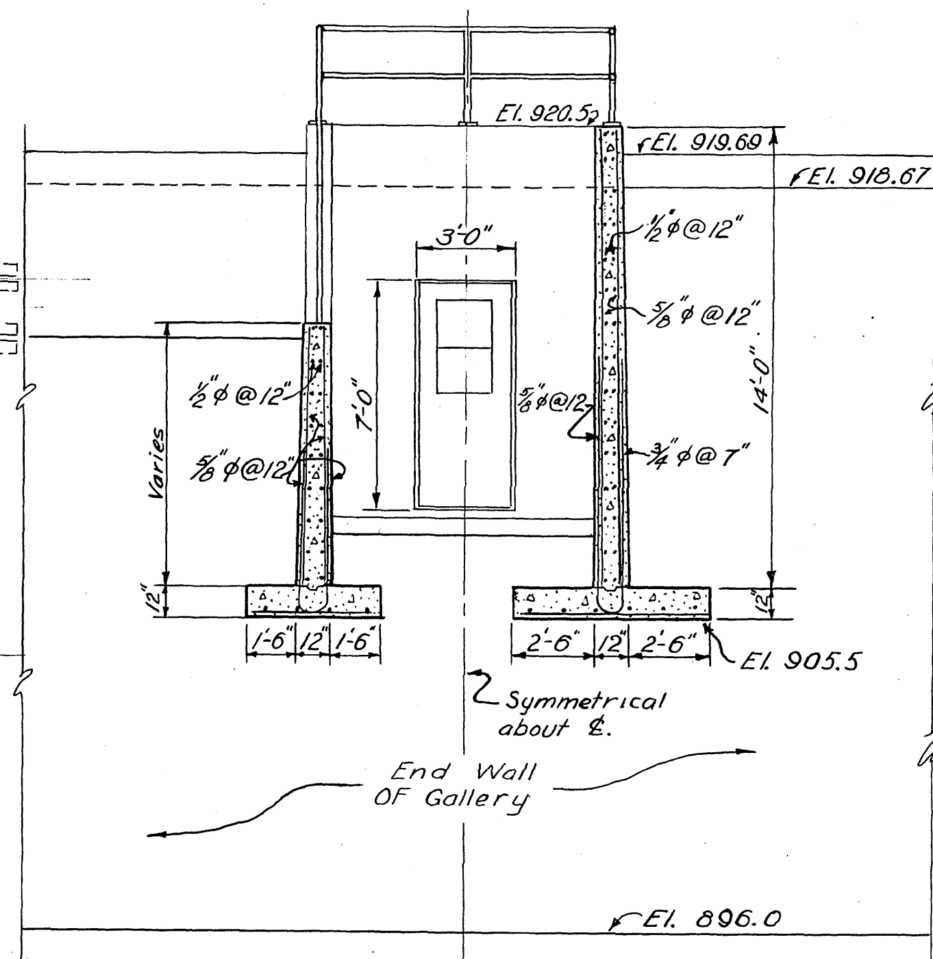
SECTION G-G
