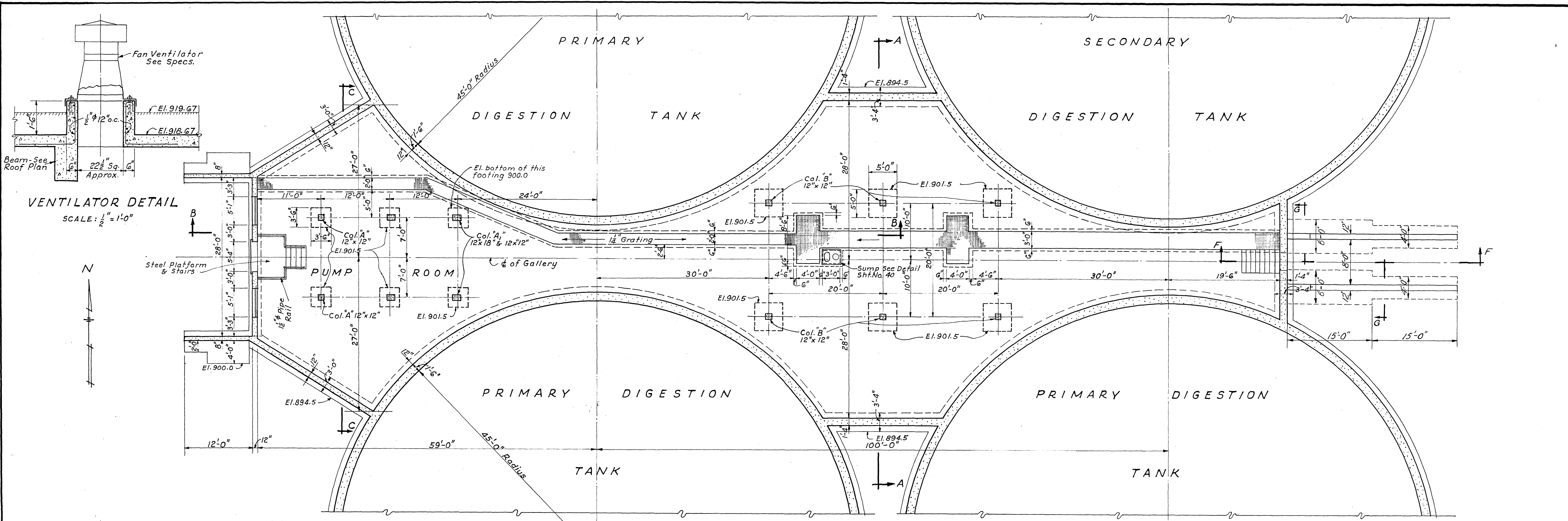
PART PLAN OF PUMP ROOM & GALLERY
