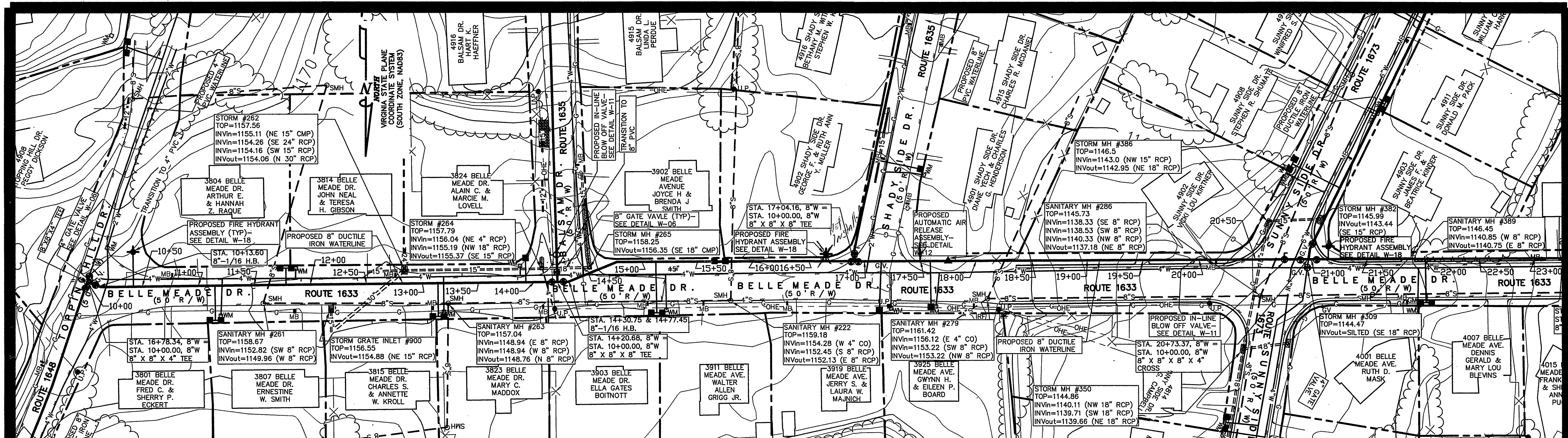
BELLE MEADE DR. SEC. A PLAN
