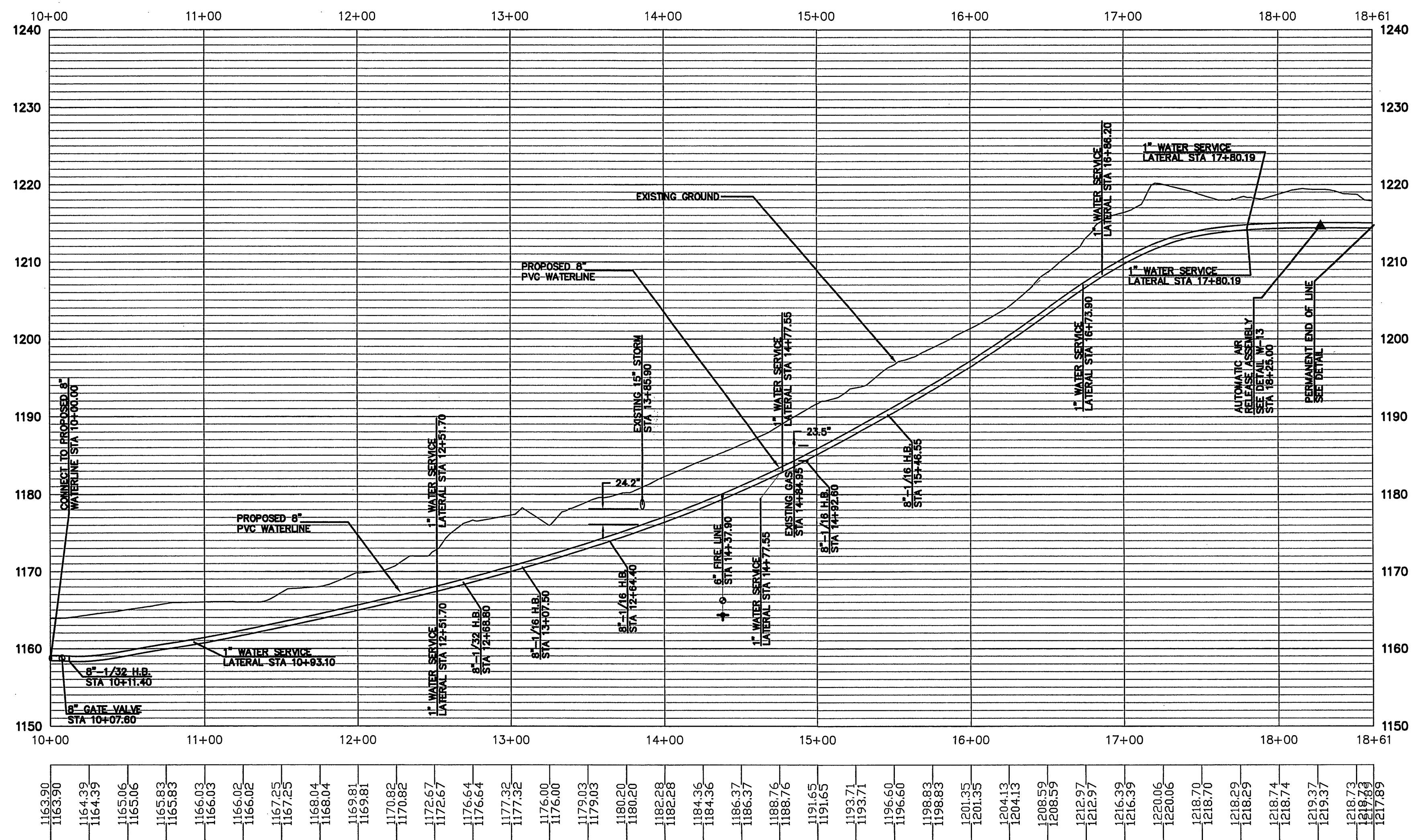
SHADY SIDE DR. SEC. PROFILE SCALE: 1"=50'H, 1"=10'V
