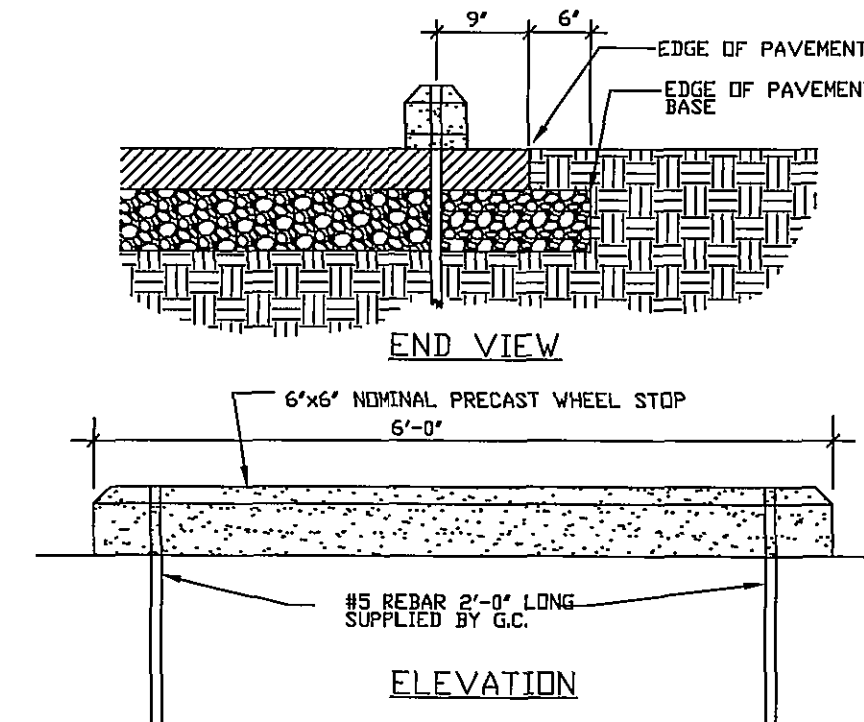
CONCRETE BUMPER BLOCK DETAIL NO SCALE
