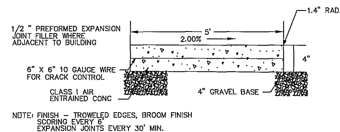
R.O.W. SIDEWALK DETAIL NO SCALE
