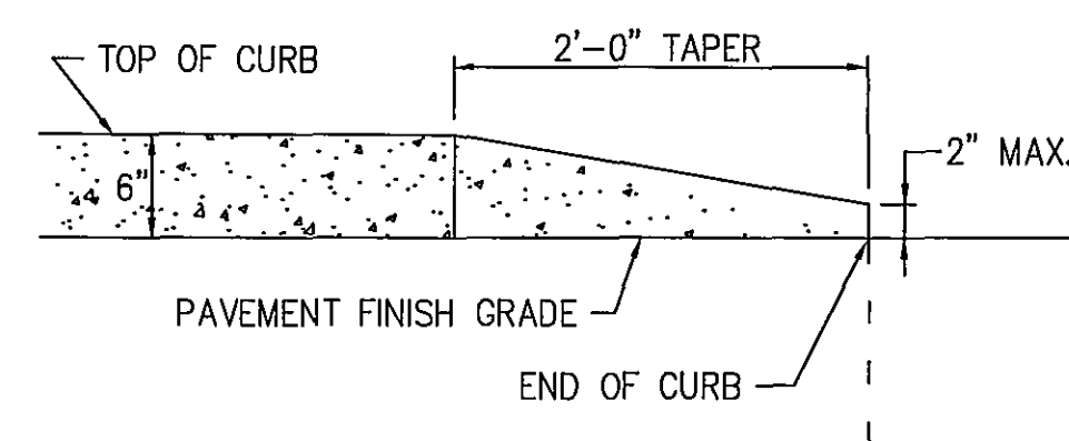
CURB TAPER DETAIL - SECTION NO SCALE
