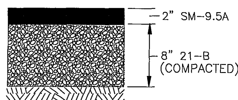
STD ASPHALT PAVEMENT SECTION NO SCALE
