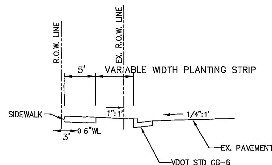
TYPICAL ROAD SECTION
