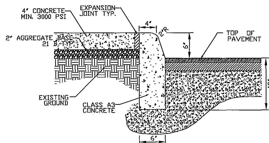
TYPICAL SIDEWALK DETAIL NO SCALE
