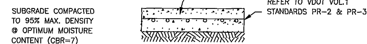
SECTION THROUGH CONCRETE DRIVE NO SCALE
