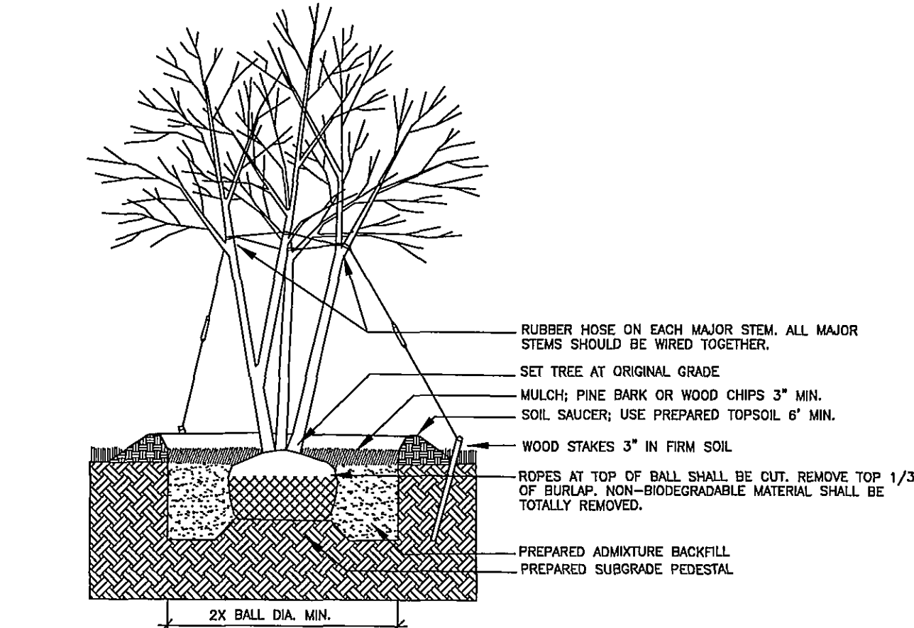
MULTI-STEM PLANTING DETAIL N.T.S.
