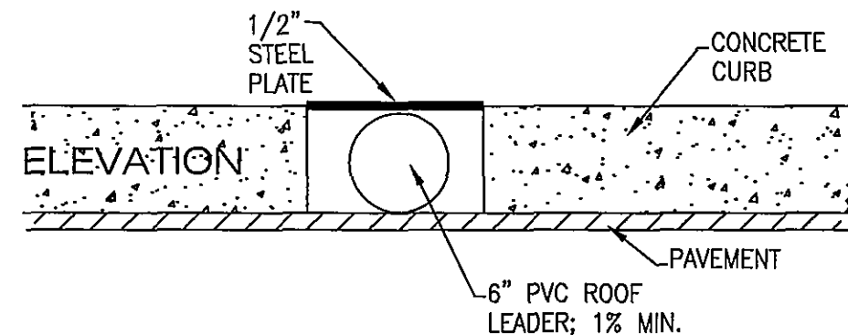
ROOF LEADER/SIDEWALK NO SCALE
