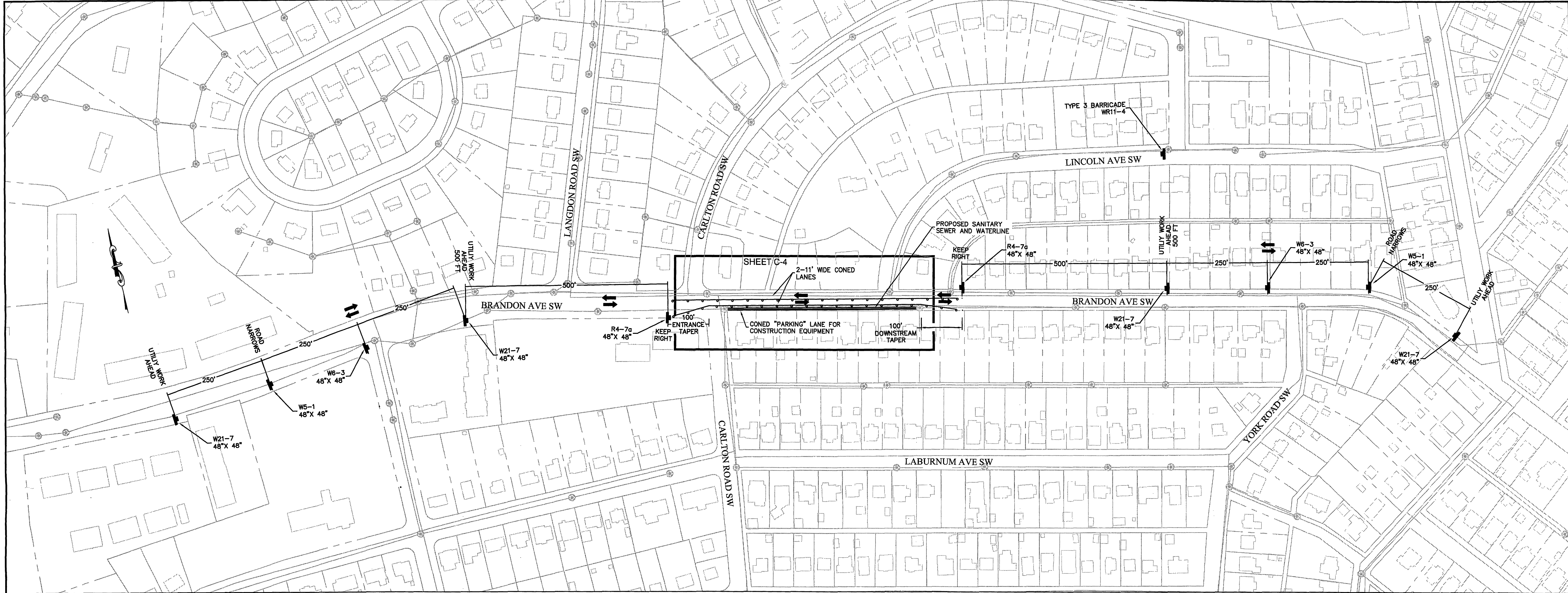
BRANDON AVENUE SEWER REPLACEMENT SCALE: 1"=120'
