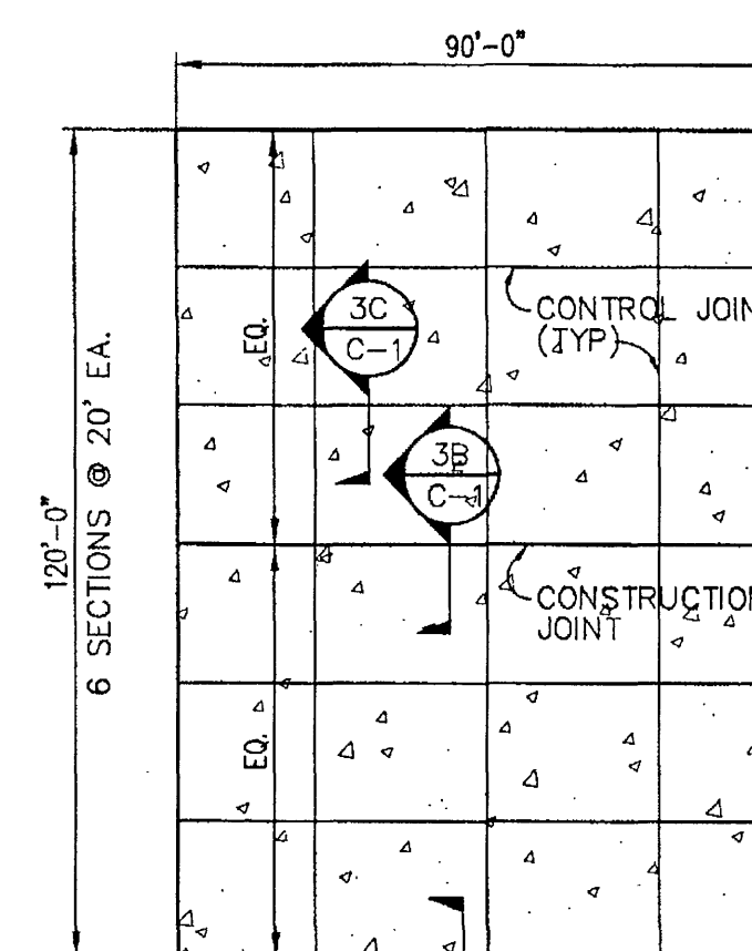
CONCRETE SLAB PLAN 2 SCALE: 1" = 30'
