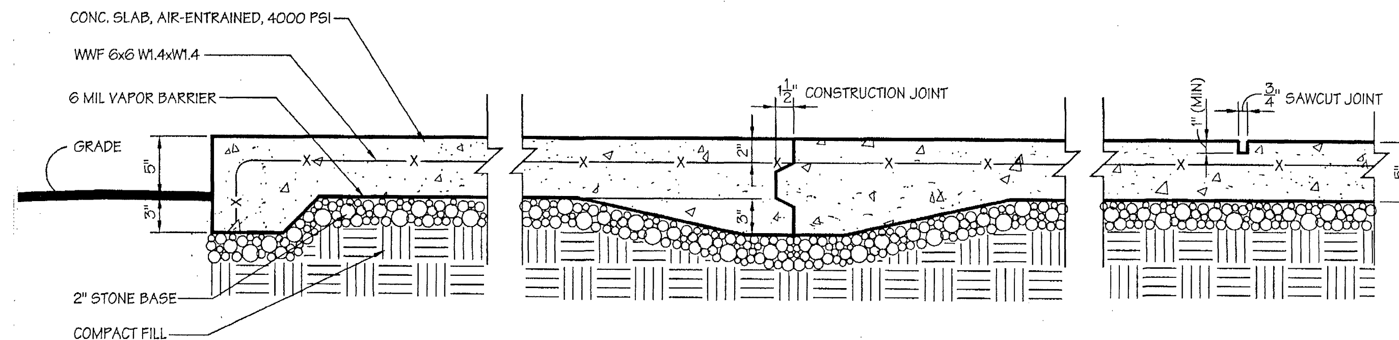
DETAIL-TURNED DOWN SLAB 3A SCALE: 1 1/2" = 1'-0"
