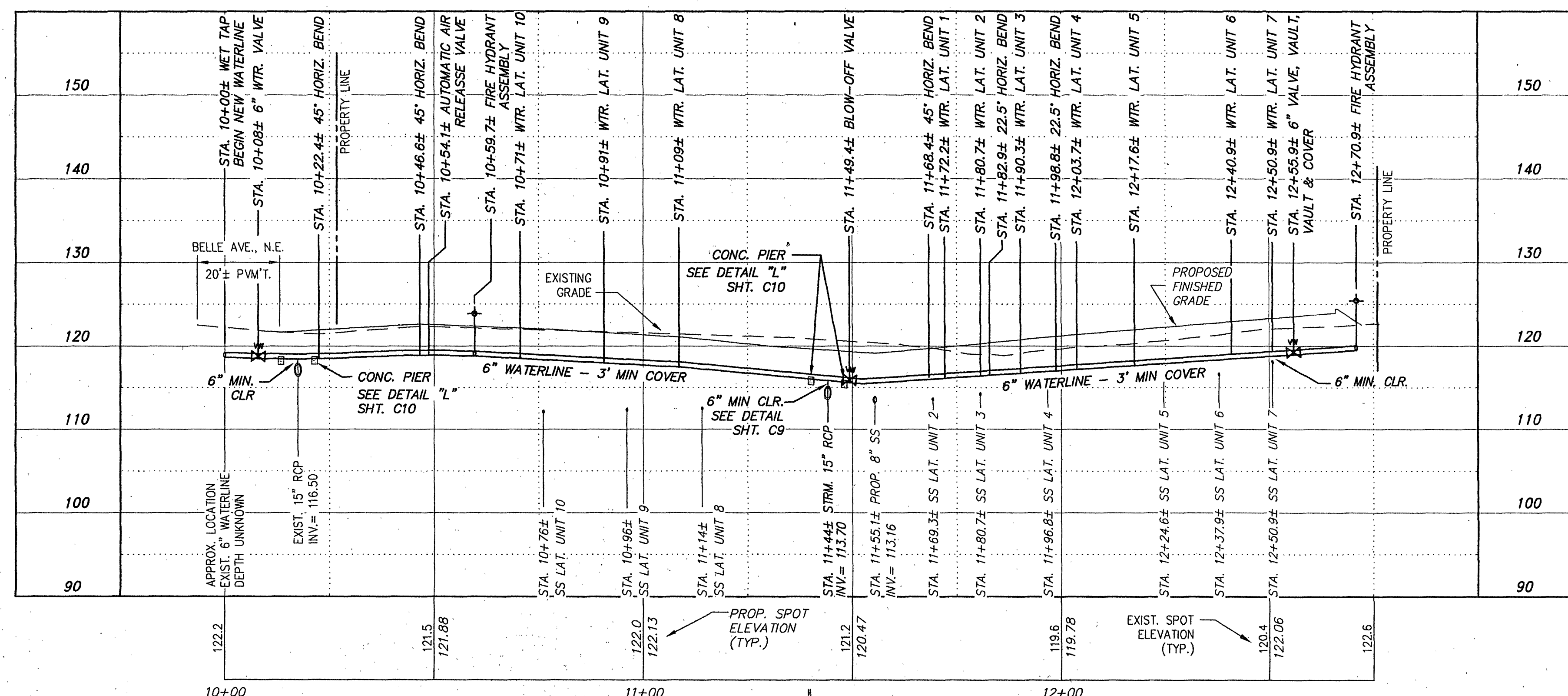
PROFILE: WATERLINE SCALES: 1" = 20' HORIZ. 1" = 10' VERT.
