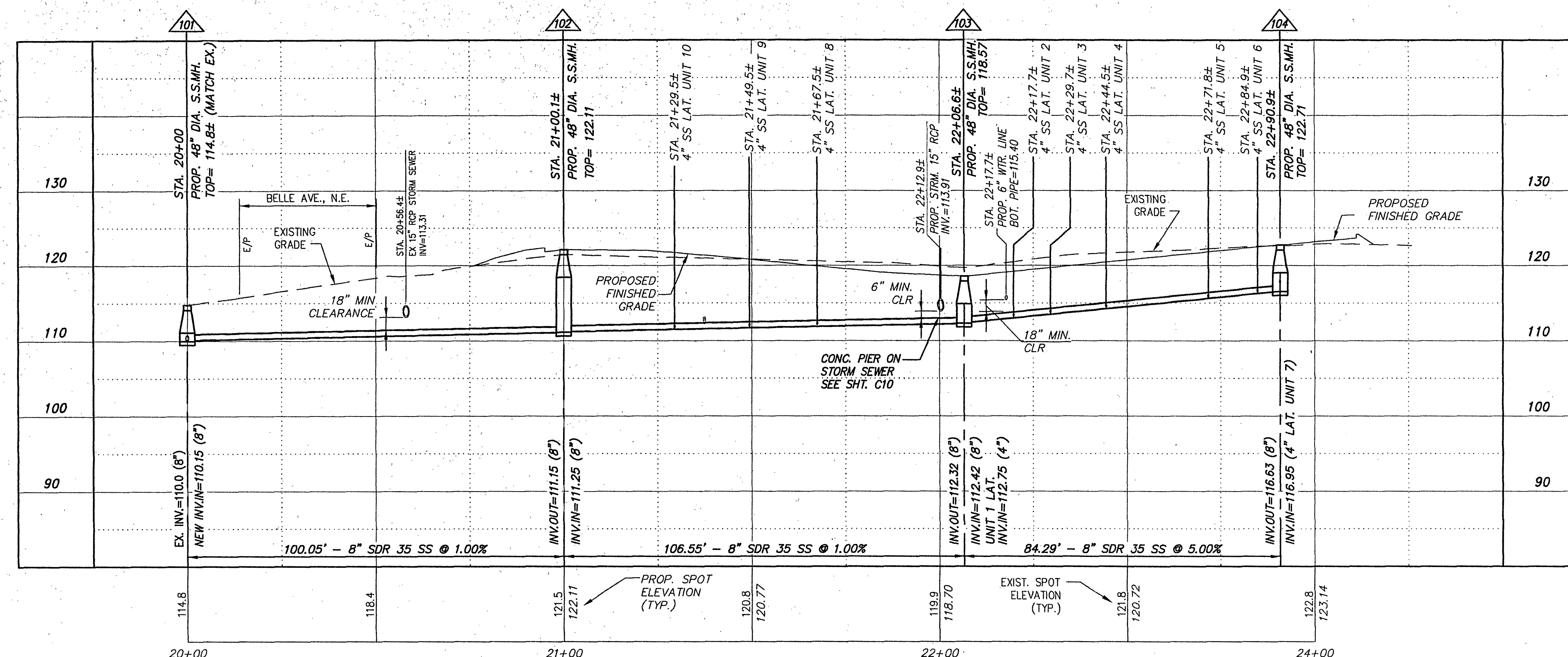
PROFILE: SANITARY SEWER SCALES: 1" = 20' HORIZ. 1" = 10' VERT.
