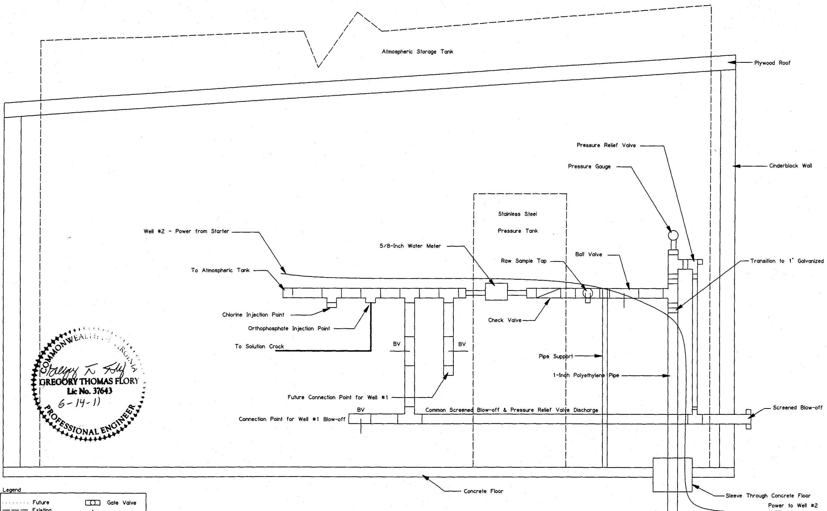
Well #2 Pumphouse Detail - Profile
