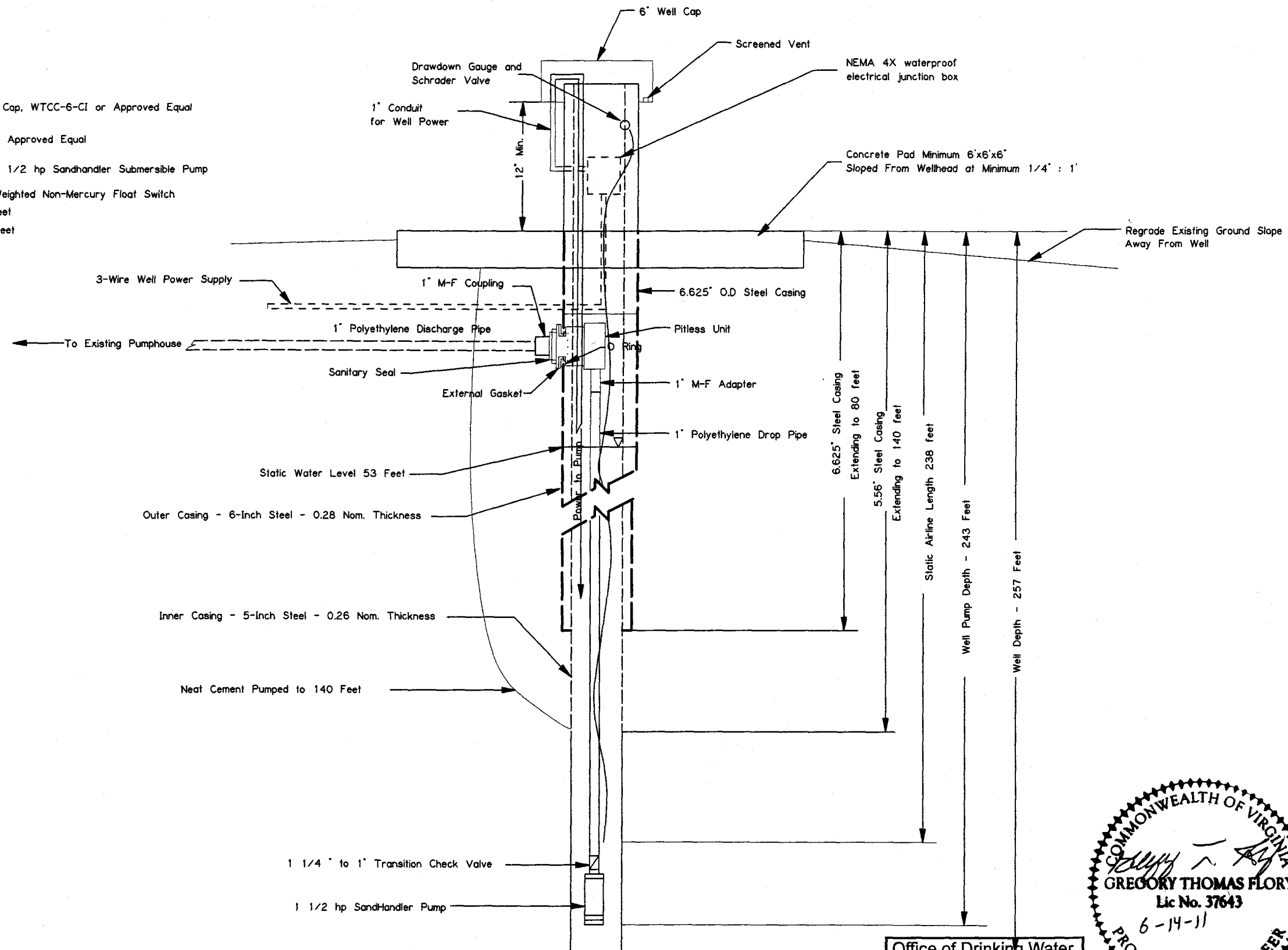
Well #2 - Wellhead Detail
