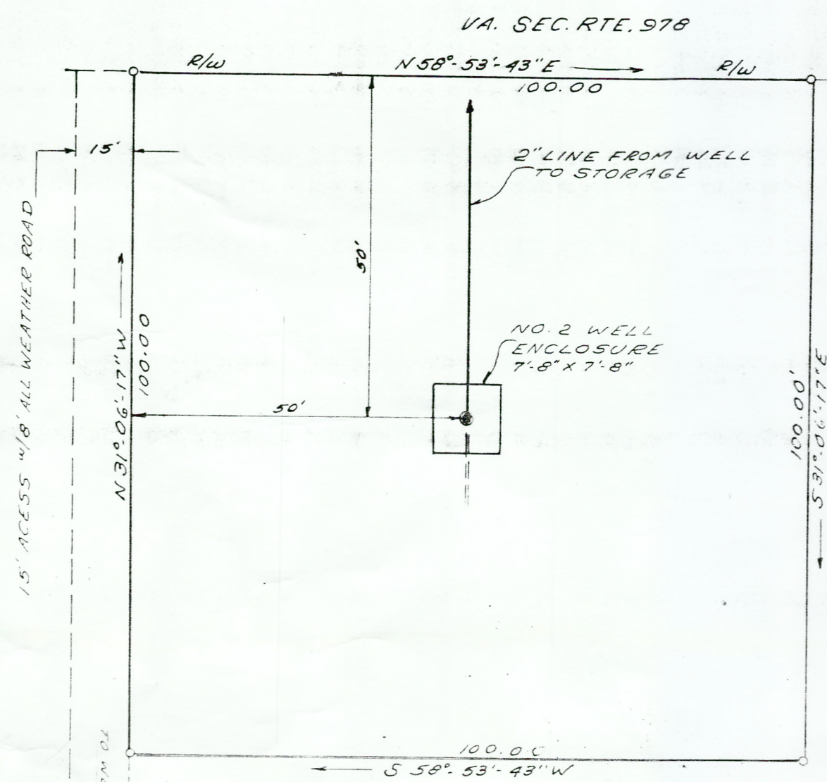
DETAIL - WELL LOT NO. 2 SCALE 1"=120 FT.
