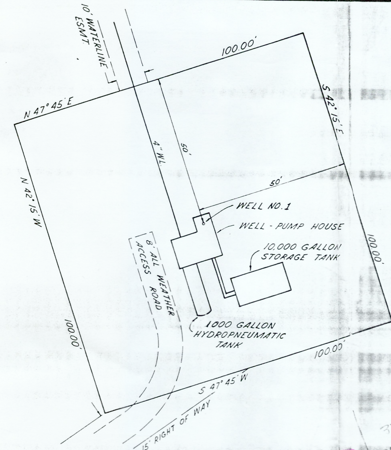
WELL LOT DETAIL SCALE 1"=20'
