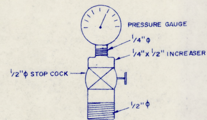
PORTABLE DRAWDOWN GAUGE ASSEMBLY - DETAIL N.T.S.
