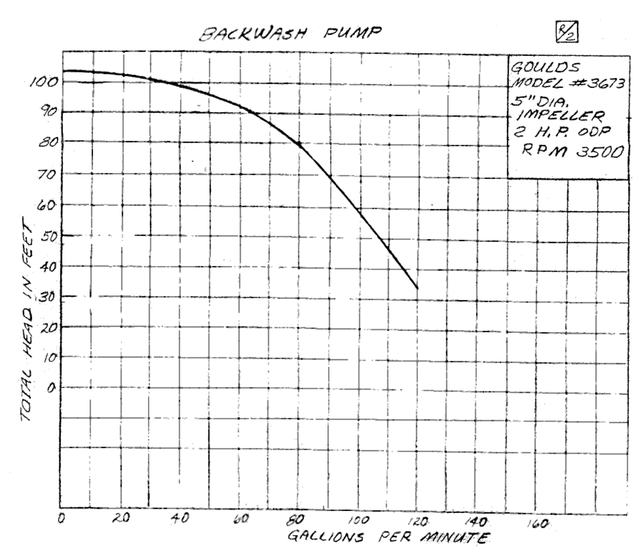
PERFORMANCE CURVES
