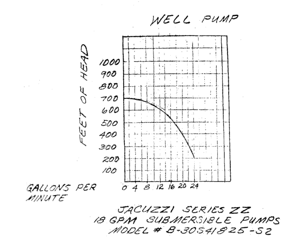
PERFORMANCE CURVES
