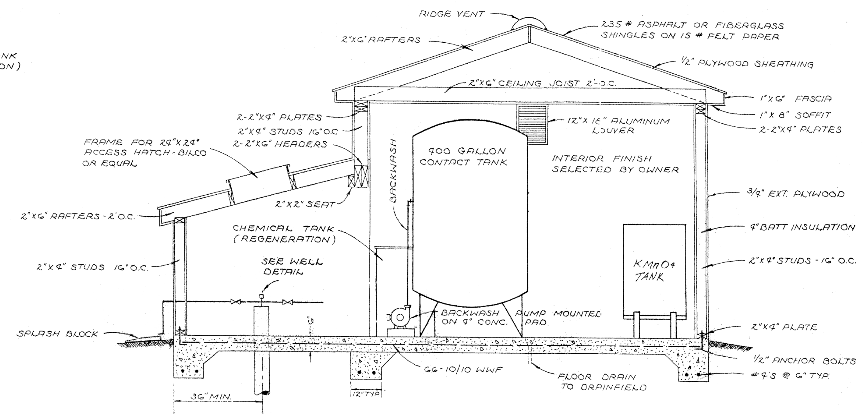
SECTION A-A NTS
