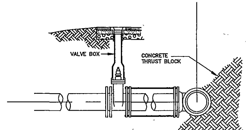
WATER LINE VALVE INSTALLATION
