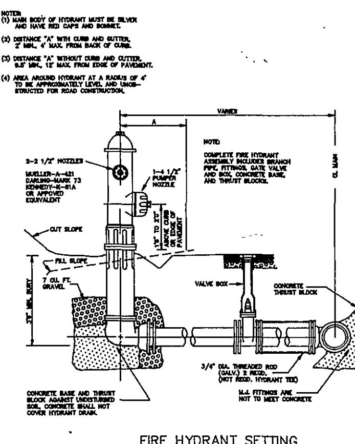
FIRE HYDRANT SETTING
