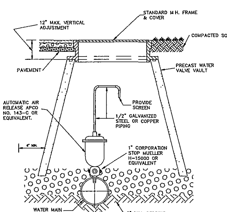
AUTOMATIC AIR RELEASE ASSEMBLY
