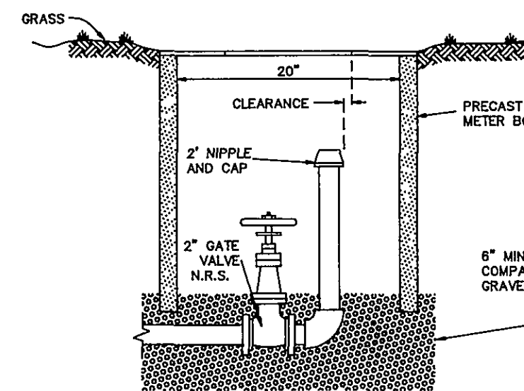
TYPICAL BLOW-OFF ASSEMBLY (OUT OF PAVEMENT)
