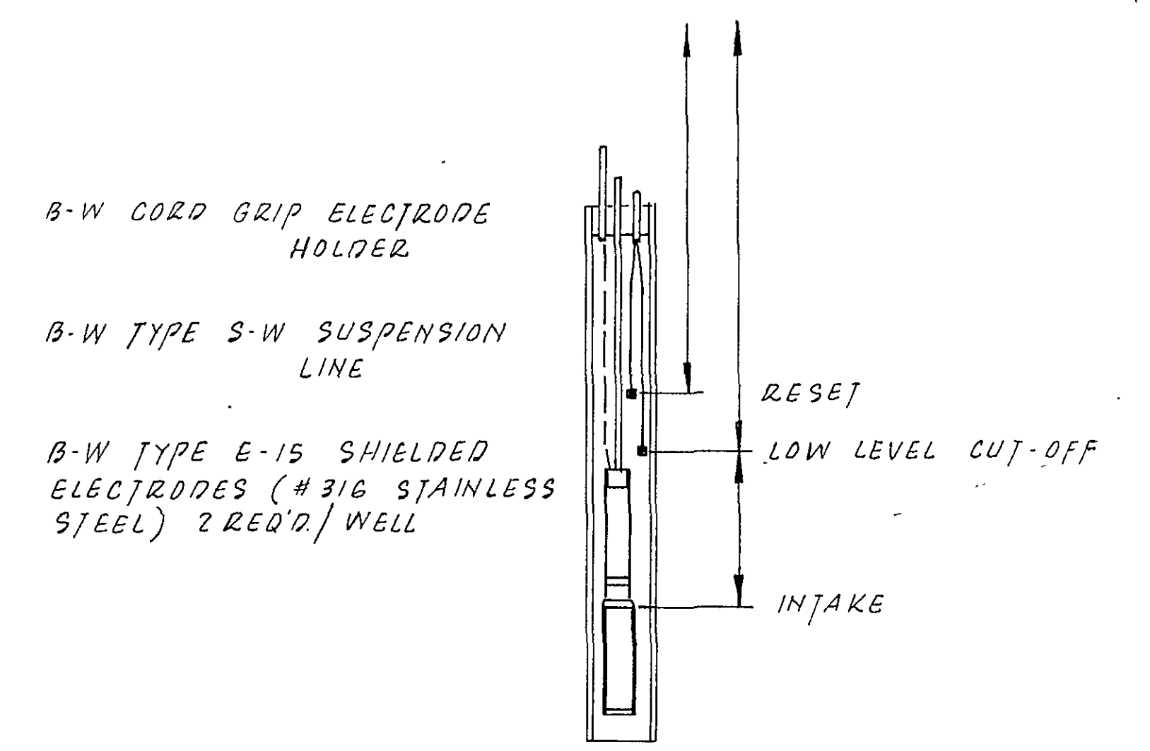
PUMP CONTROLS SCHEMATIC
