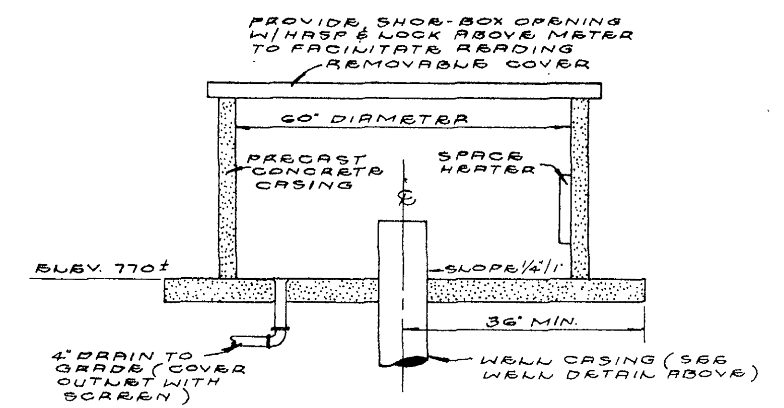
WELL HOUSING DETAIL
