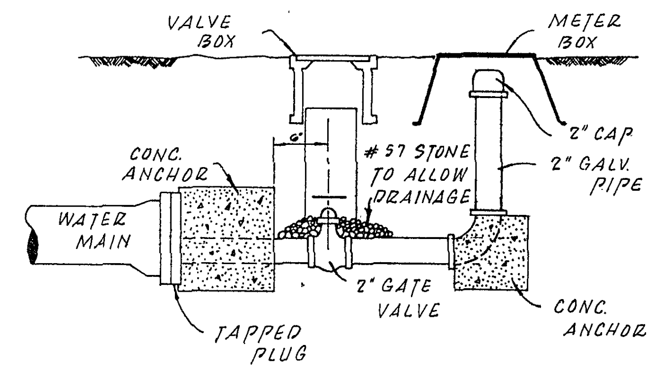
2" BLOW-OFF ASSEMBLY
