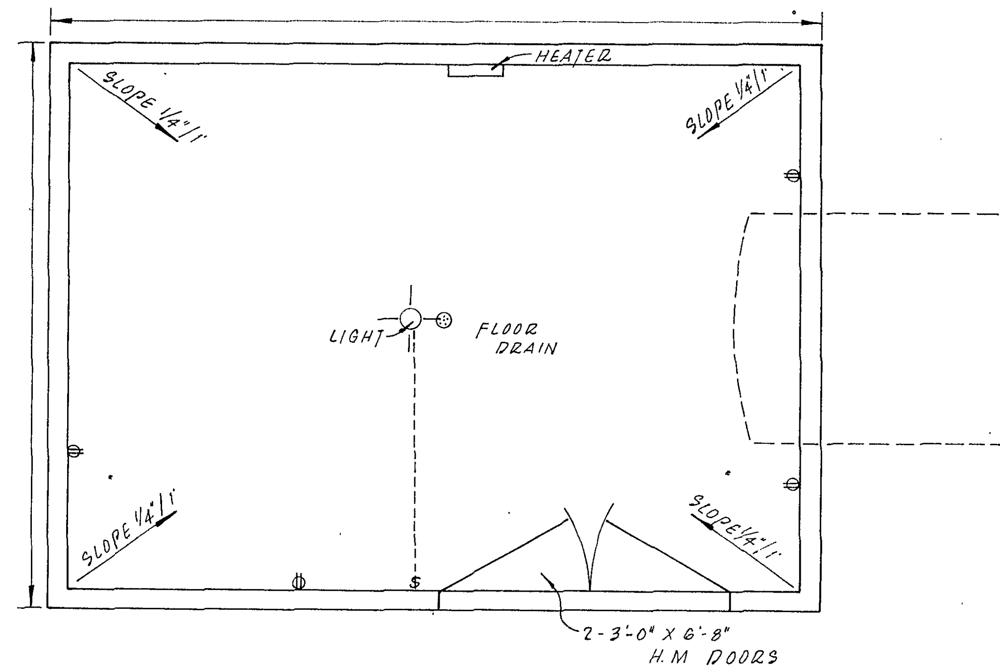
PUMP HOUSE PLAN
