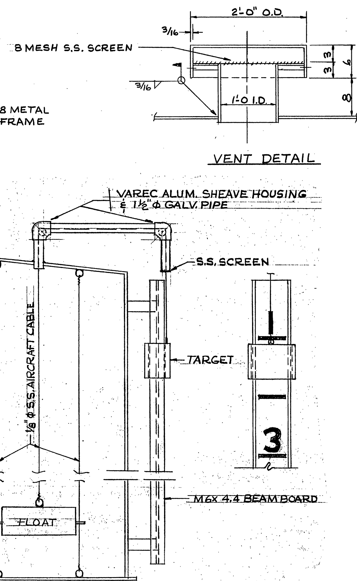
LIQUID LEVEL GAUGE DETAILS
