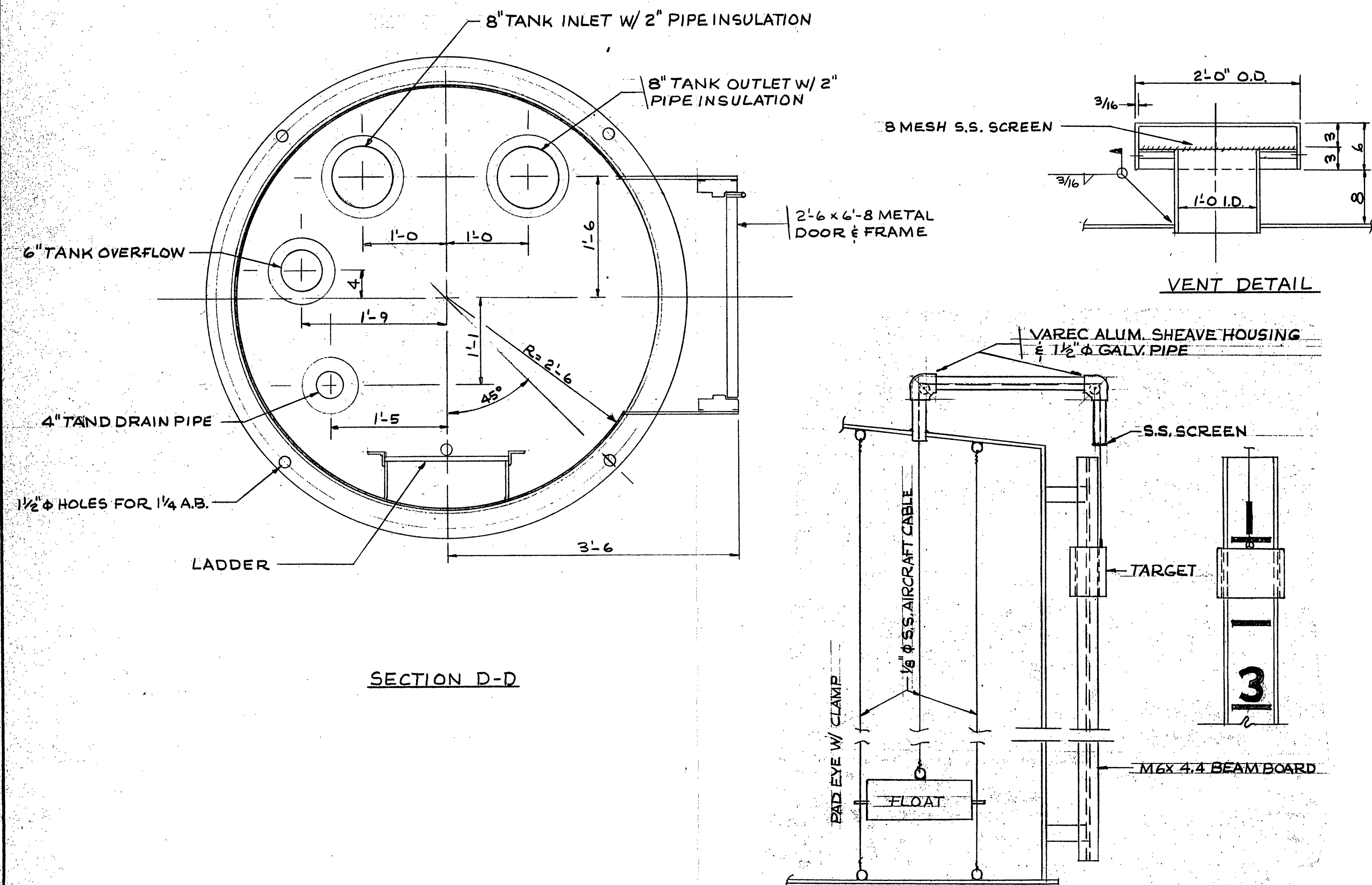
LIQUID LEVEL GAUGE DETAILS
