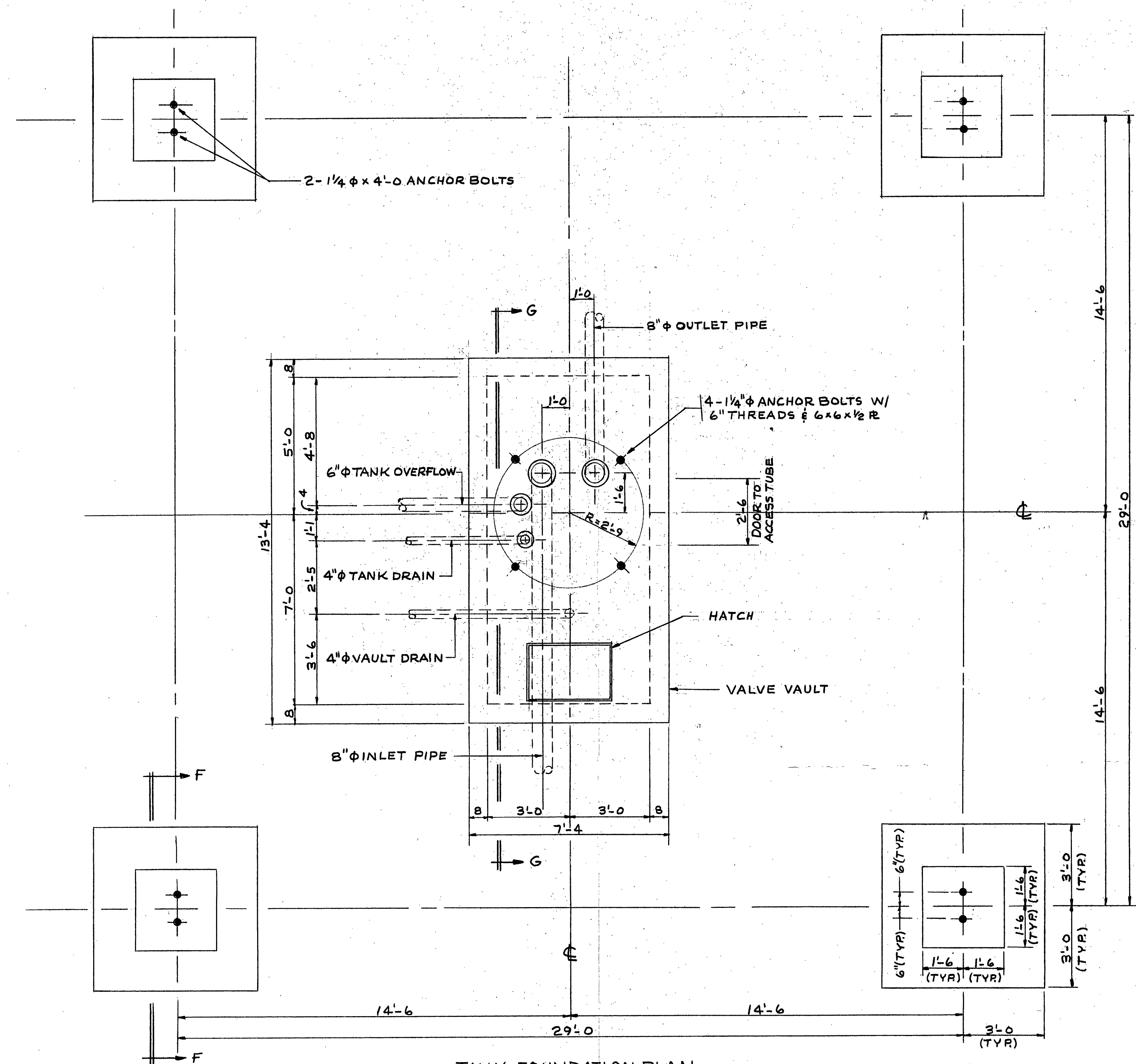
TANK FOUNDATION PLAN
