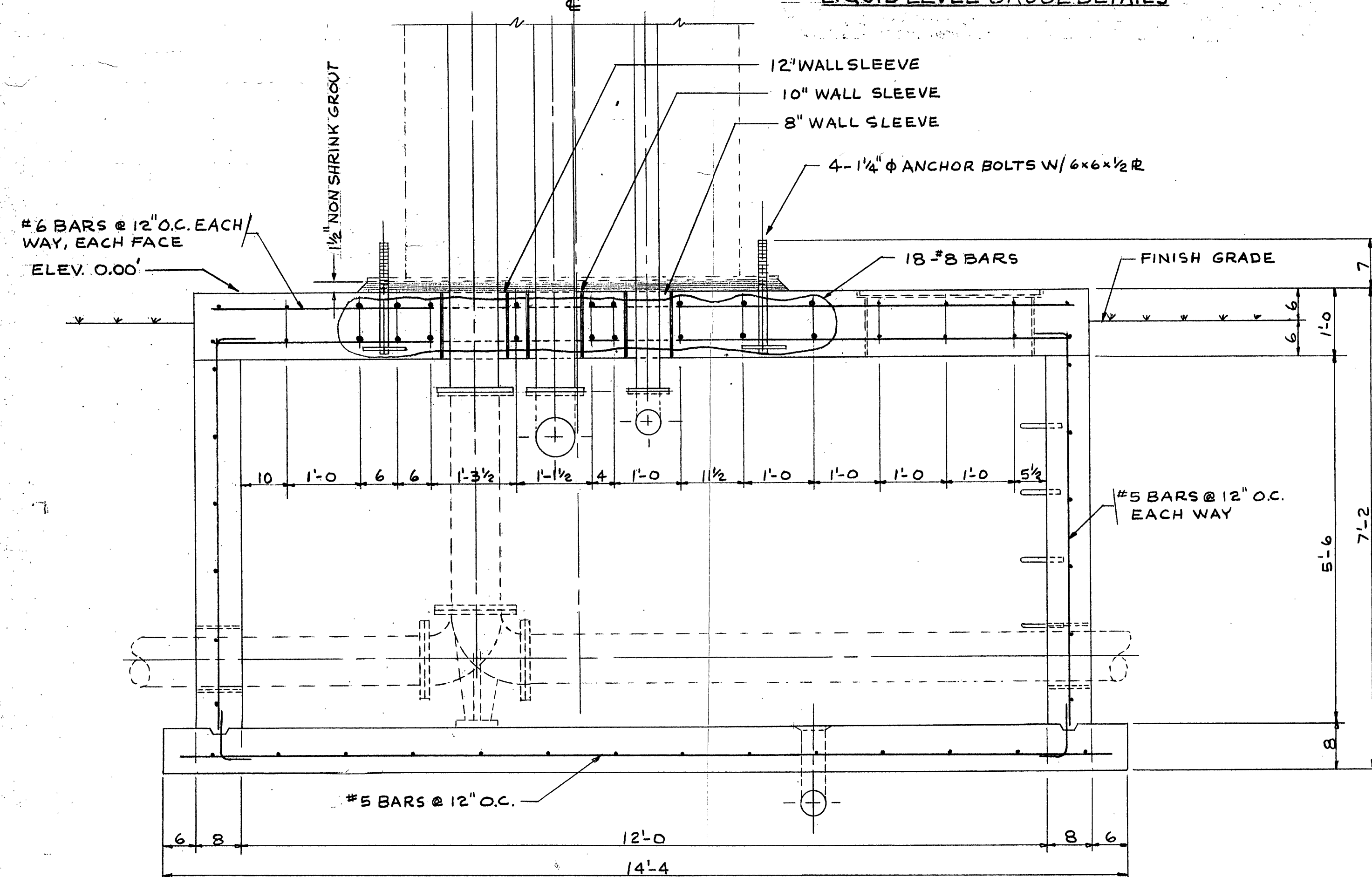
SECTION G-G
