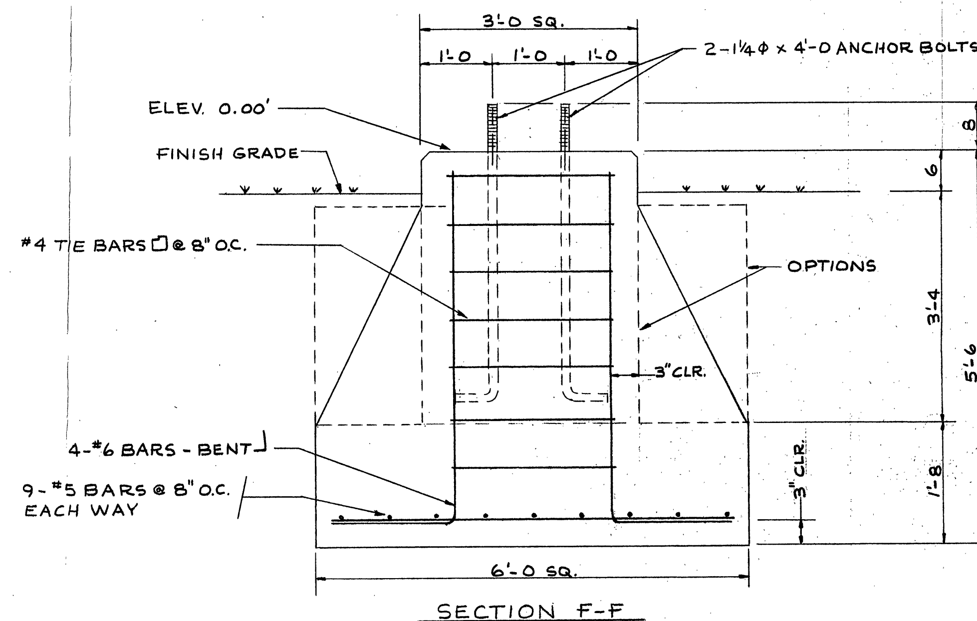
SECTION F-F
