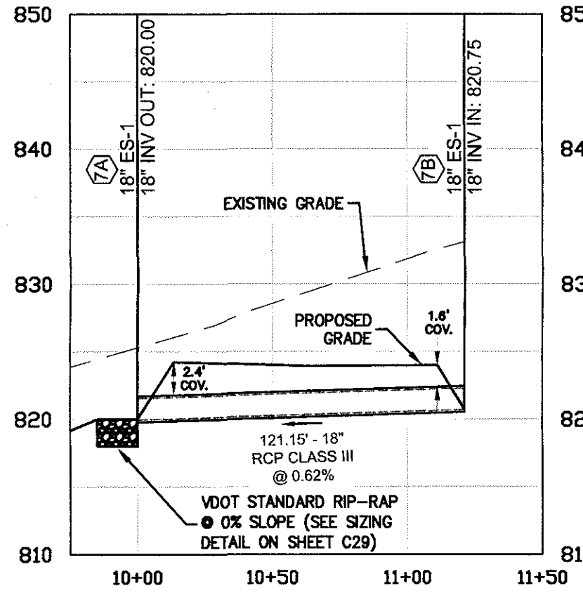
STORM - 7B-7A PROFILE 1" = 30' Horizontal 1" = 6' Vertical
