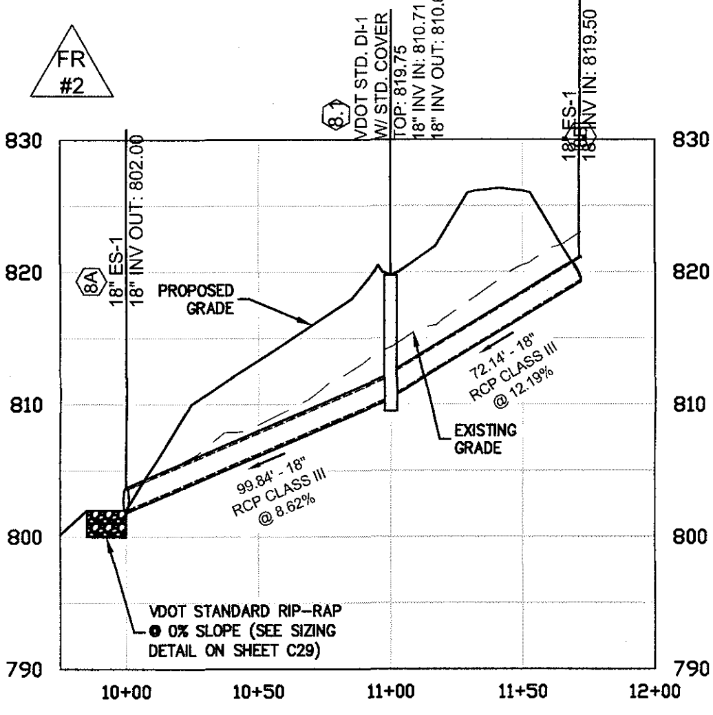
STORM 8B-8A PROFILE 1" = 30' Horizontal 1" = 6' Vertical
