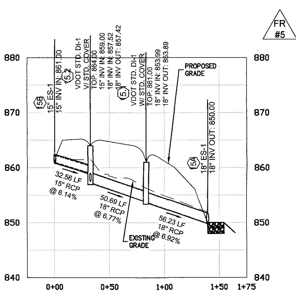
STORM 15B-15A PROFILE 1" = 30' Horizontal 1" = 6' Vertical
