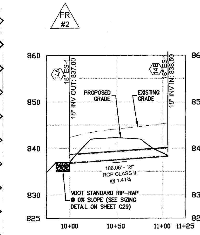
STORM 14B-14A PROFILE 1" = 30' Horizontal 1" = 6' Vertical
