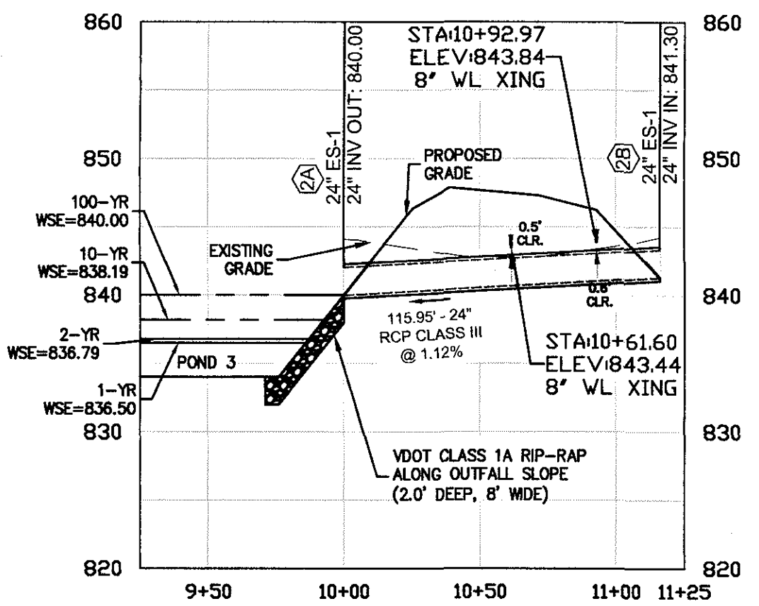
STORM - 2B-2A PROFILE 1" = 30' Horizontal 1" = 6' Vertical
