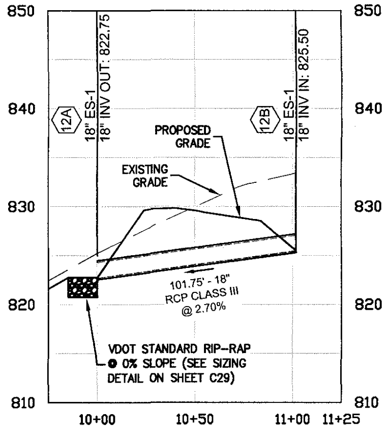
STORM 12B-12A PROFILE 1" = 30' Horizontal 1" = 6' Vertical
