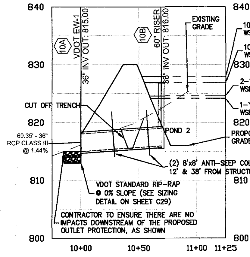
STORM - 10B-10A PROFILE 1" = 30' Horizontal 1" = 6' Vertical
