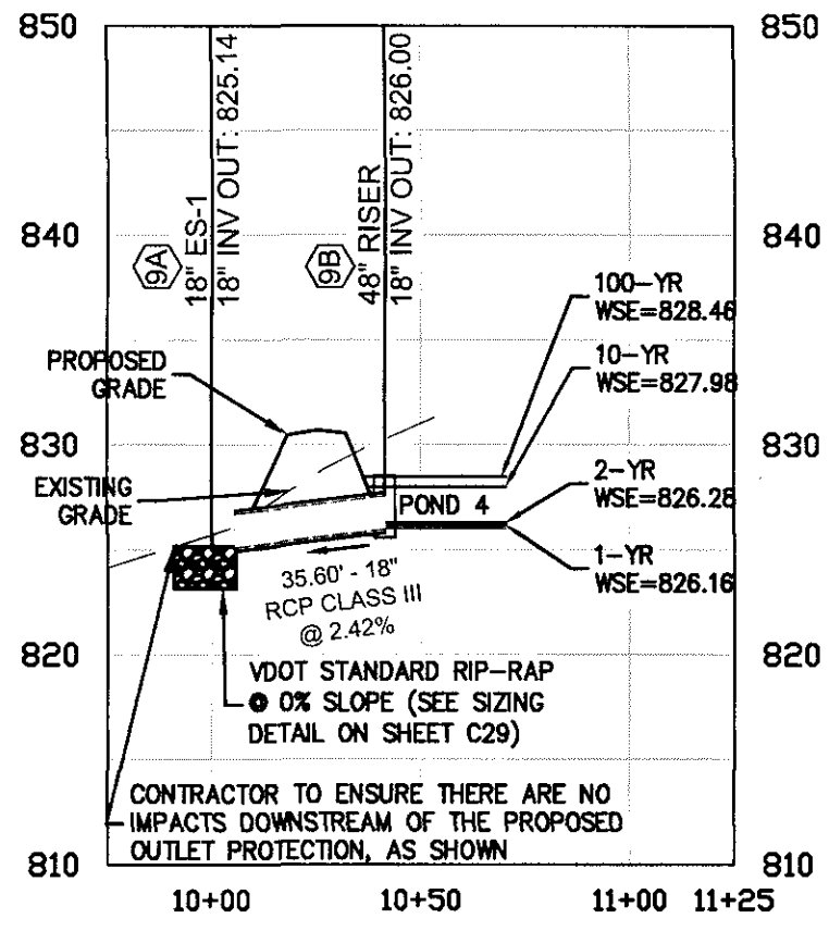
STORM - 9B-9A PROFILE 1" = 30' Horizontal 1" = 6' Vertical
