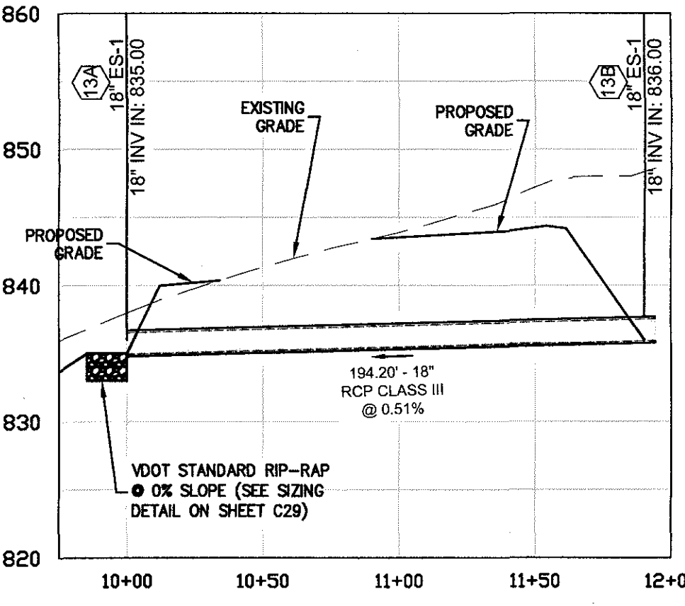
STORM 13B-13A PROFILE 1" = 30' Horizontal 1" = 6' Vertical
