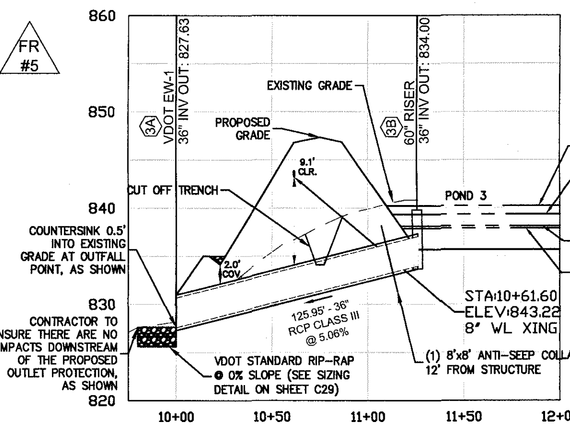
STORM - 3B-3A PROFILE 1" = 30' Horizontal 1" = 6' Vertical
