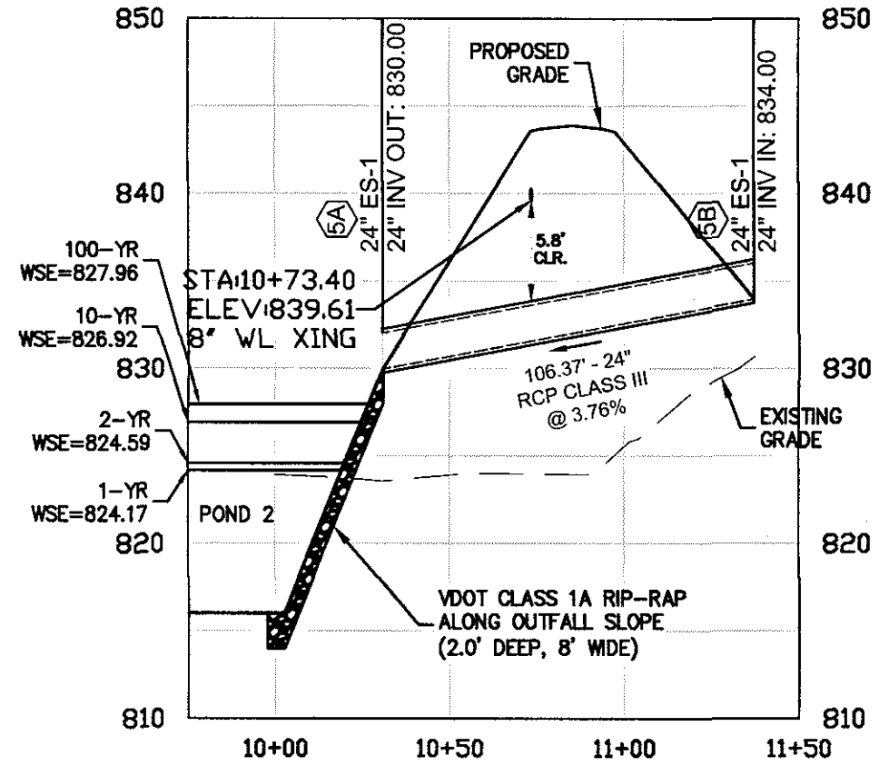
STORM - 5B-5A PROFILE 1" = 30' Horizontal 1" = 6' Vertical
