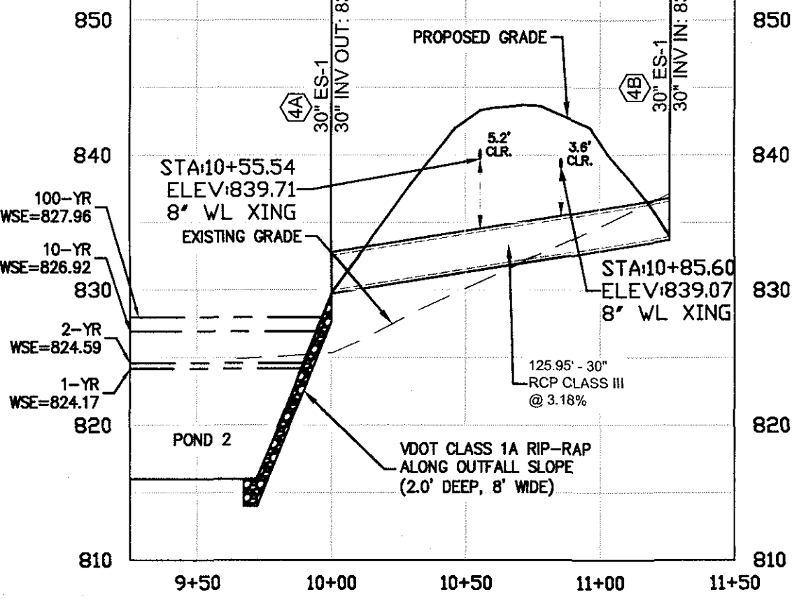
STORM - 4B-4A PROFILE 1" = 30' Horizontal 1" = 6' Vertical
