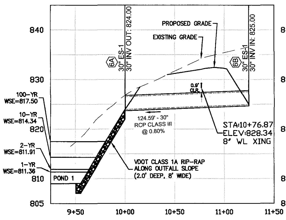
STORM - 6B-6A PROFILE 1" = 30' Horizontal 1" = 6' Vertical
