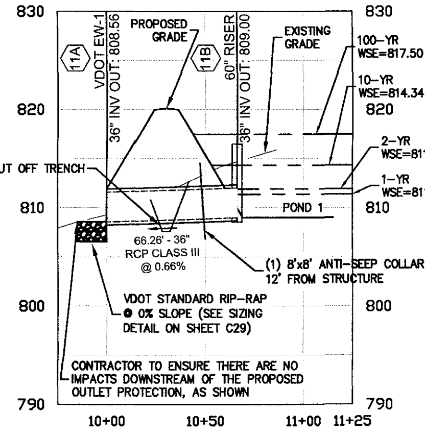
STORM 11B-11A PROFILE 1" = 30' Horizontal 1" = 6' Vertical
