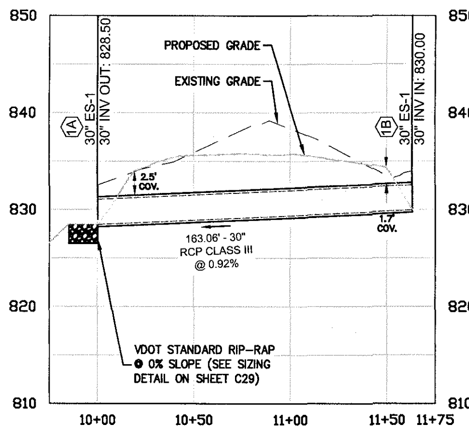
STORM - 1B-1A PROFILE 1" = 30' Horizontal 1" = 6' Vertical
