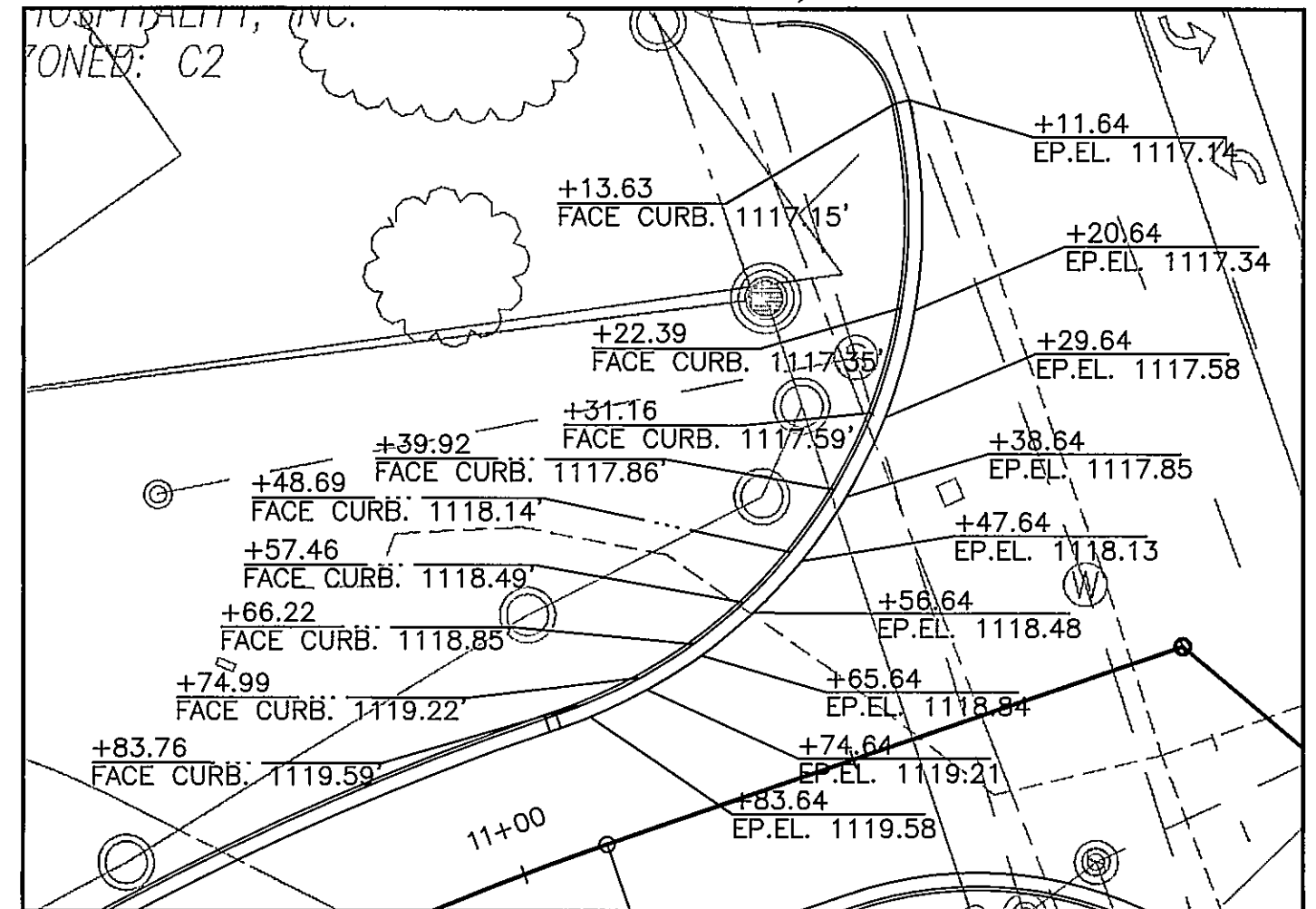
PAVEMENT AND GUTTER PAN WARPING DETAIL SCALE: 1"=25'
