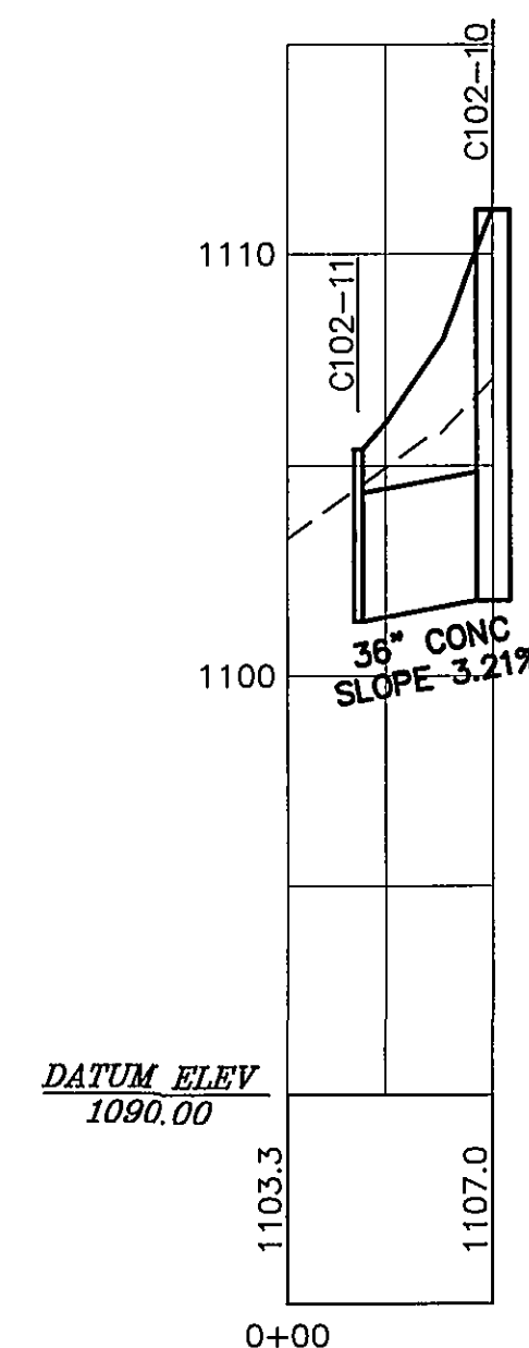
STORM DRAIN PROFILE C102-11 TO C102-10
