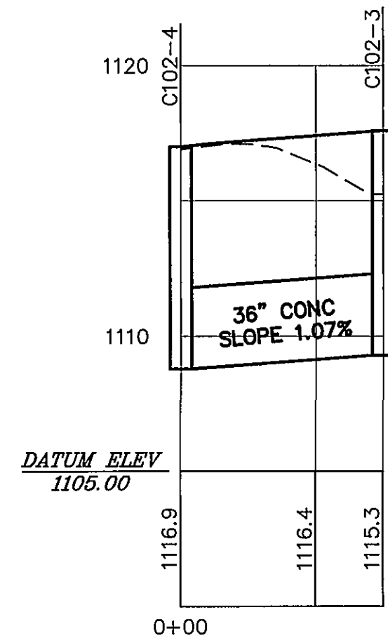
STORM DRAIN PROFILE C102-4 TO C102-3
