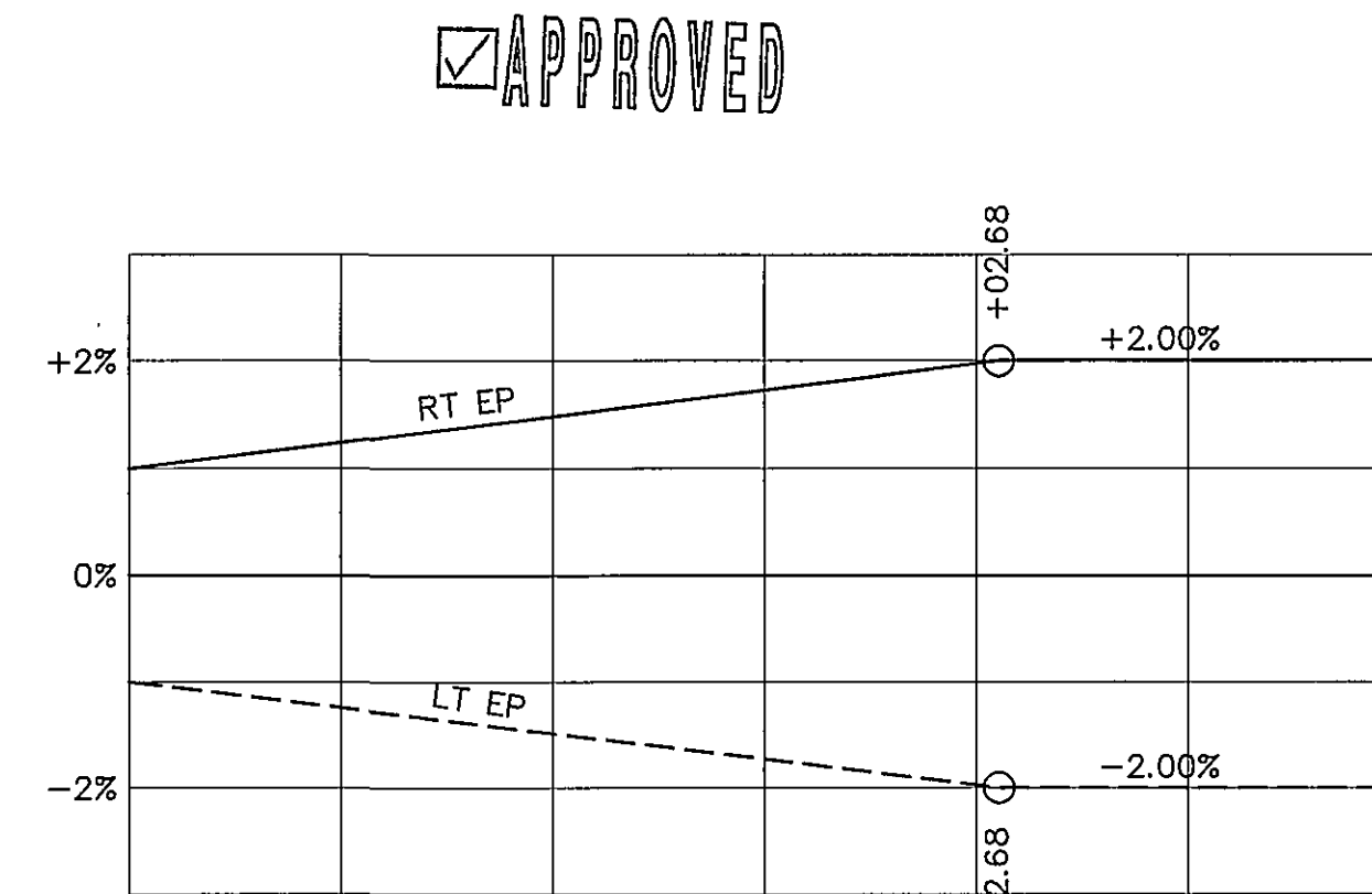
SUPERELEVATION DIAGRAM
