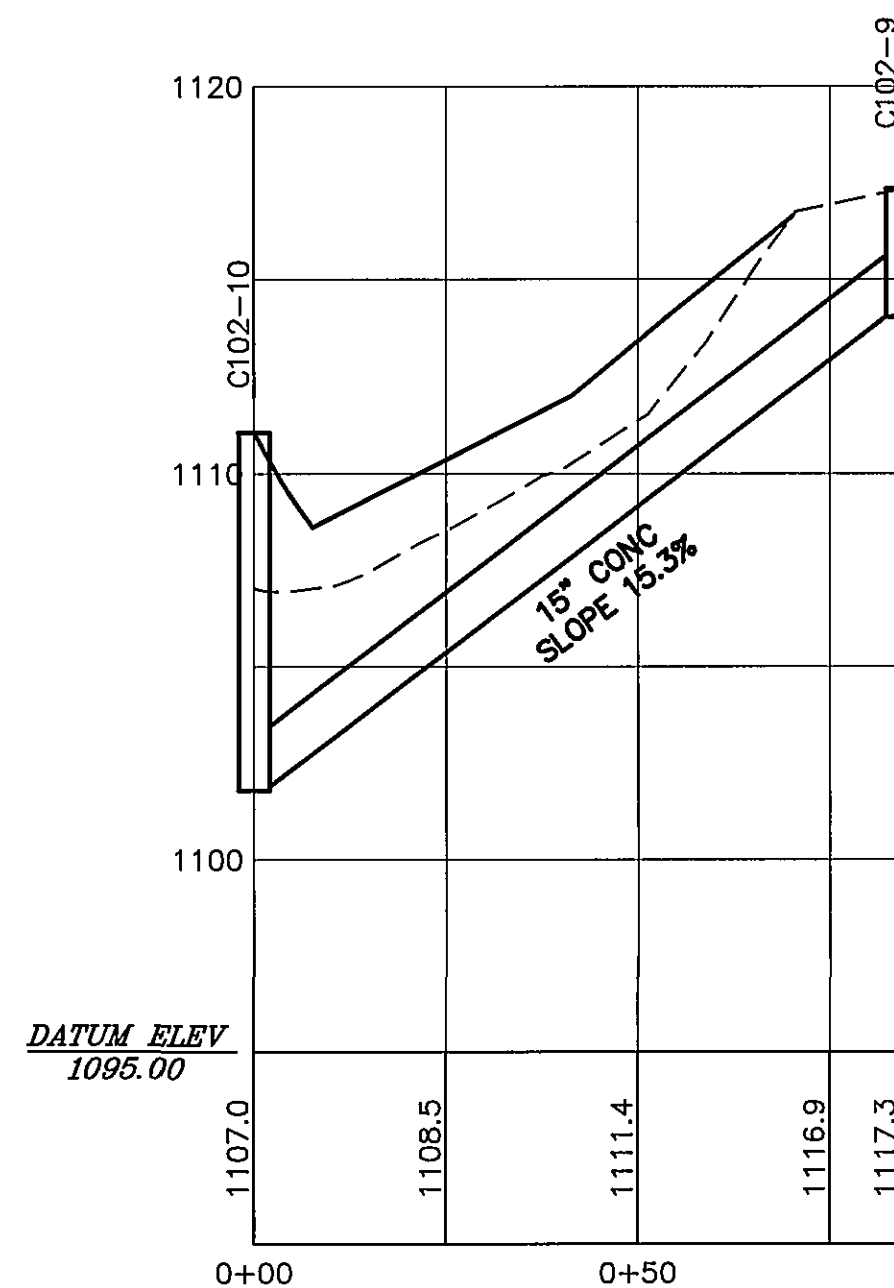
STORM DRAIN PROFILE C102-10 TO C102-9
