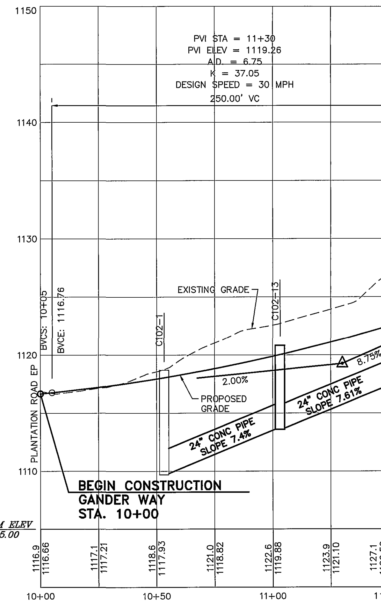
GANDER WAY PROFILE
