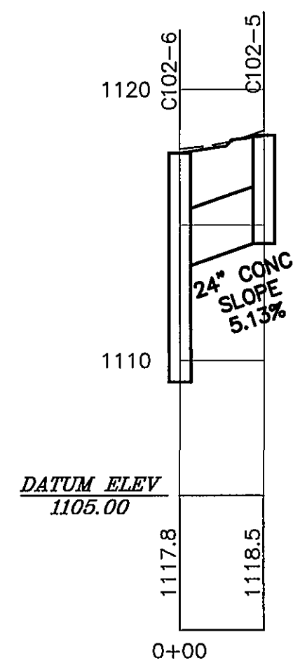
STORM DRAIN PROFILE C102-6 TO C102-5
