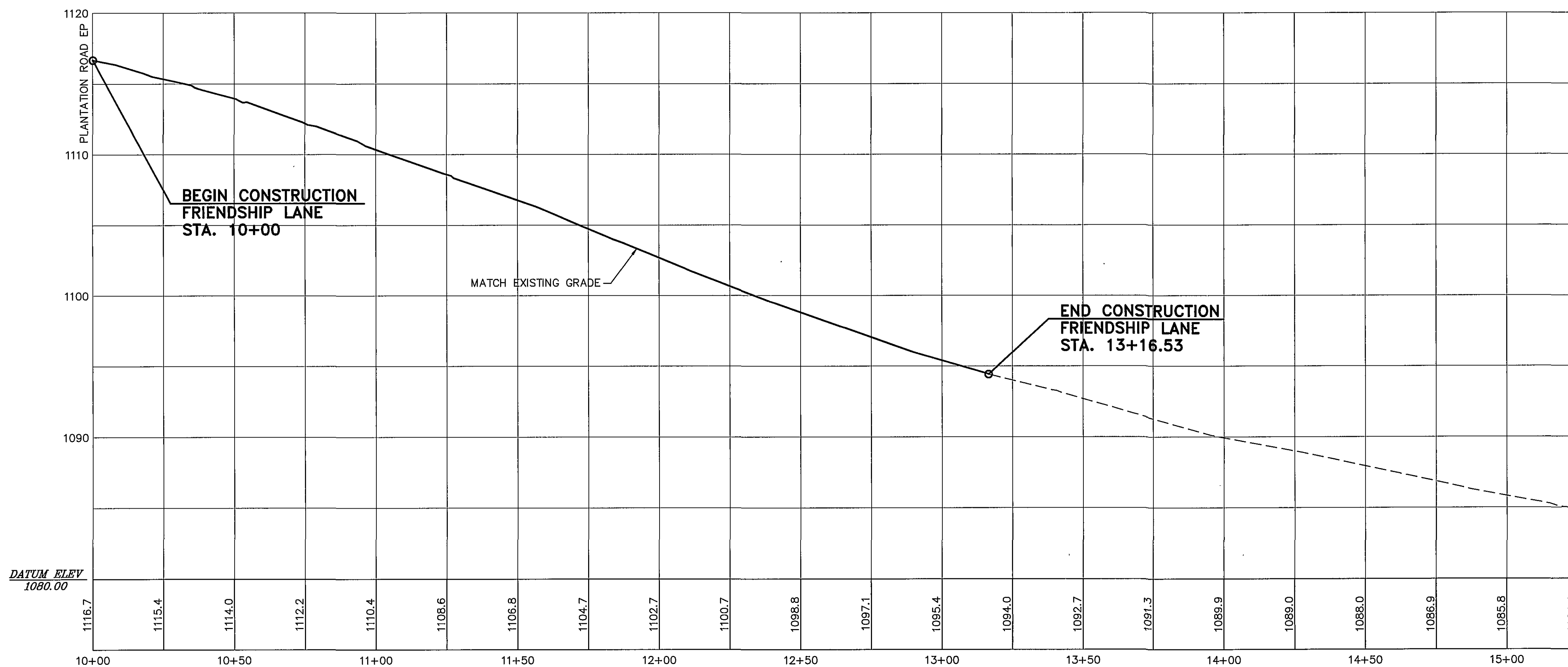
FRIENDSHIP LANE PROFILE
