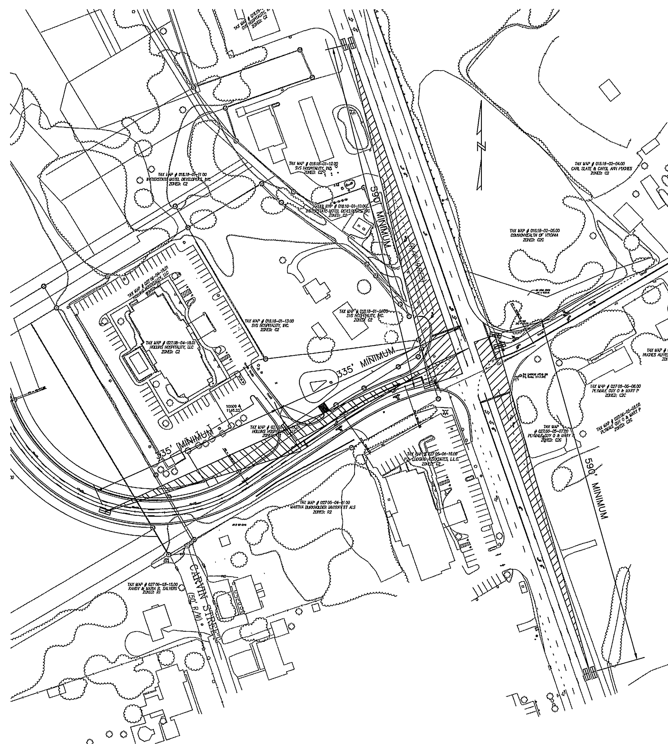
SIGHT DISTANCE TRIANGLES SCALE: 1"=100'
