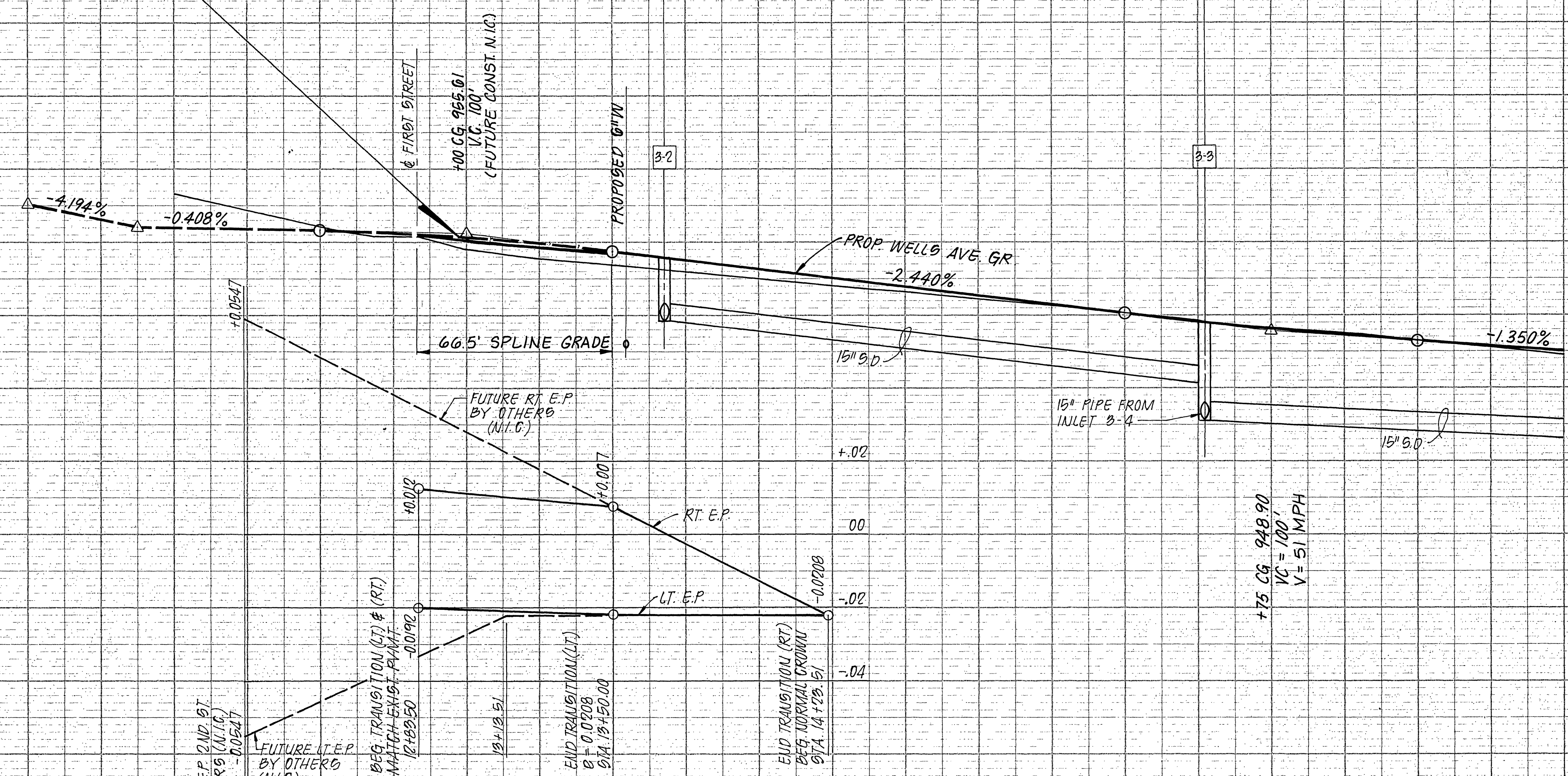
SUPERELEVATION CHART
