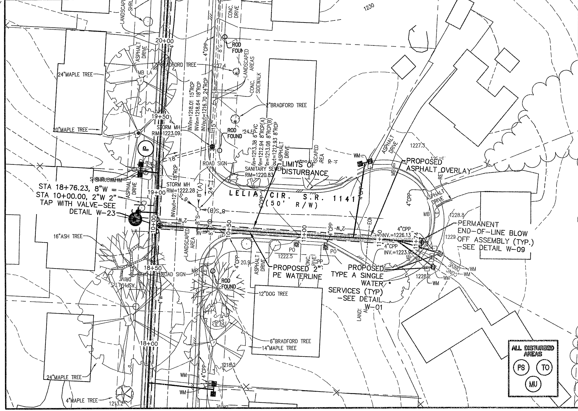
LELIA CIRCLE PLAN SCALE: 1"=30'
