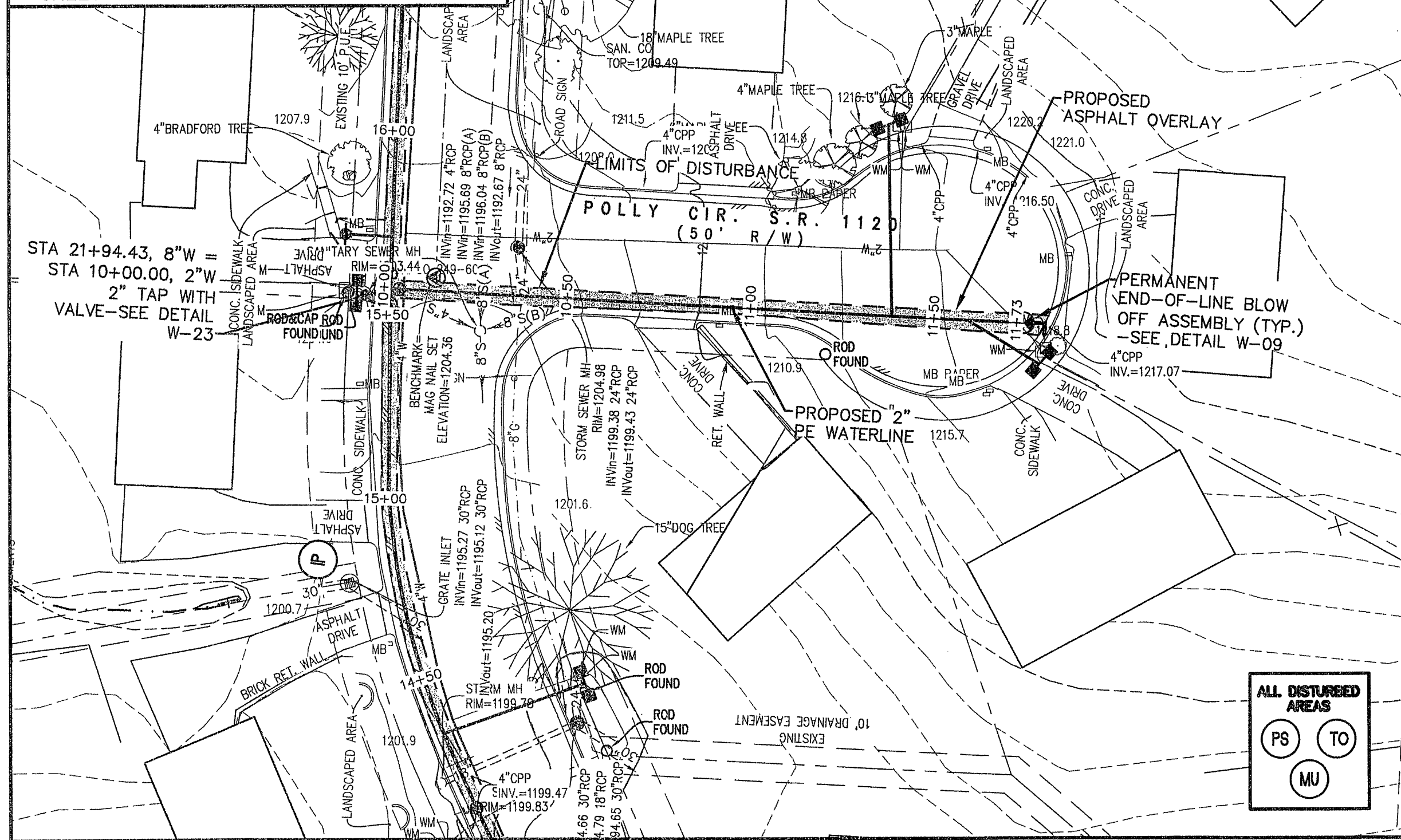
POLY CIRCLE PLAN SCALE: 1"=30'
