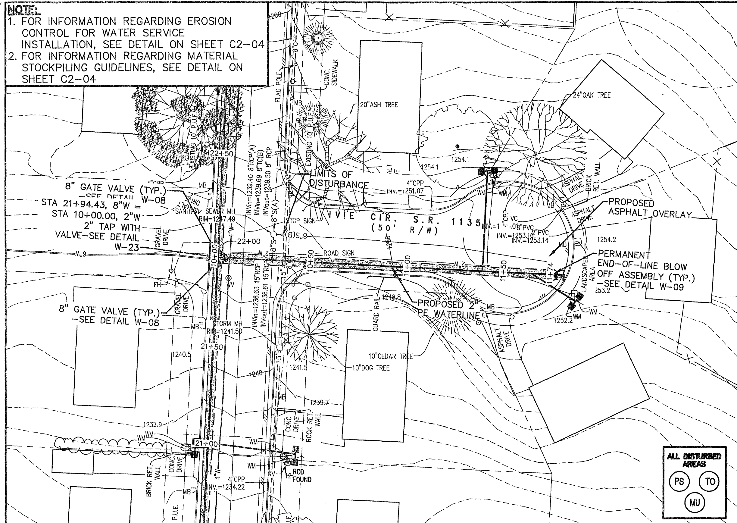
IVIE CIRCLE PLAN SCALE: 1"=30'
