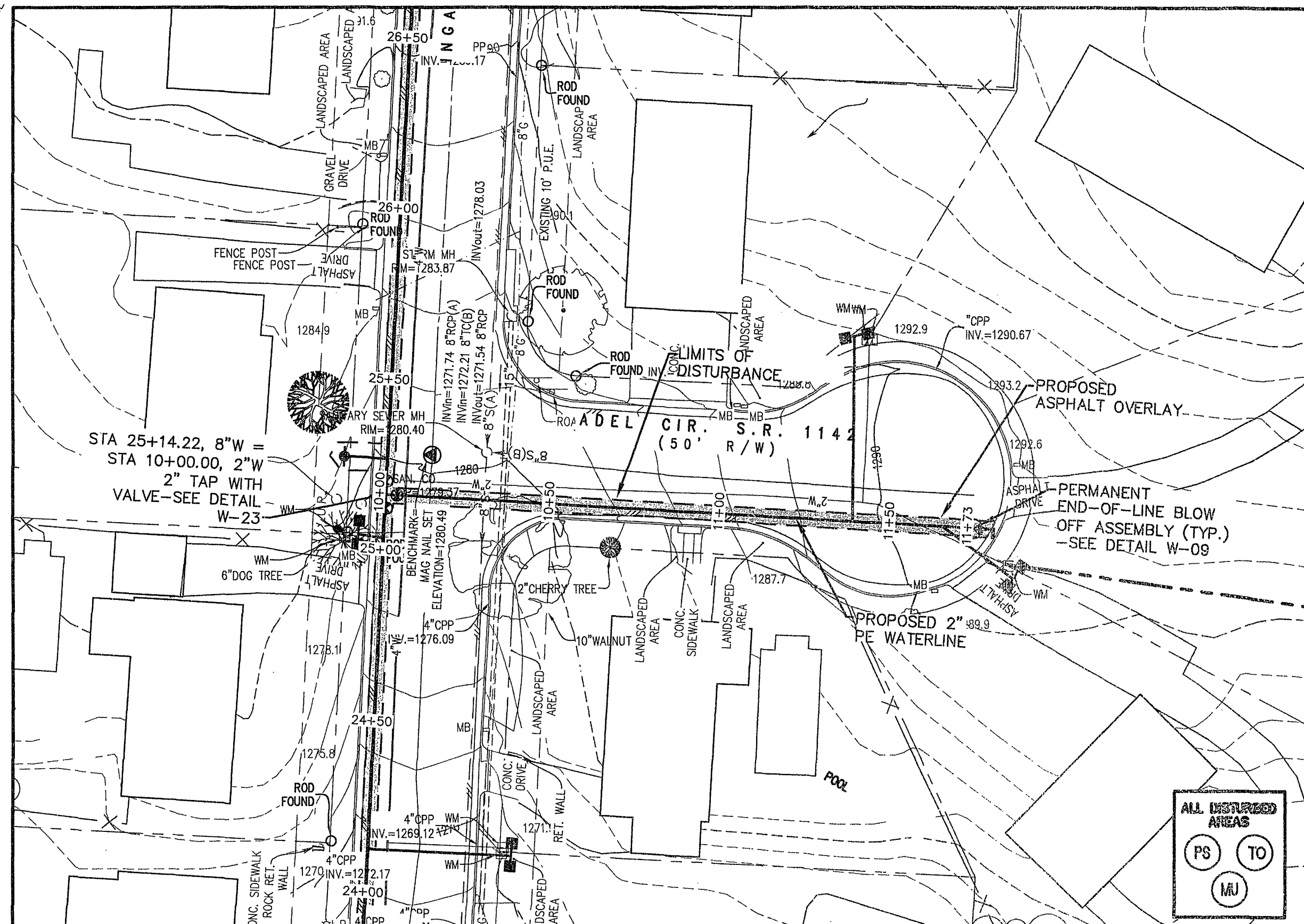
ADEL CIRCLE PLAN SCALE: 1"=30'
