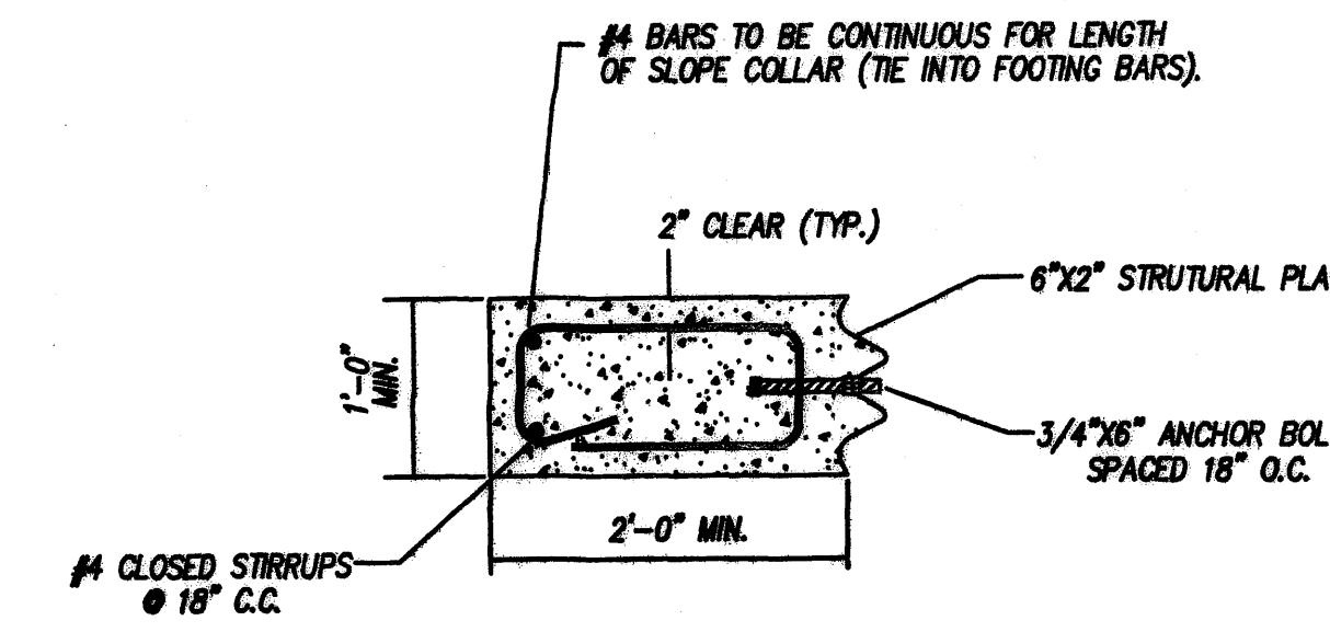
SECTION - A NO SCALE
