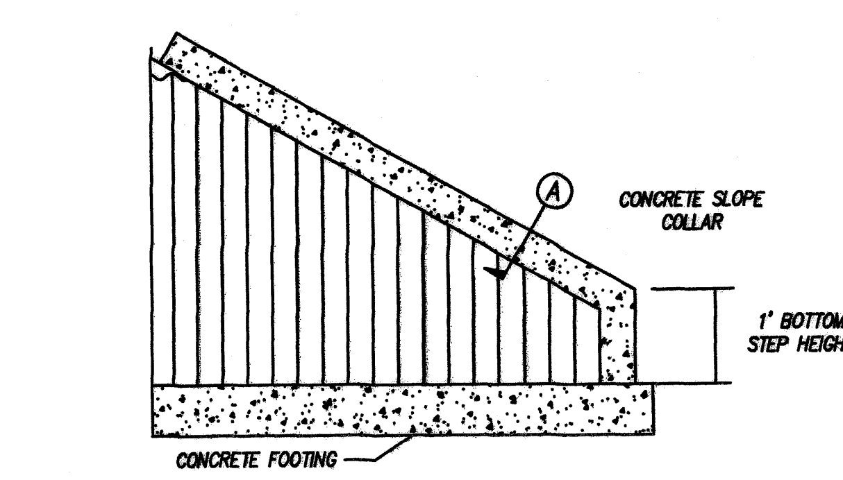
CONCRETE SLOPE COLLAR NO SCALE
