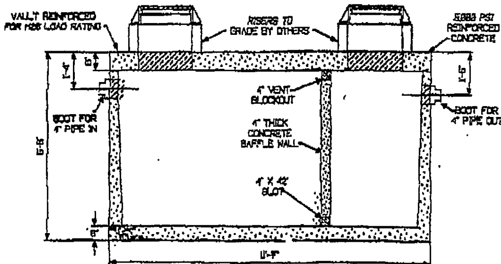
SECTION VIEW
