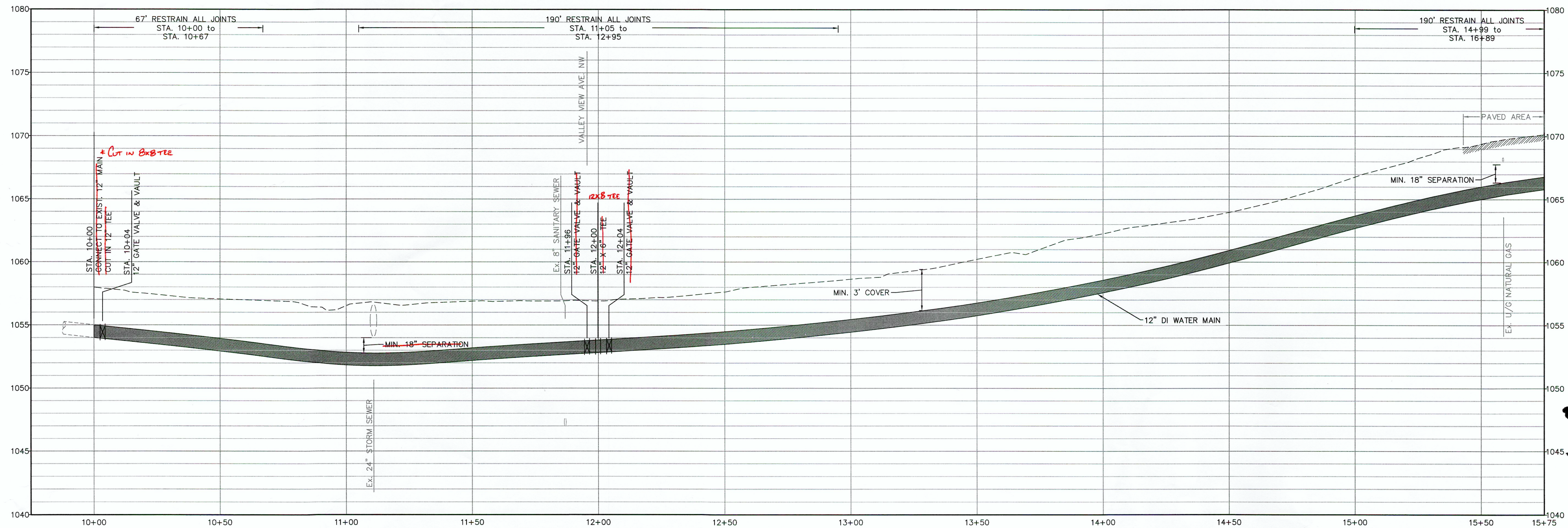
WATER MAIN PROFILE SCALE: H:1"=20' V:1"=4'
