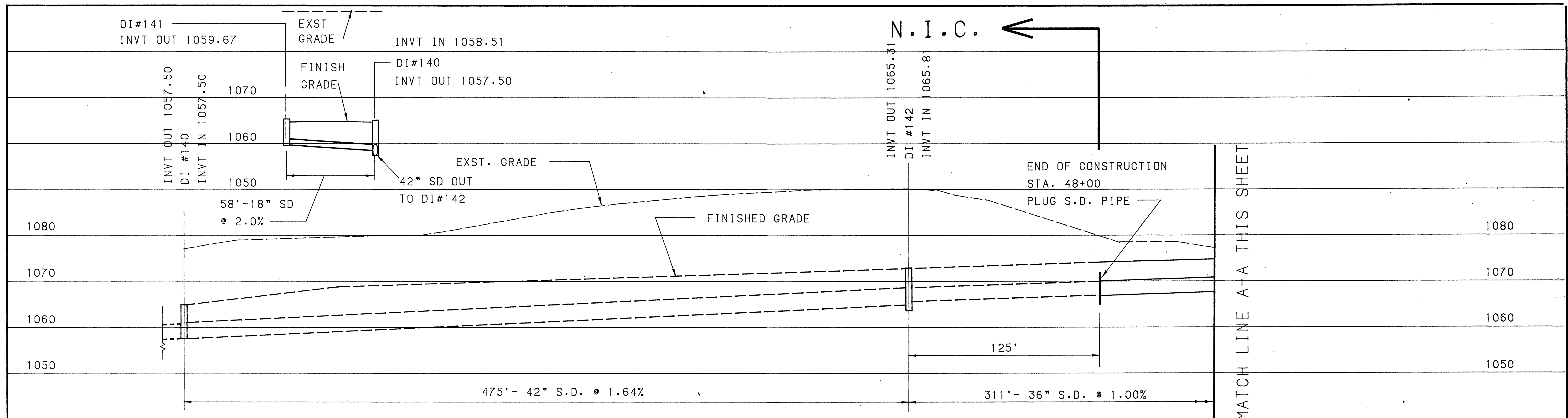
PROFILE- 42" AND 36" STORM DRAIN ROAD °A'
