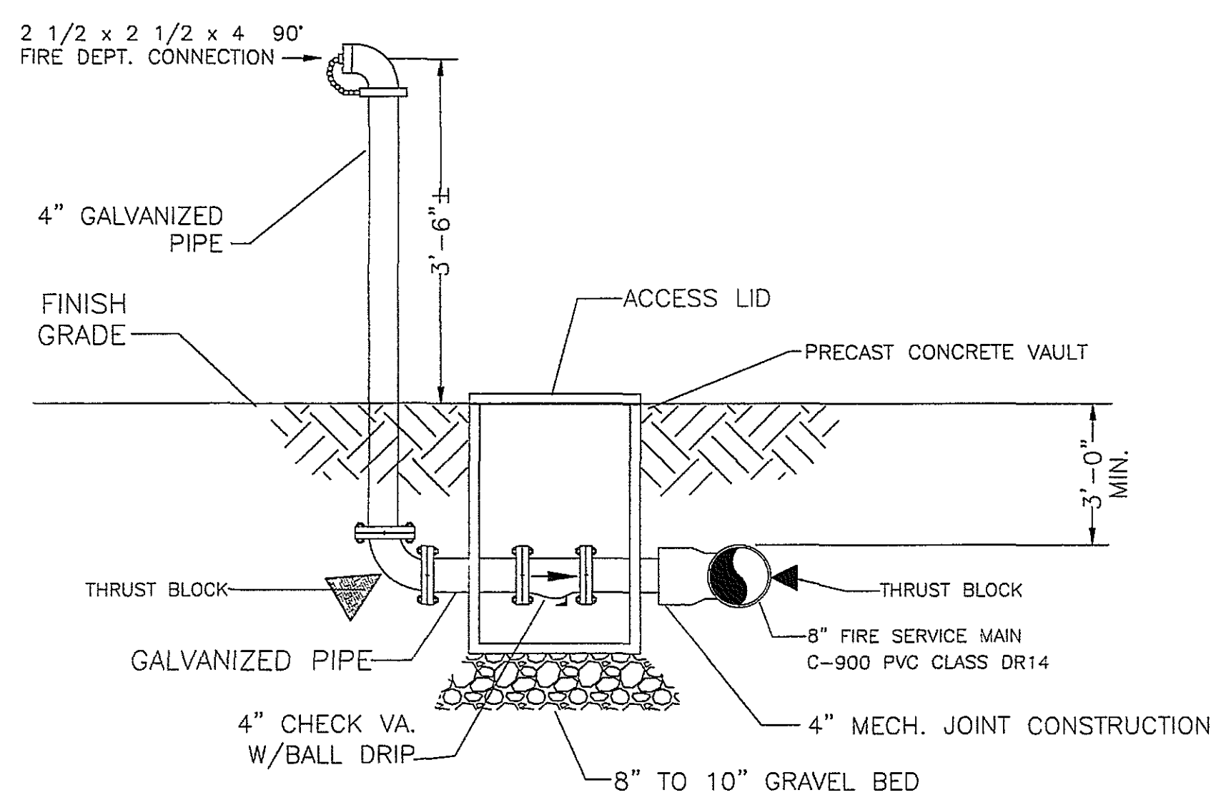
FIRE DEPARTMENT CONNECTION DETAIL NO SCALE
