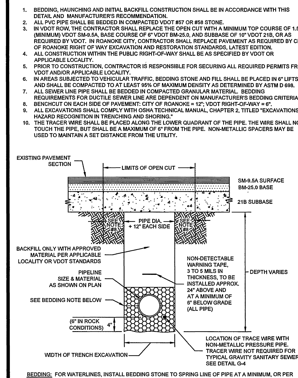
WESTERN VIRGINIA REGIONAL - CONSTRUCTION DETAIL 1 BEDDING AND BACKFILL UNDER PAVEMENT AND IN RIGHT-OF-WAY G- 01/01/12
