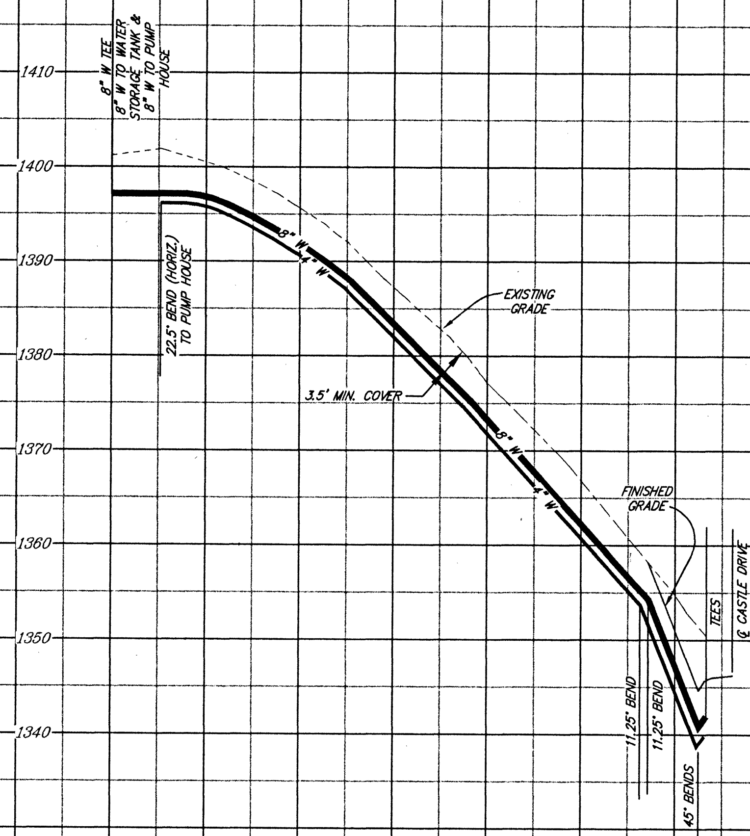
WATER PROFILE
