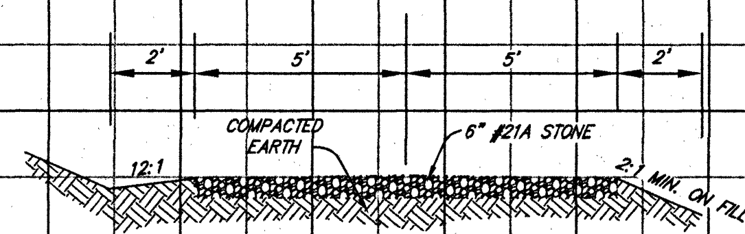
WELL LOT DRIVEWAY TYPICAL SECTION
