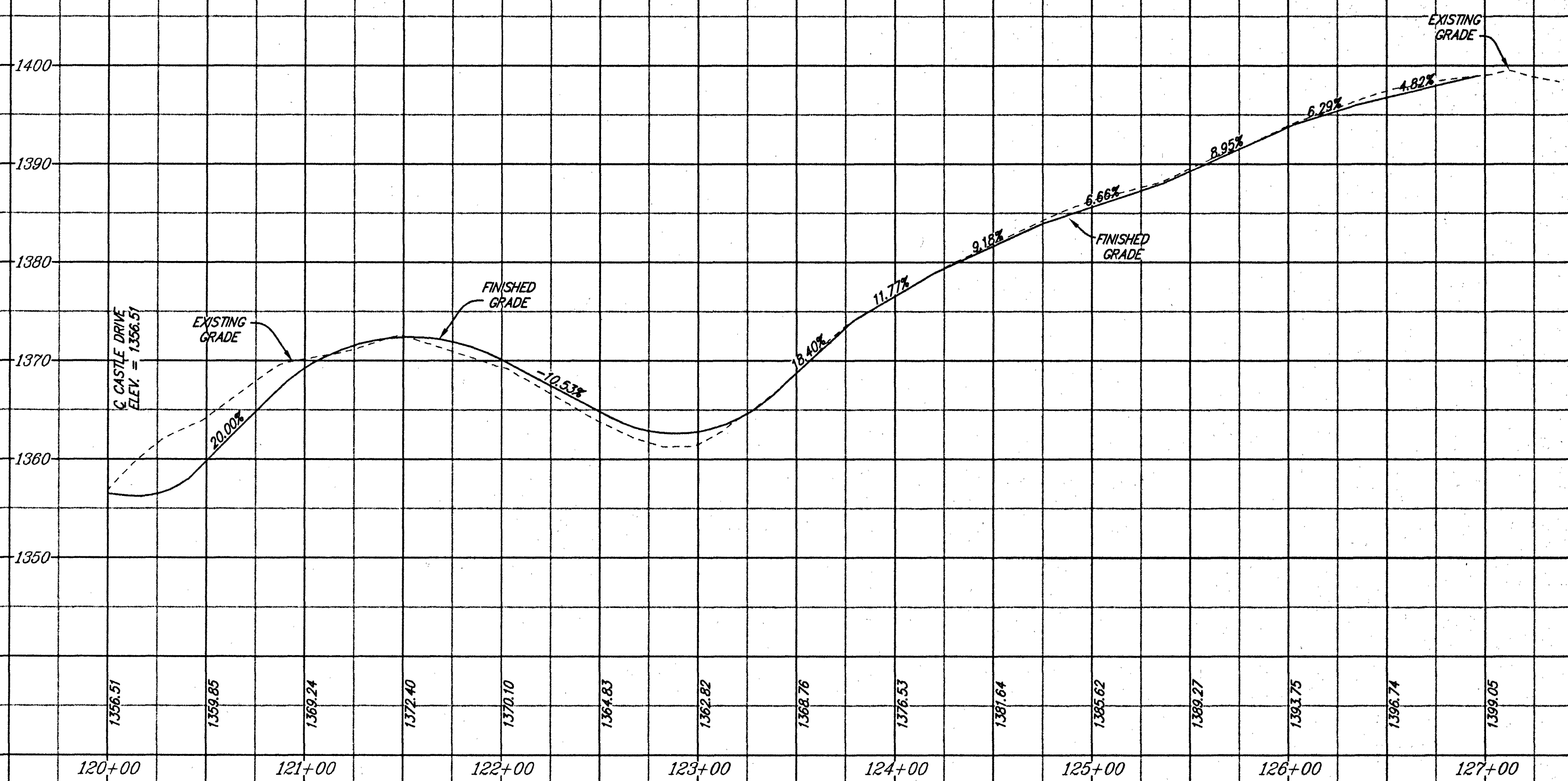
WELL LOT DRIVEWAY
