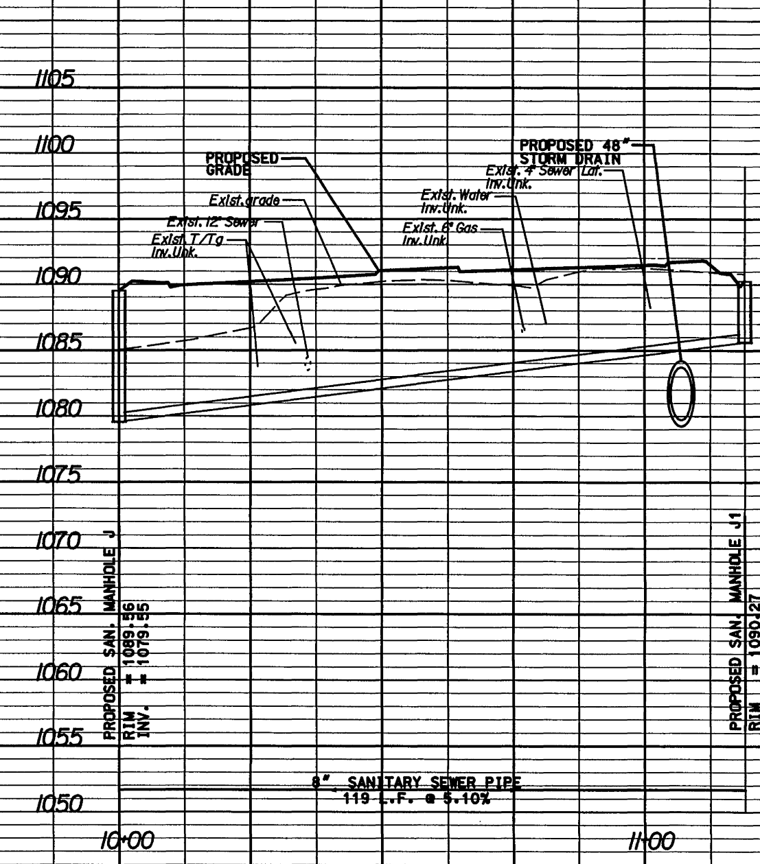
8" SANITARY SEWER PIPE, PLAN SHEETS 21(5) APPROX. STA. 31+99.57 RT. CONST. @ ON ROUTE 11 TO APPROX. STA. 32+02.62 LT. CONST. @ ON ROUTE 11
