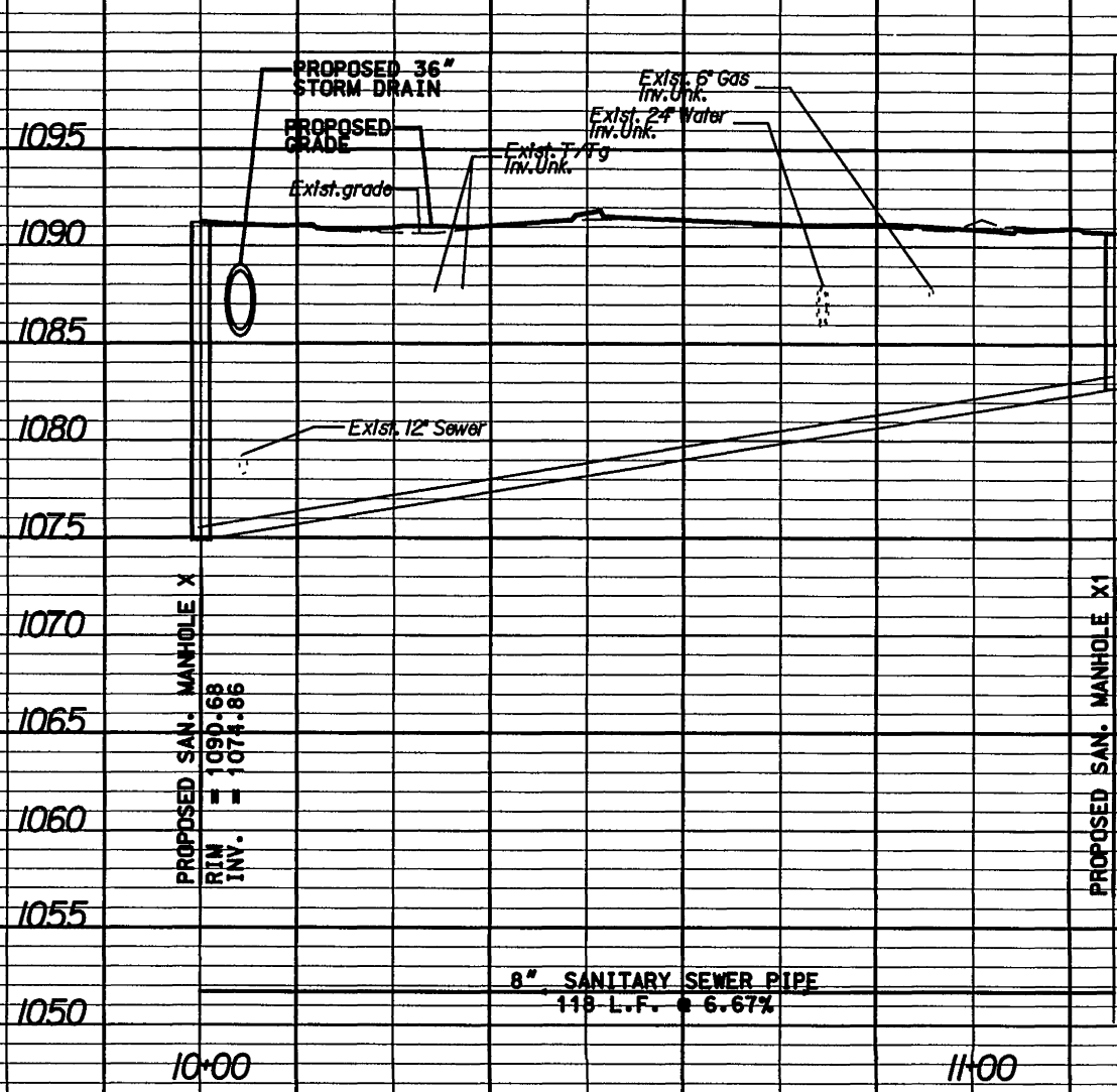
8" SANITARY SEWER PIPE, PLAN SHEETS 21(12) APPROX. STA. 83+82.54 RT. CONST. @ ON ROUTE 11 TO APPROX. STA. 83+86.59 LT. CONST. @ ON ROUTE 11
