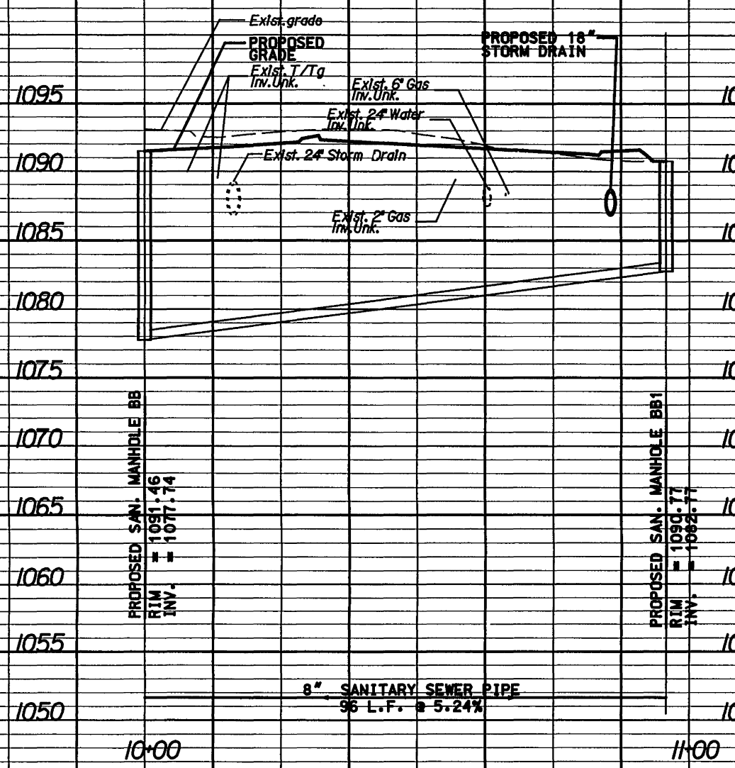
8" SANITARY SEWER PIPE, PLAN SHEETS 21(13) APPROX. STA. 93+98.36 RT. CONST. @ ON ROUTE 11 TO APPROX. STA. 93+99.59 LT. CONST. @ ON ROUTE 11
