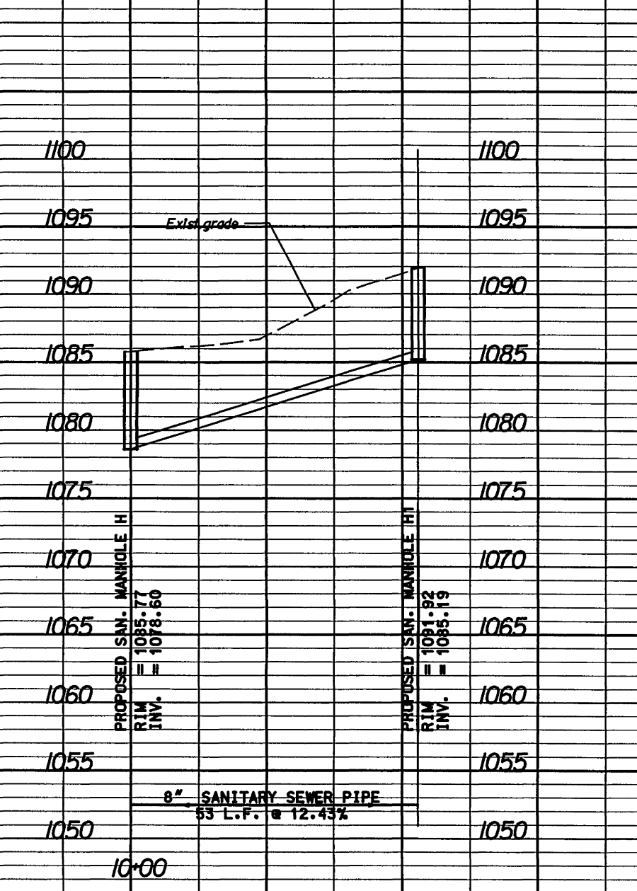
8" SANITARY SEWER PIPE, PLAN SHEETS 21(5) APPROX. STA. 11+23.38 LT. CONST. @ ON ROUTE 11 TO APPROX. STA. 11+57.9' LT. CONST. @ ON ROUTE 11
