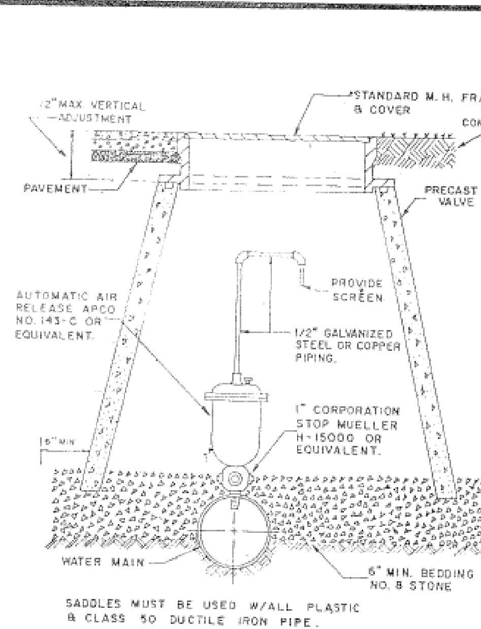
AUTOMATIC AIR RELEASE ASSEMBLY
