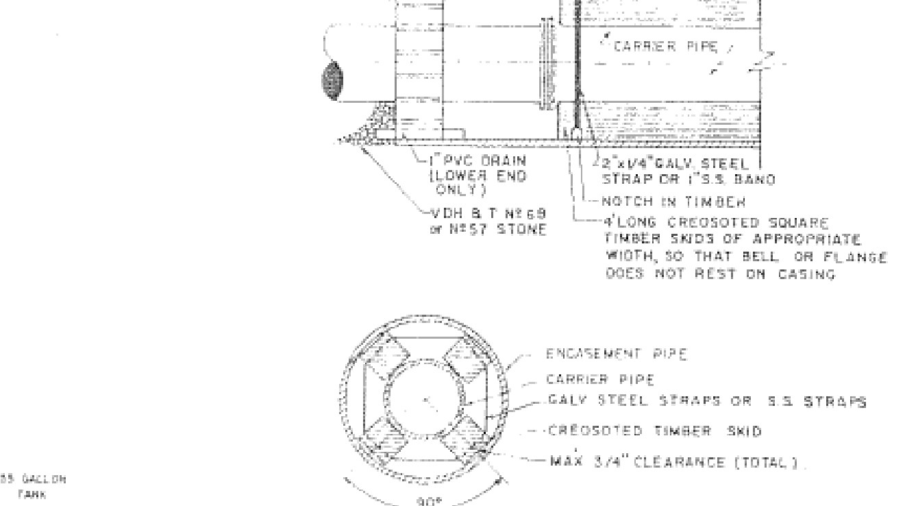
PIPE SUPPORT IN CASING PIPE
