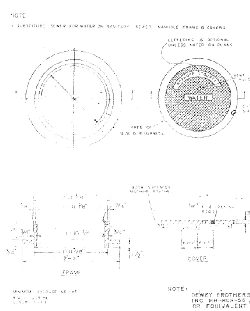
MANHOLE FRAME AND COVER
