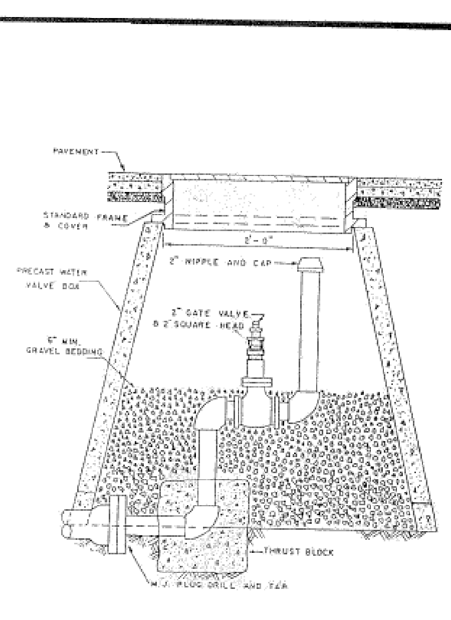
PERMANENT END OF LINE
