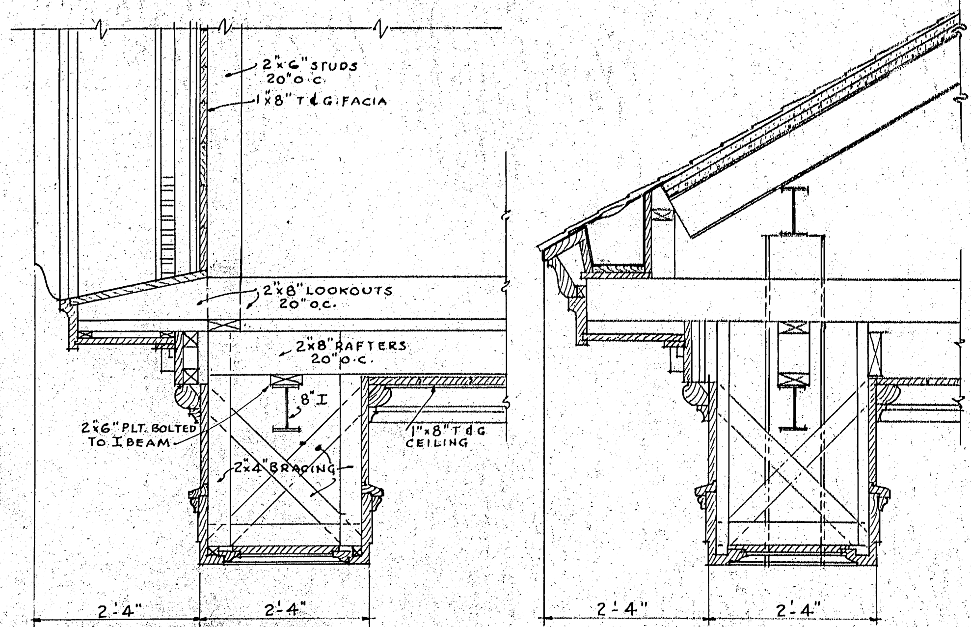
CORNICE SECTION AT SIDE OF PORTICO.
