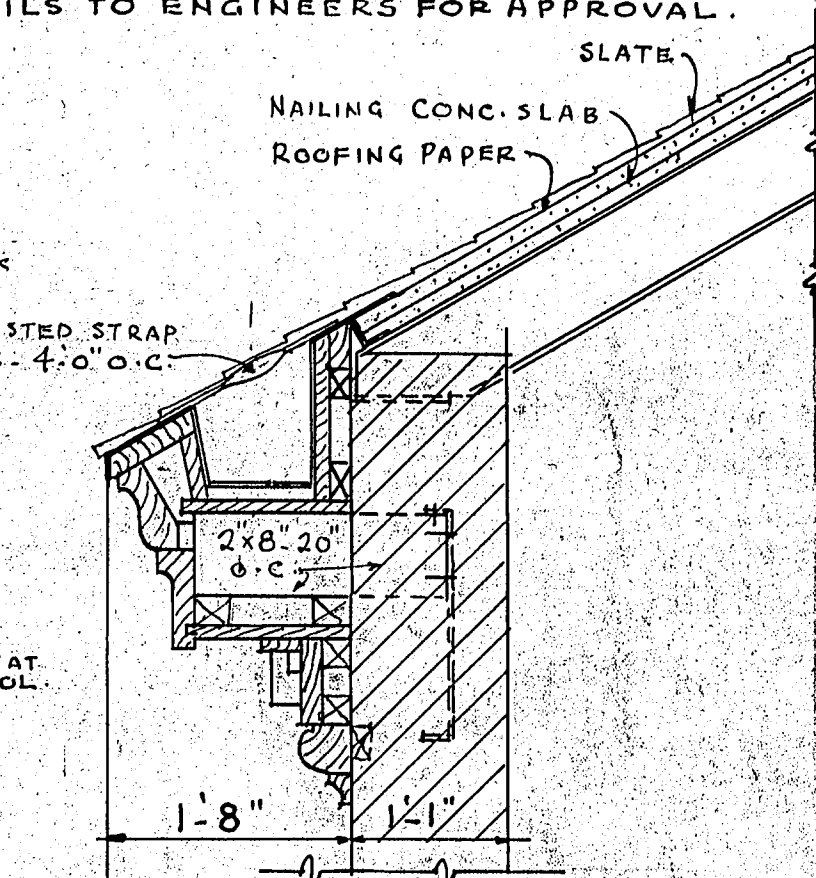
TYPICAL CORNICE DETAIL FOR FRONT BUILDING SCALE \frac{3}{4}"=1'-0" .
