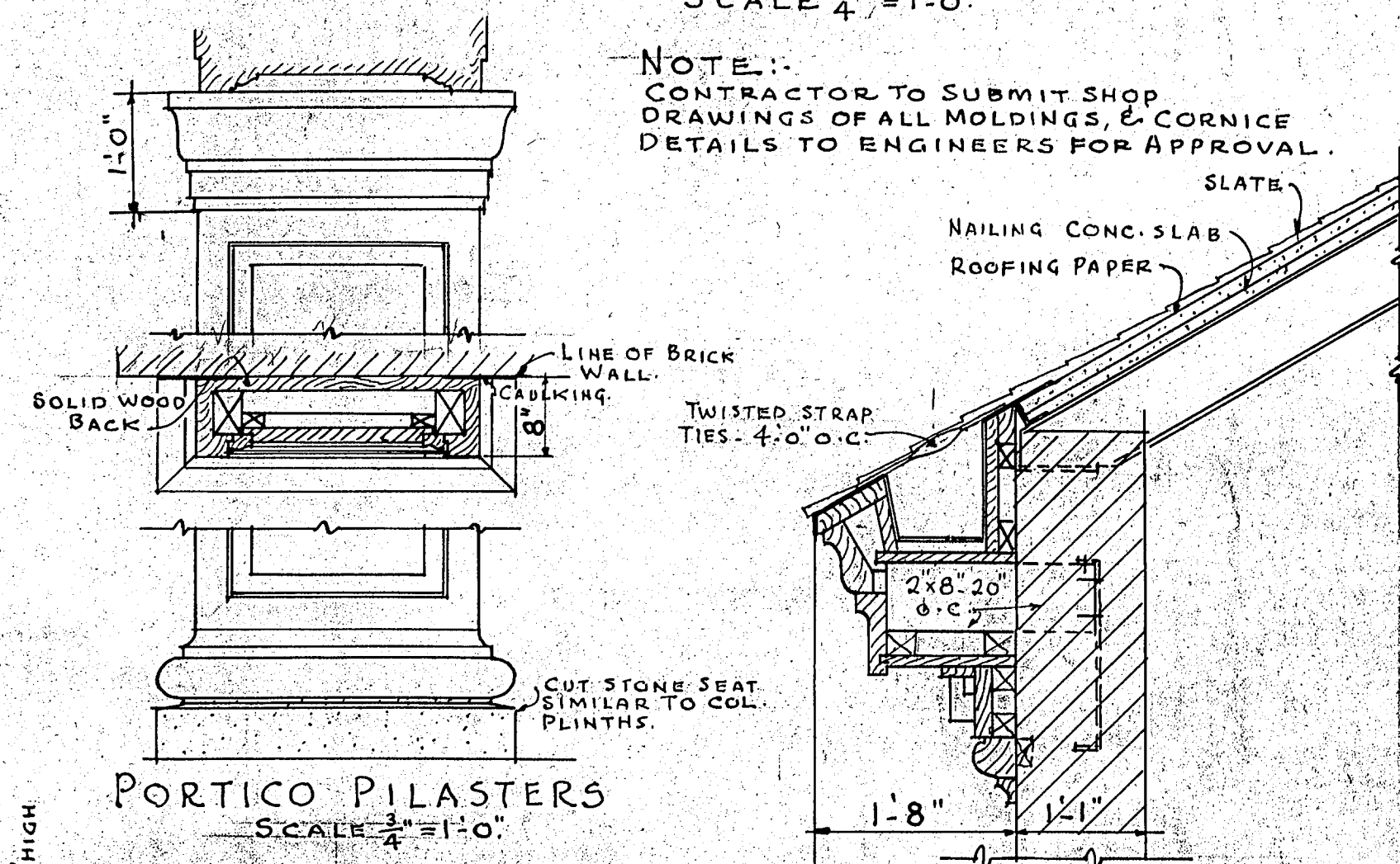
TYPICAL CORNICE DETAIL FOR FRONT BUILDING SCALE \frac{3}{4}"=1'-0" .
