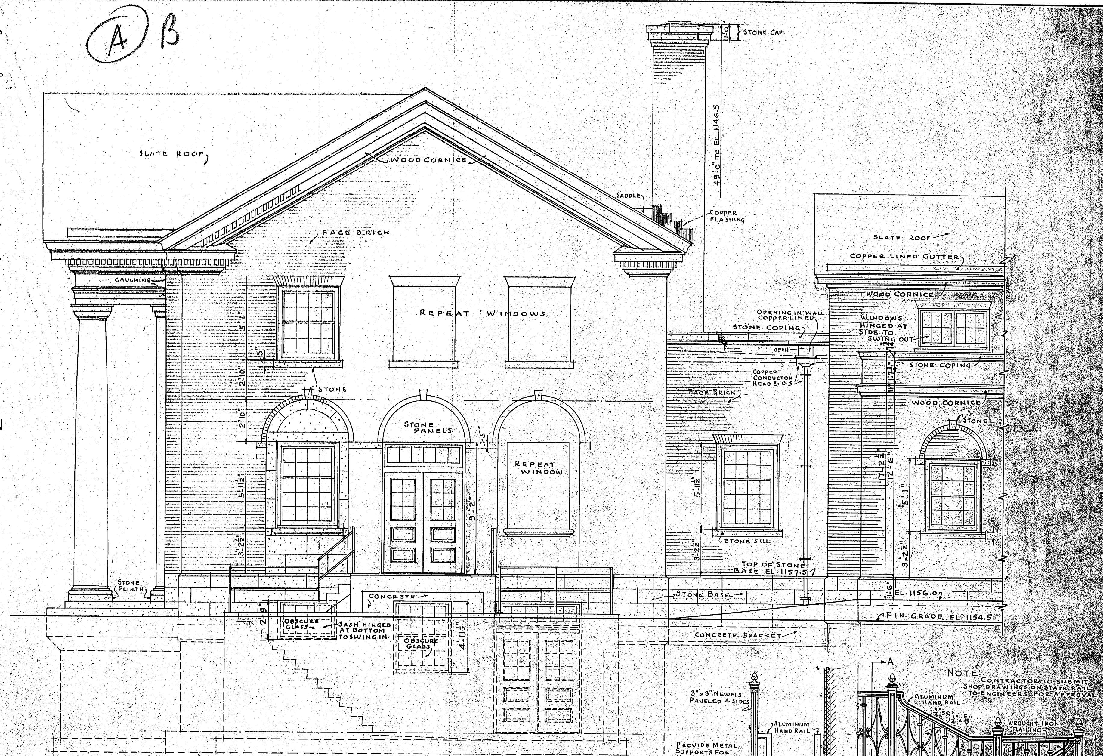
DETAIL OF SIDE ELEVATION LOOKING SOUTHWEST. SCALE \frac{1}{4}" = 1'-0"
