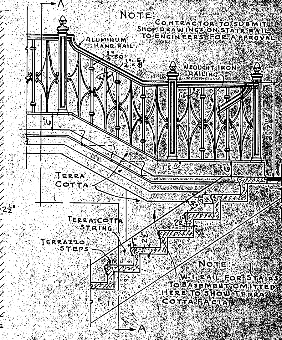
DETAIL OF STAIRS IN ENTRANCE HALL SCALE \frac{1}{2}" = 1'-0"
