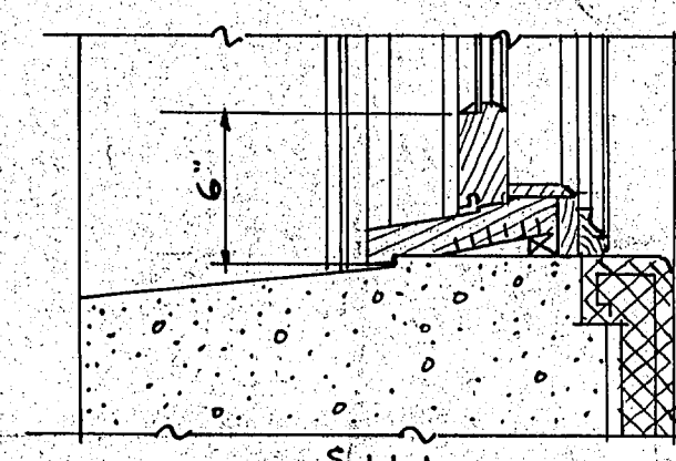
D.H. WINDOW IN BASEMENT.
