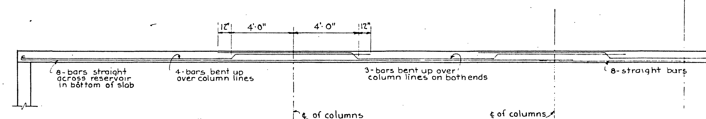
SECTION SHOWING BENDING & ARRANGEMENT OF BARS IN BELT B
