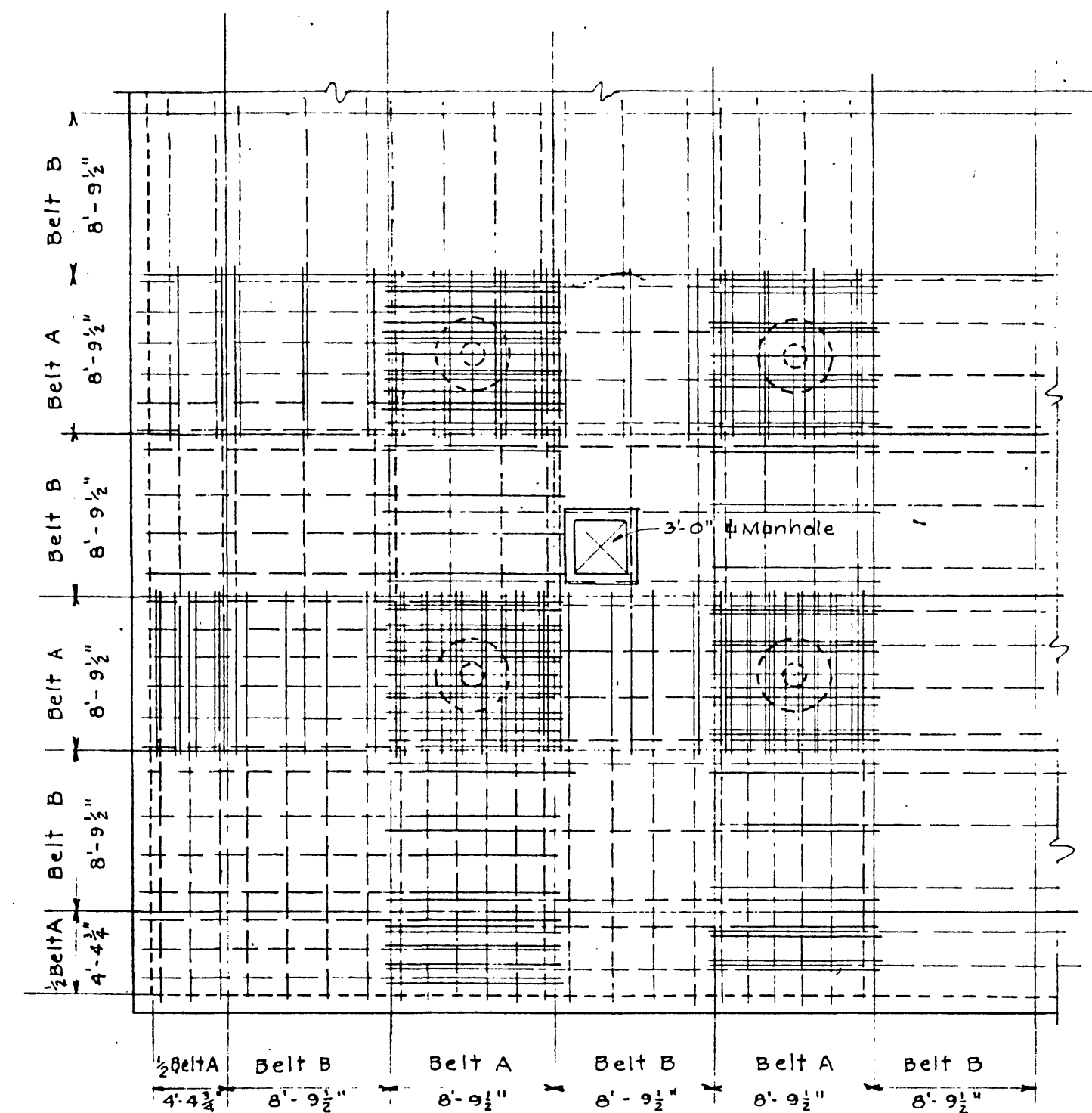
PLAN OF TYPICAL ARRANGEMENT OF FLAT SLAB BARS SCALE \frac{1}{8} " = 1'-0"
