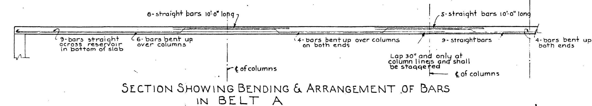
TYPICAL SECTION THRU COLUMNS (BELT A) SCALE \frac{1}{4} " = 1'-0"
