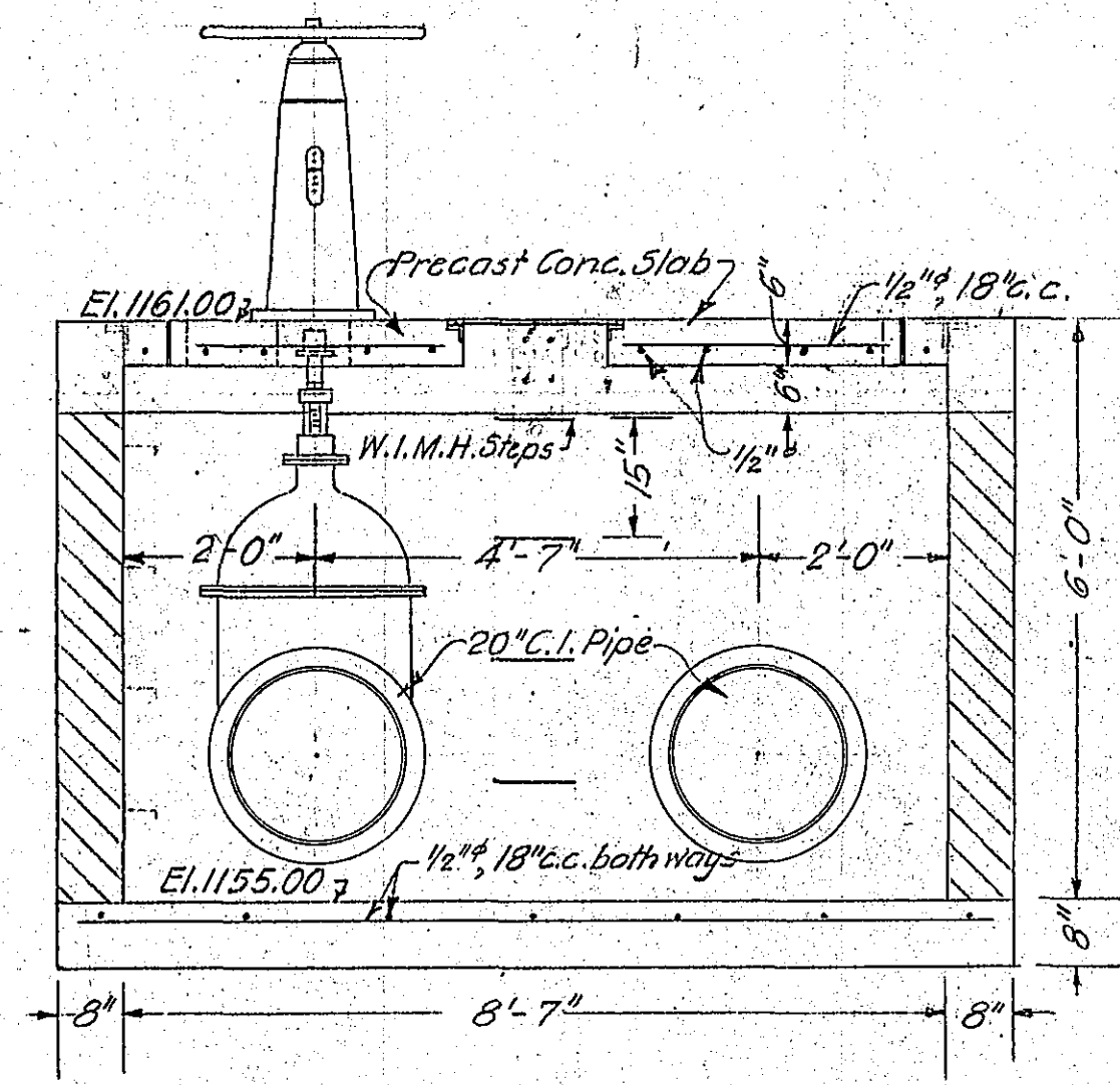
SECTION P-P
