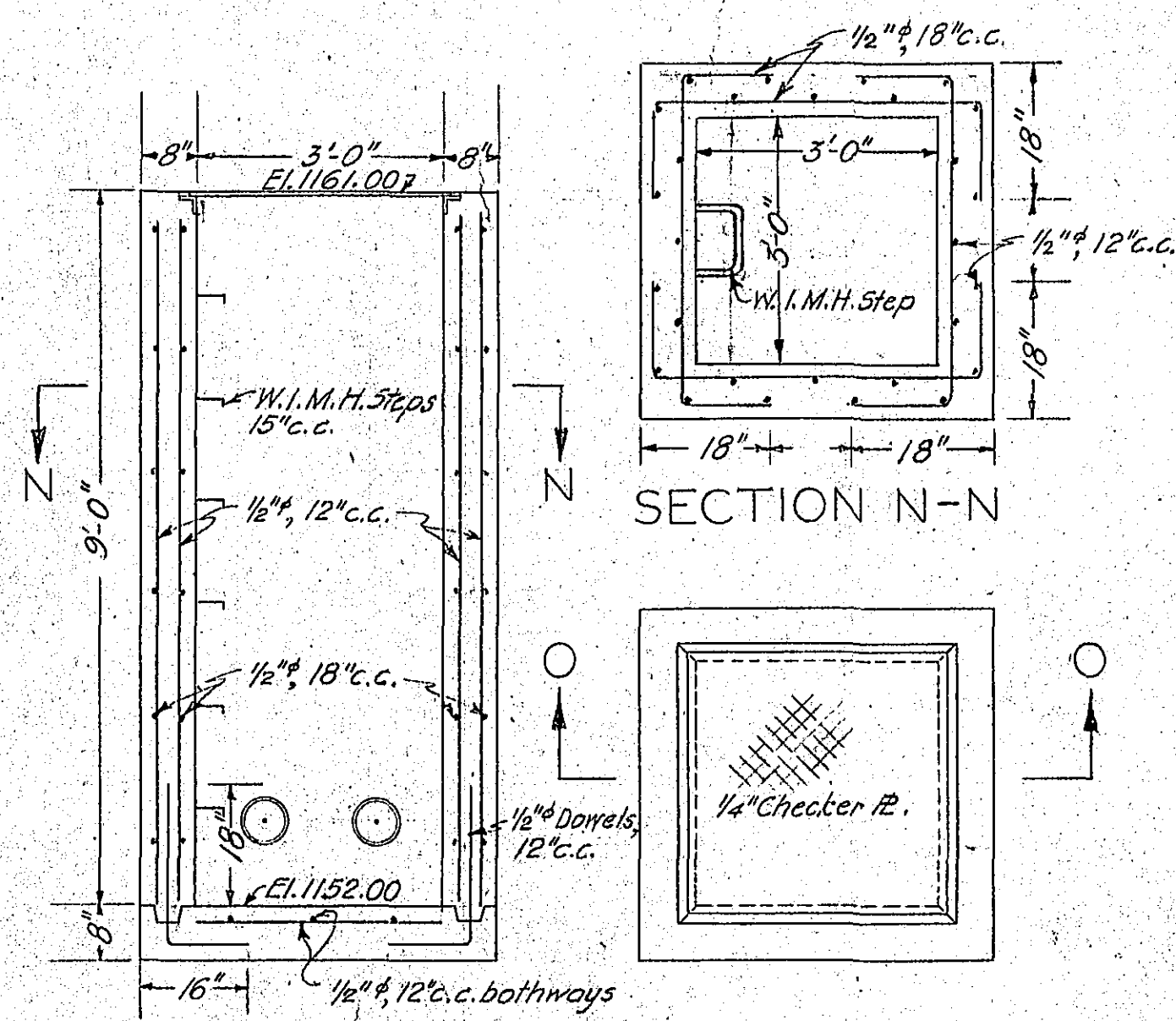
SECTION O-O DRAIN MANHOLE DETAILS SCALE: 1" = 2'-0"
