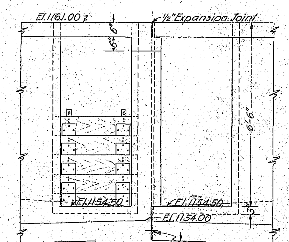
SECTION U-U STOP LOG GROOVE DETAILS SCALE: 1" = 2'-0"
