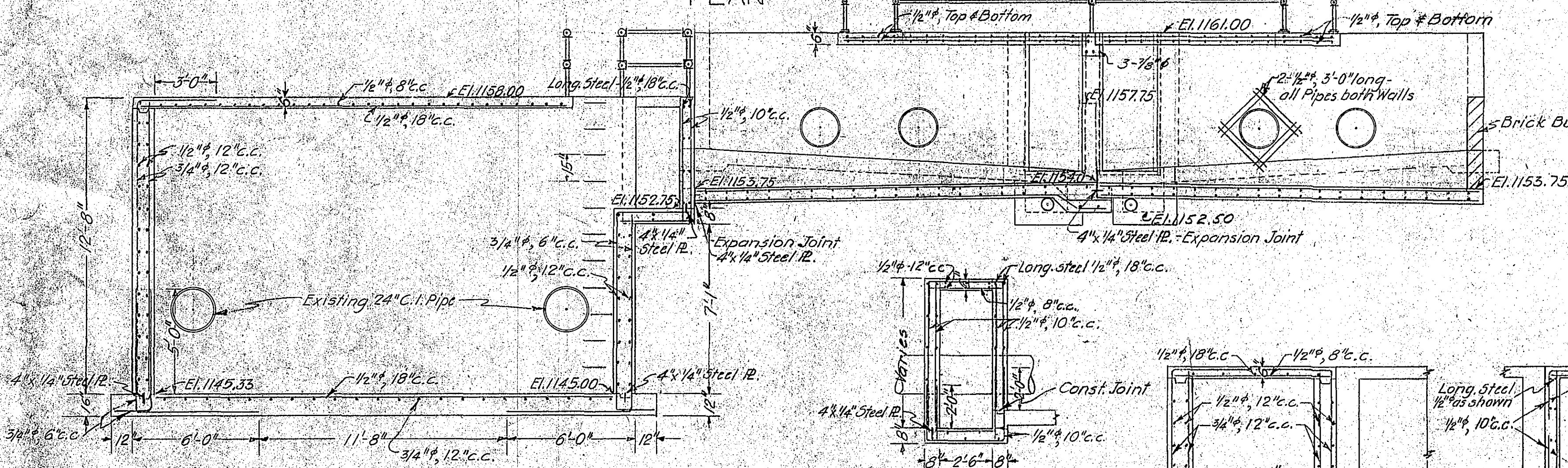
SECTION Q-Q
