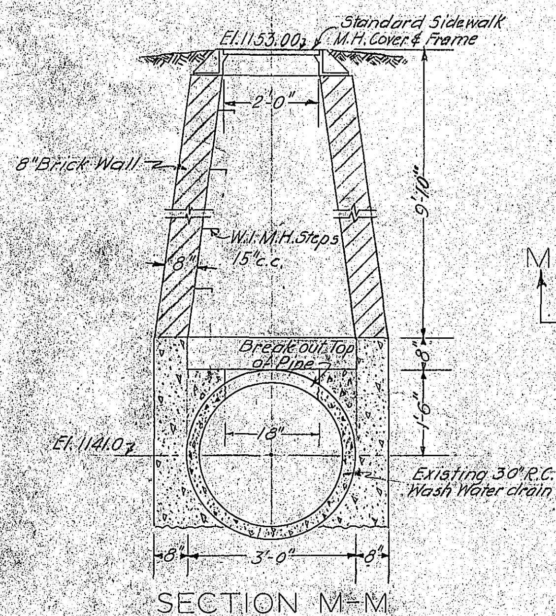
SECTION M-M DETAILS OF NEW MANHOLE OF 30" DRAIN SCALE: 1" = 2'-0"
