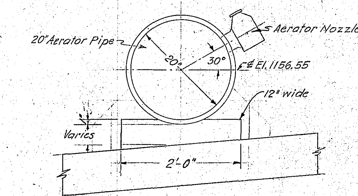
DETAIL OF AERATOR PIPE SUPPORT SCALE: 1" = 1'-0"
