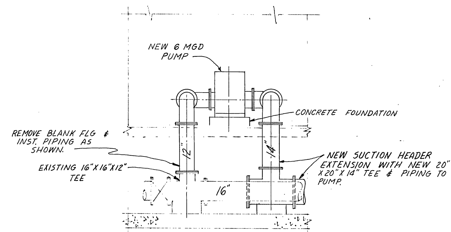
SECTION: B-B SCALE: \frac{1}{4}" = 1'-0"
