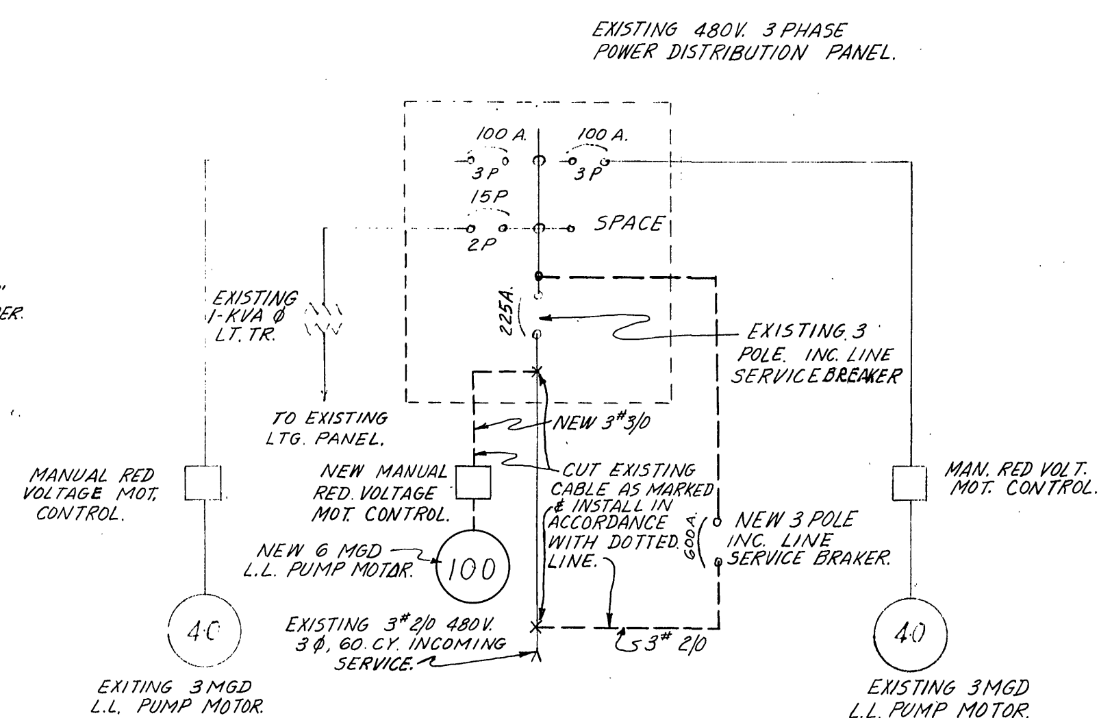
ONE LINE WIRING DIAGRAM
