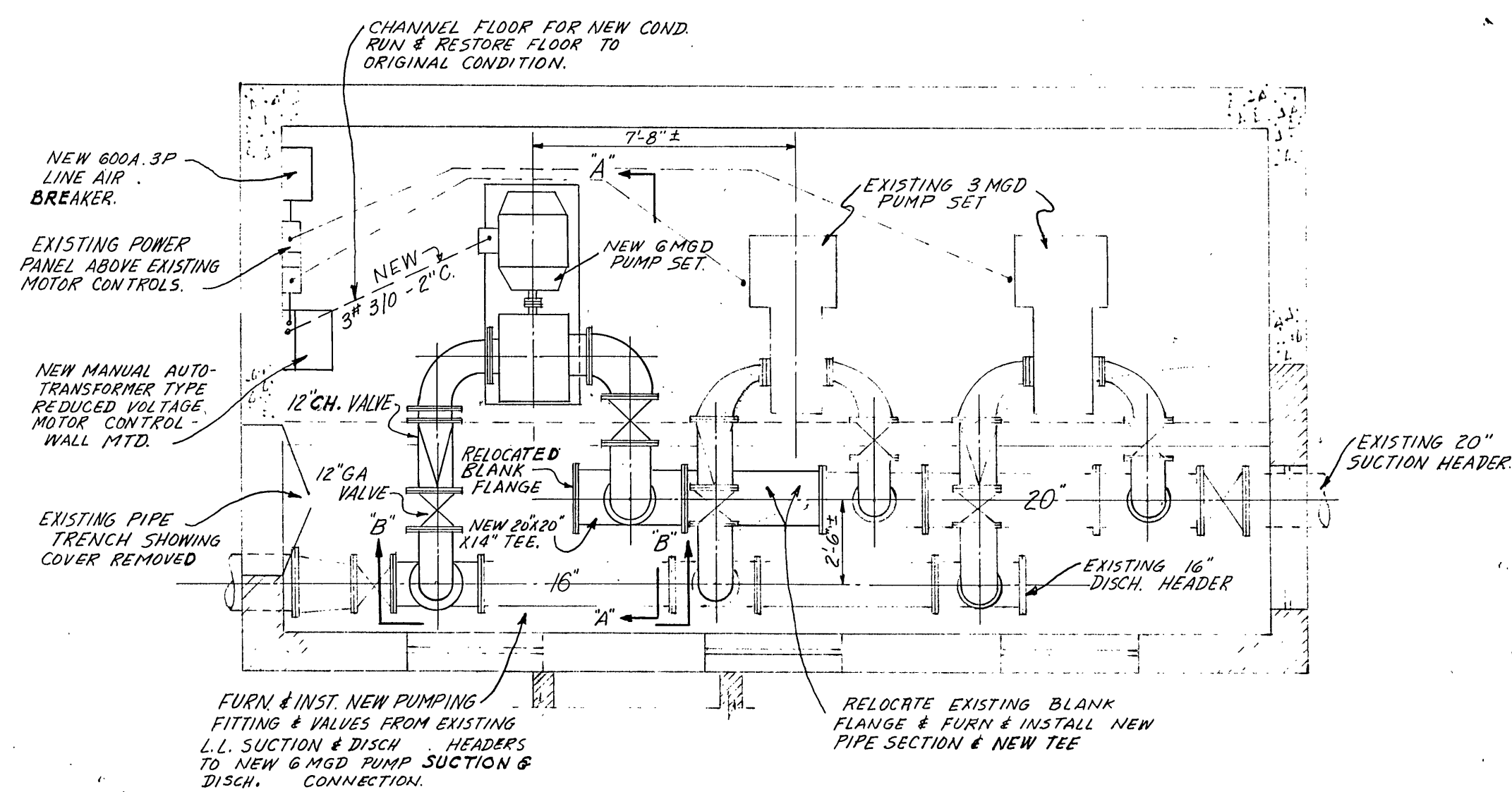
PLAN OF LOW LIFT PUMP HOUSE SCALE: \frac{1}{4}" = 1'-0"
