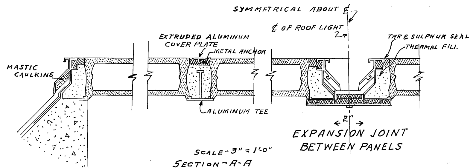
DETAIL OF ROOF LIGHTS OVER FILTER OPERATING GALLERY
