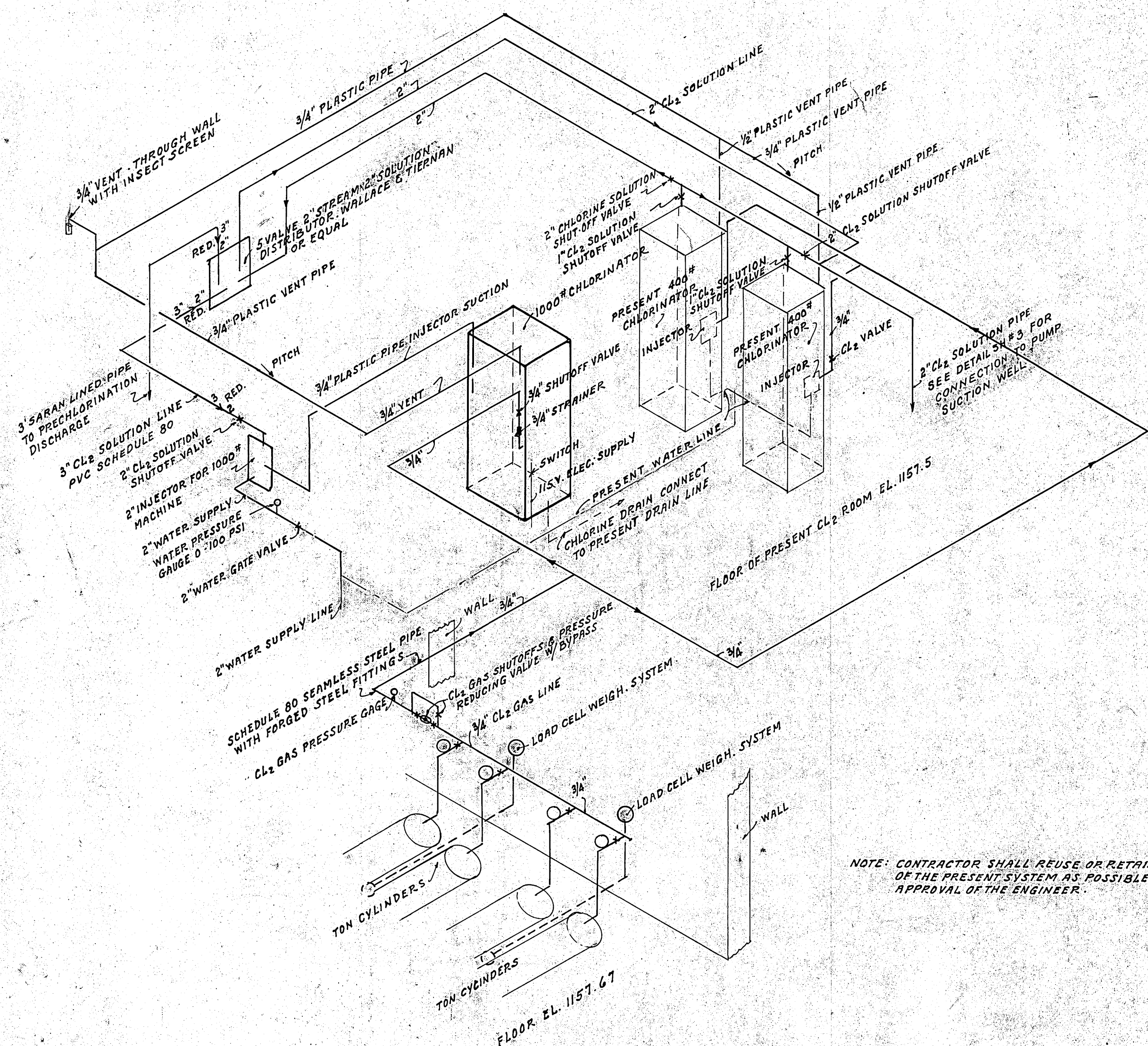
SCHEMATIC CHLORINE SYSTEM NO SCALE
