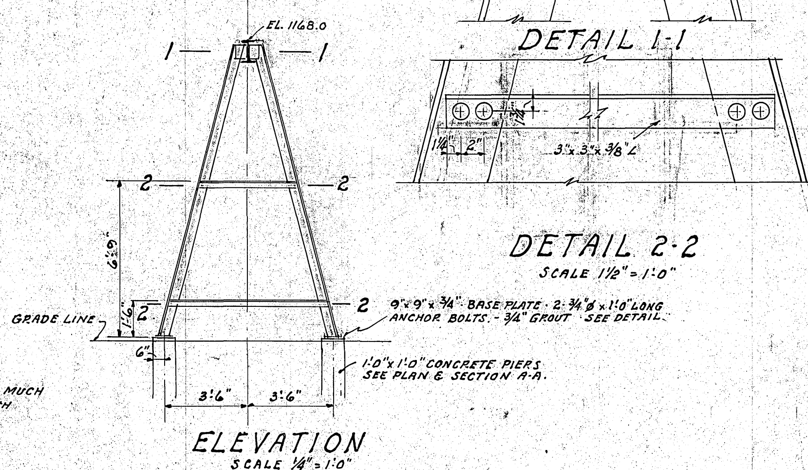
DETAILS OF "A" FRAME
