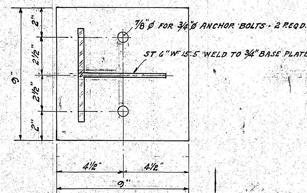
BASE PLATE DETAIL SCALE 3" = 1'-0"
