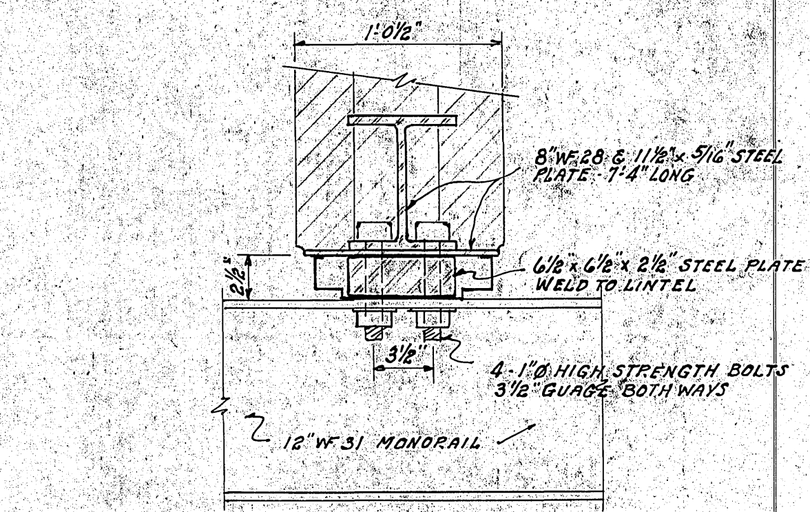
DETAIL OF MONORAIL AT DOOR SCALE 1 1/2" = 1'-0"
