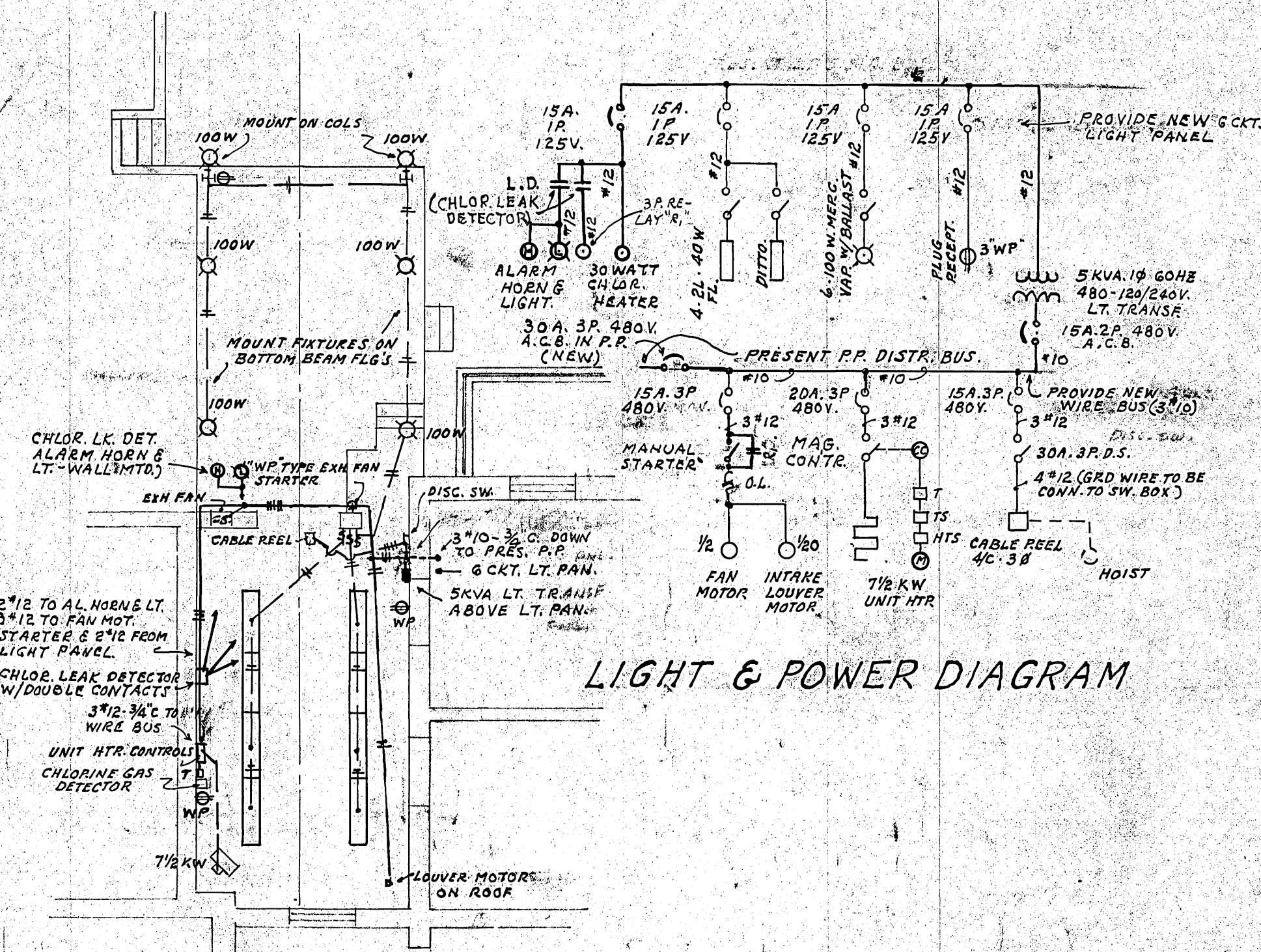
PLAN SCALE 1/8" = 1'-0" ELECTRICAL LAYOUT
