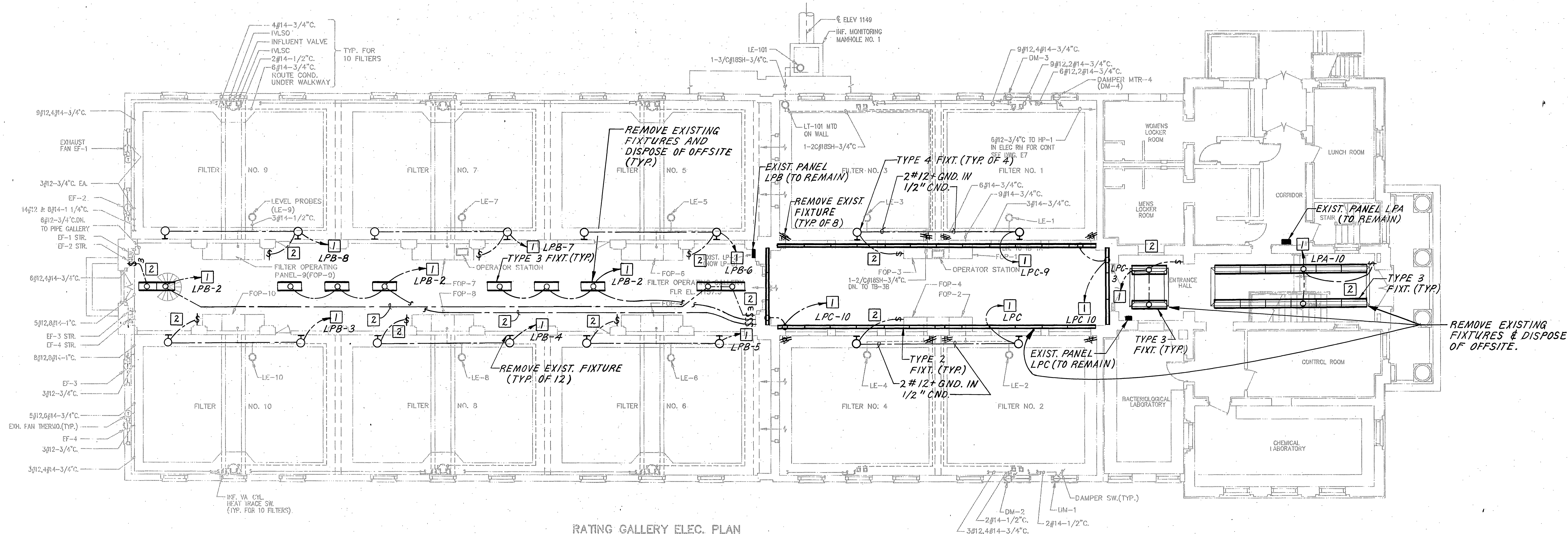
RATING GALLERY ELEC. PLAN SCALE OF DRAWING 1/8" = 1'-0" 0 2 4 6 8 10 12 14 16
