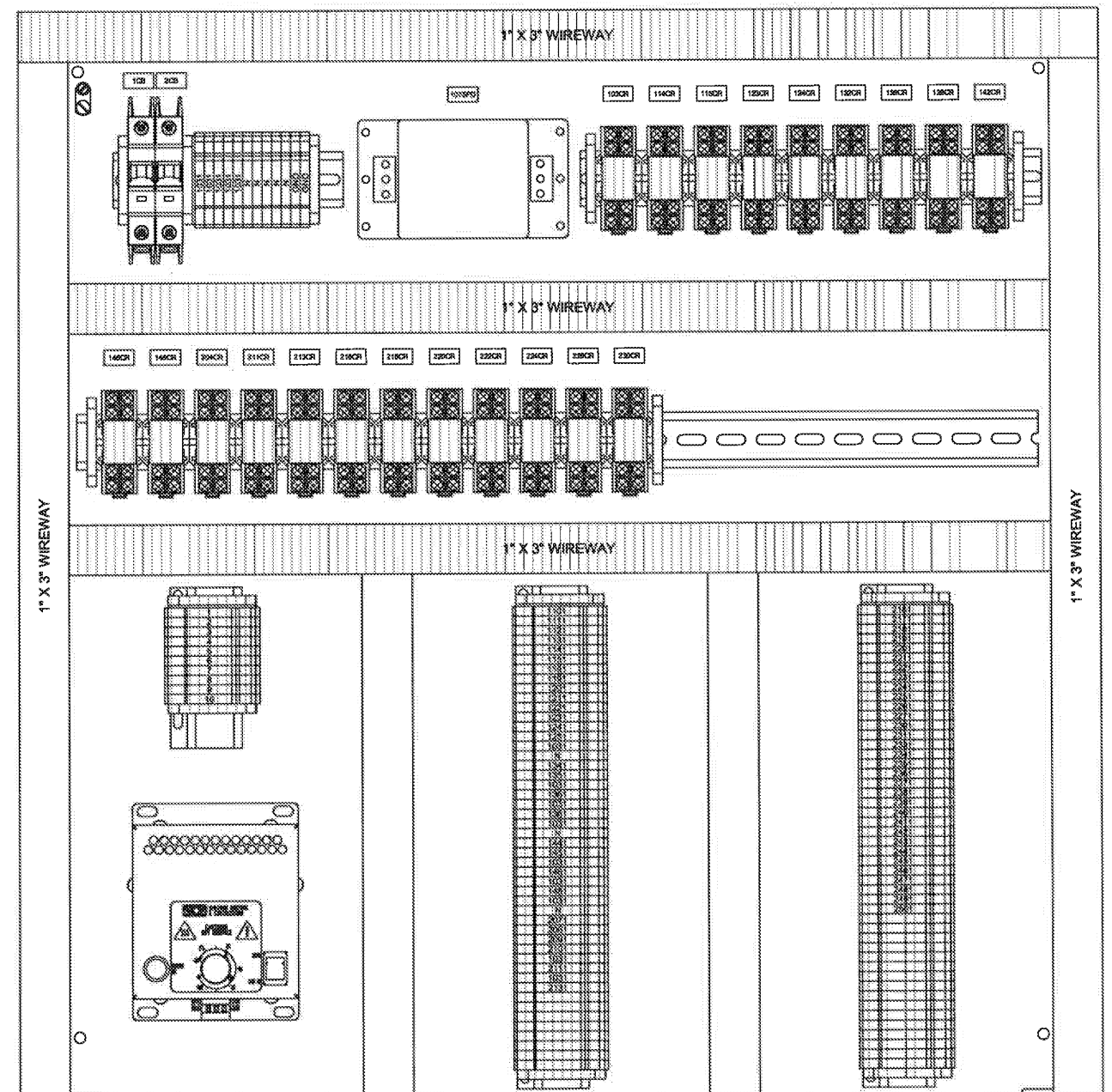
SUB-PANEL LAYOUT
