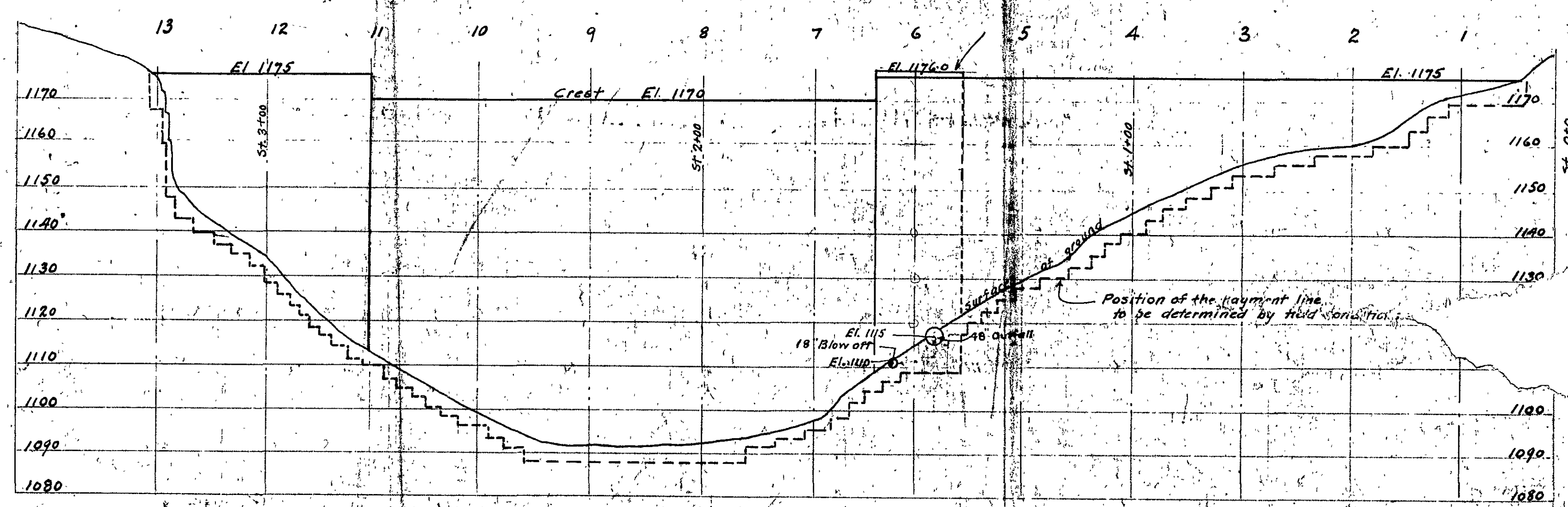
PROFILE OF DAM ON CENTER LINE
