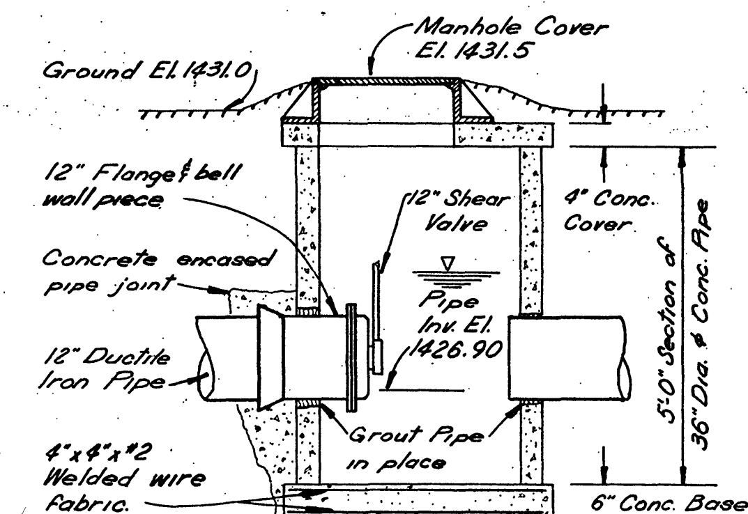
Section Through Manhole BYPASS CULVERT MANHOLE DETAILS Scale: 1/2"=1'-0"
