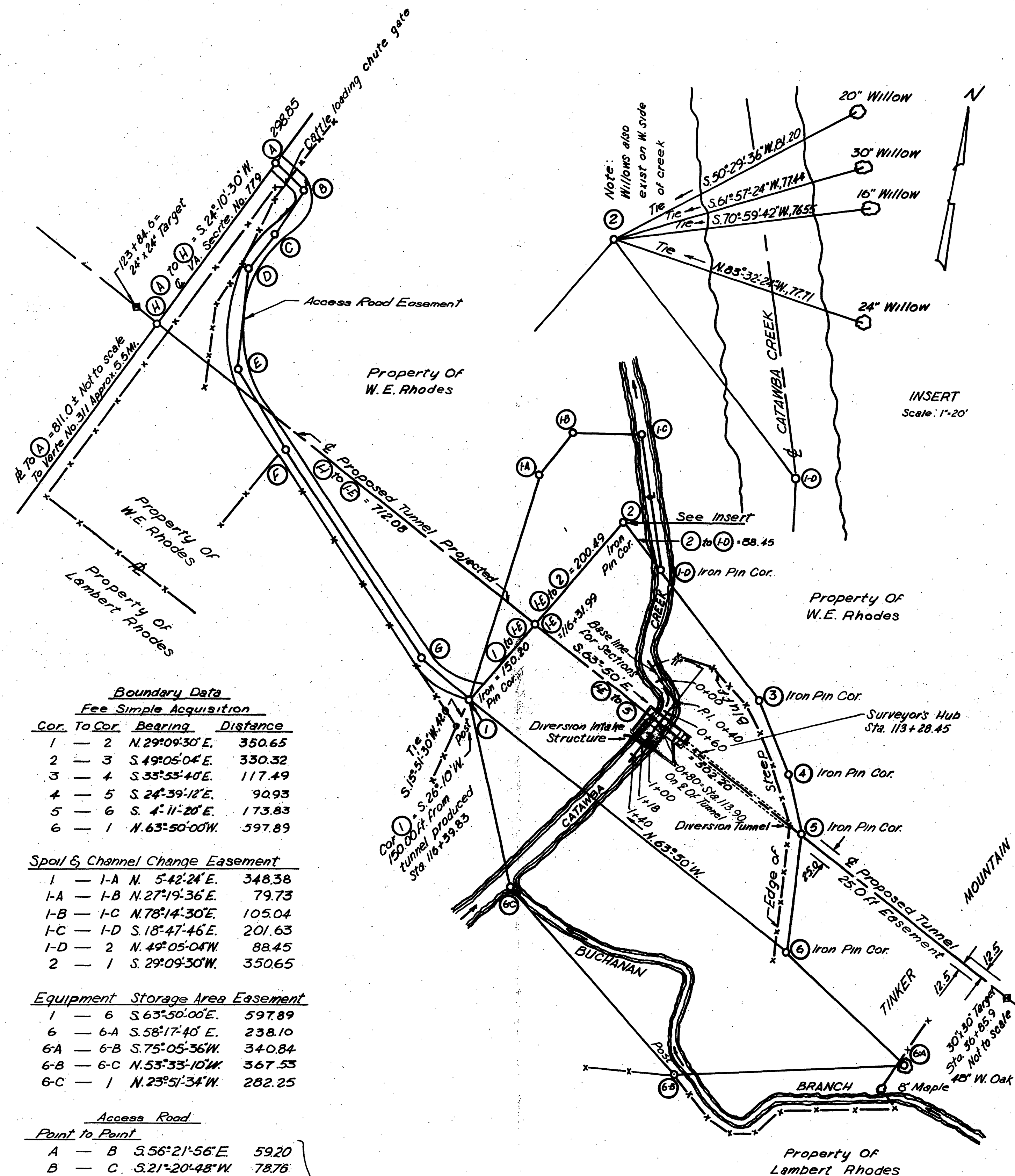
PLAT OF SURVEY AND PLAN Scale: 1"=100'
