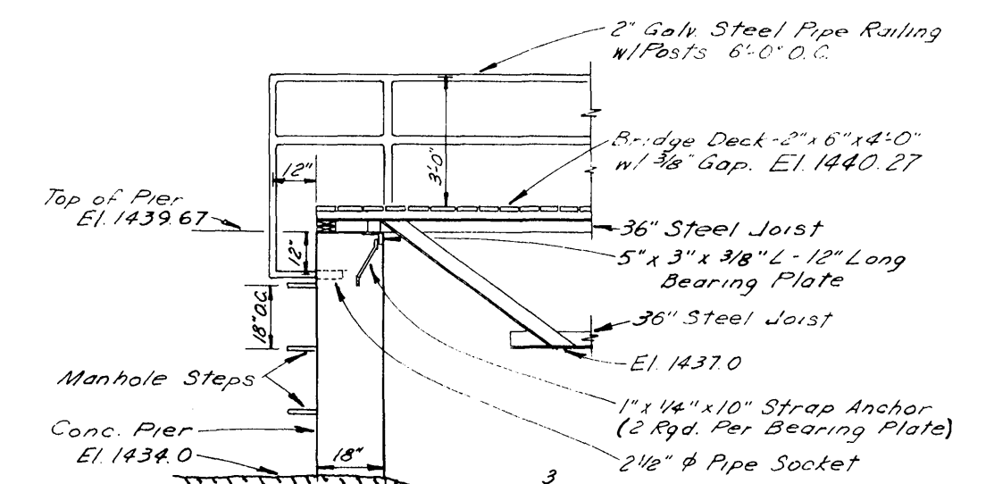
DETAIL PIER #3 Scale: 1/4"=1'-0"
