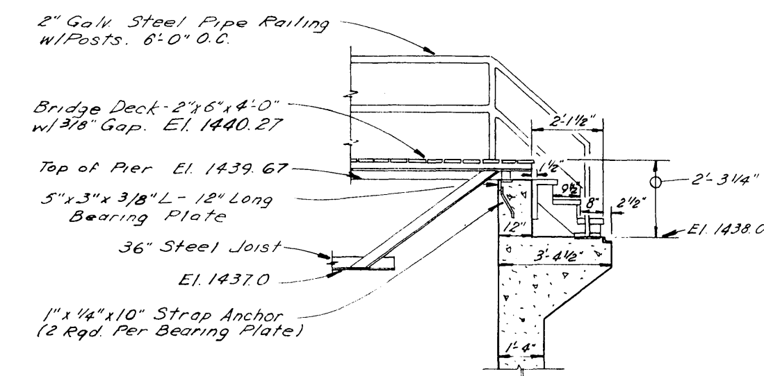
DETAIL PIER #1 Scale: 1/4"=1'-0"
