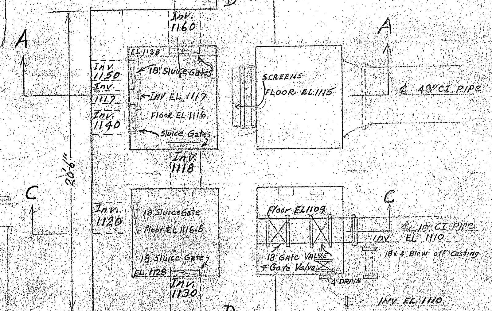
PLAN BELOW EL. 1170
