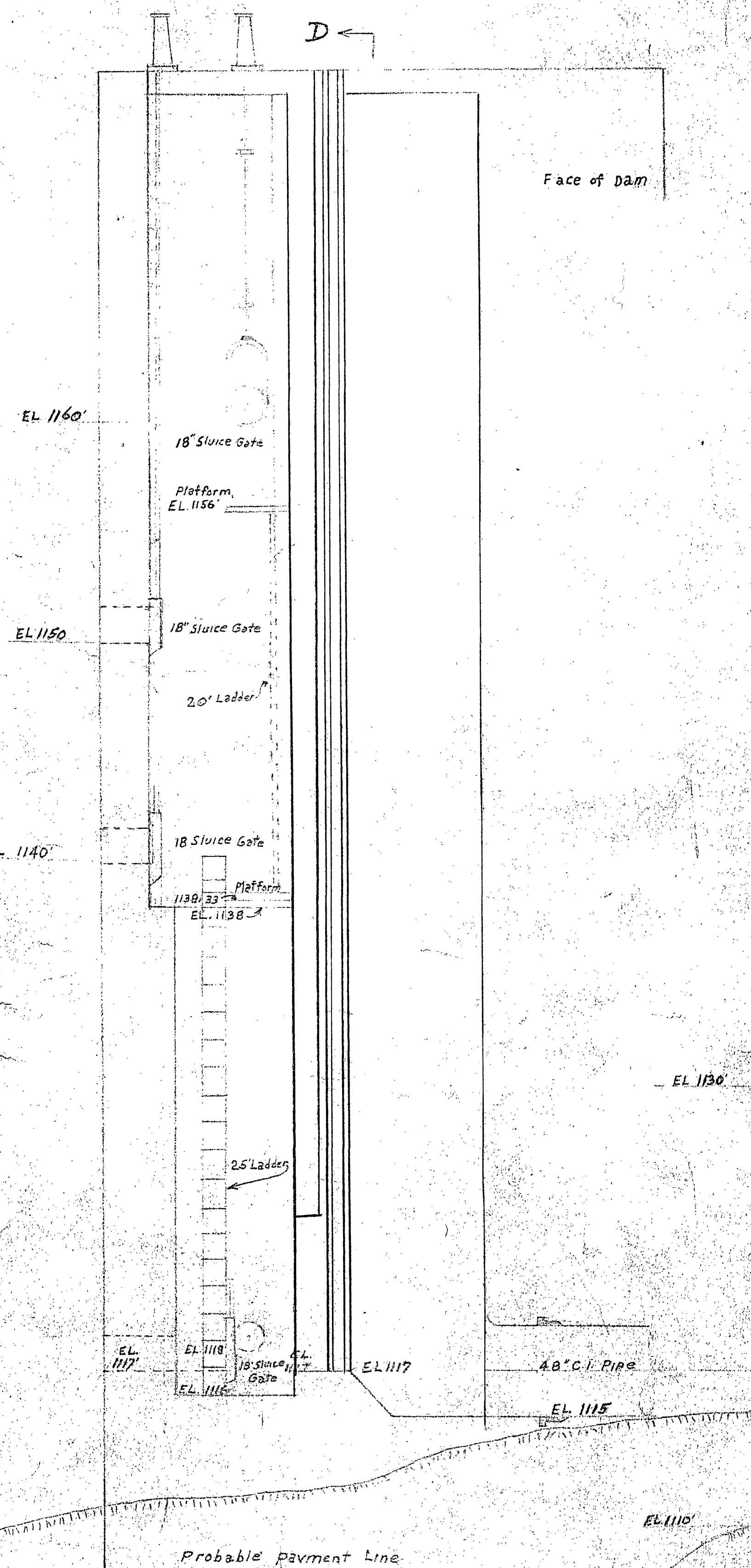
SECTION AA
