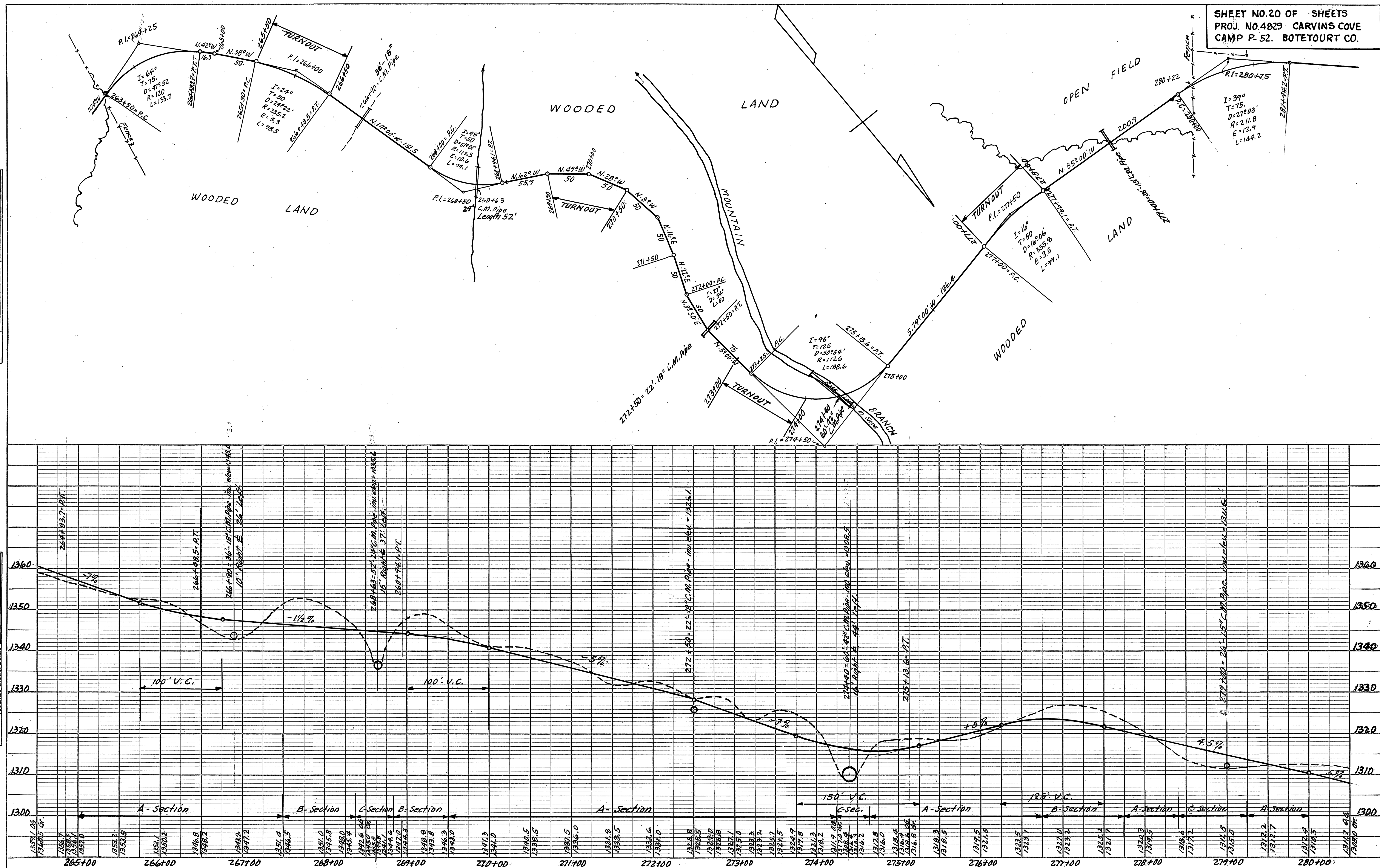
PLATE 1—PLAN PROFILE O. P. R. & R. E. STANDARD THE FREDERICK POST CO., CHICAGO
